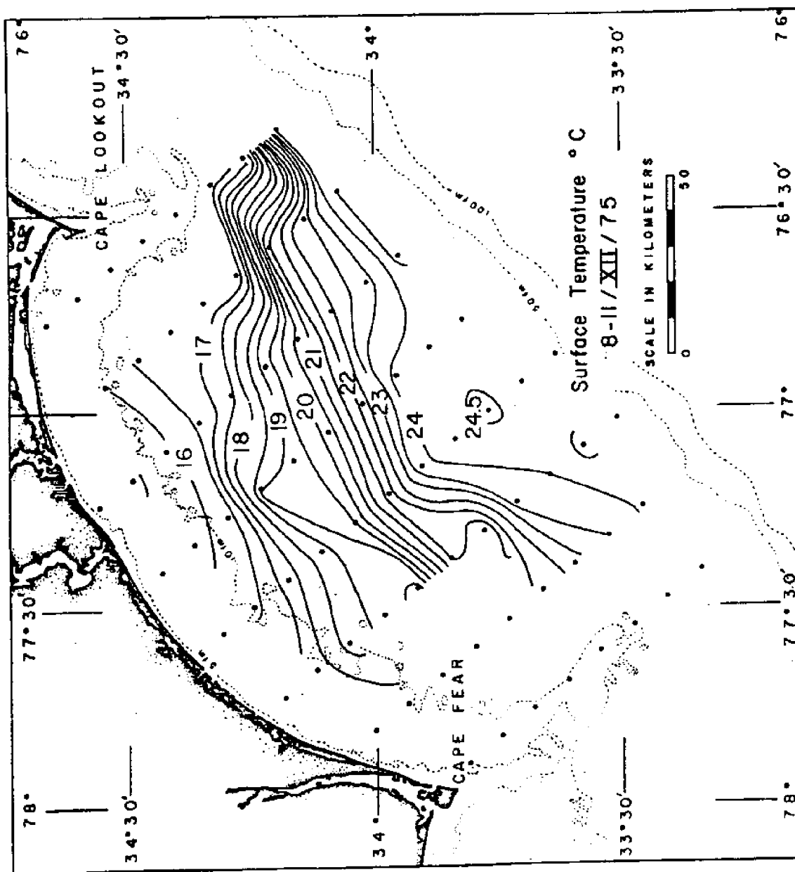
Figure 12. Surface temperature (8-11 December 1975)
