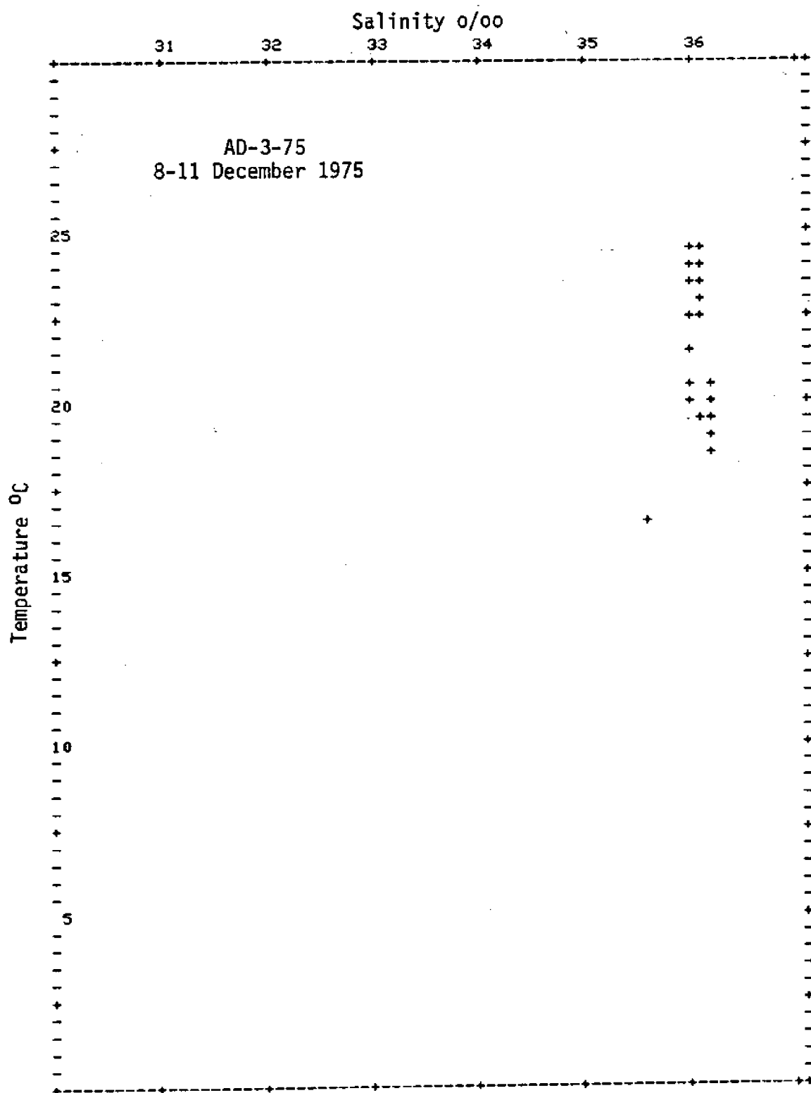
Figure 19. T-S Plot (OBIS IV: 8-11 December 1975)
