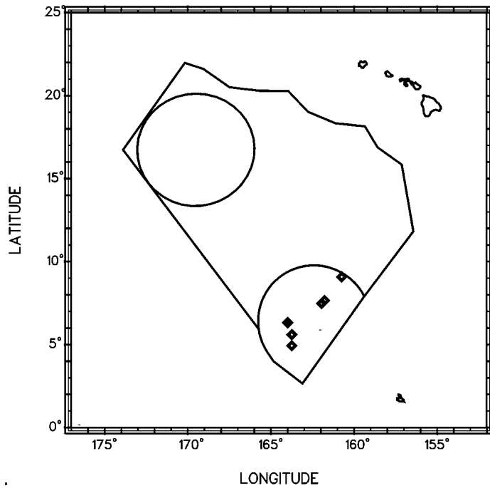
Figure 3. Location of acoustic detections of confirmed false killer whales (diamonds, n=6 ) that were missed by the visual line-transect survey. These confirmed detections were visually identified after they had passed abeam and had been obviously missed by the visual search team.
