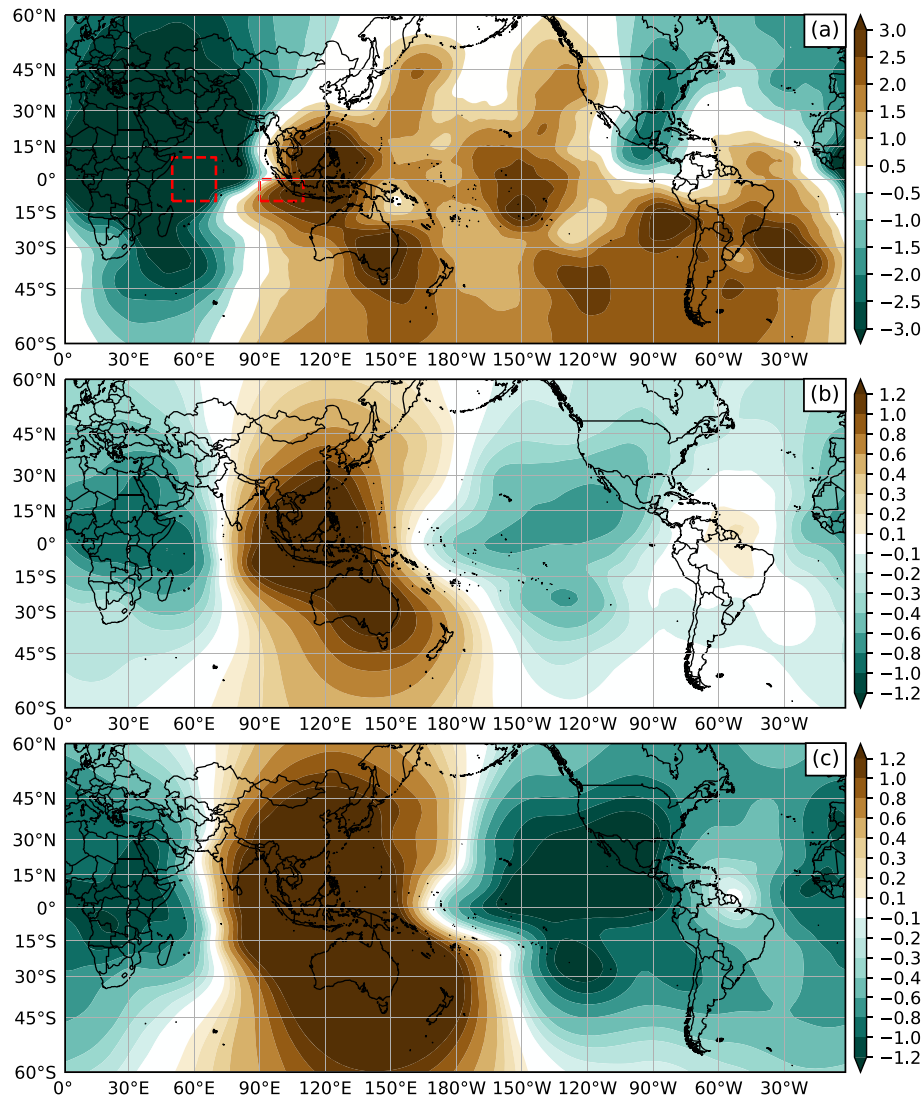
Figure 4. The 200-hPa velocity potential anomalies ( 10^6 \text{ m}^2 \text{ s}^{-1} ) relative to 1981–2010. (a) October 2019 from ERA5. Dashed red boxes indicate the western and eastern regions used to calculate the IOD index. (b) October 1960–2019 NCEP/NCAR Reanalysis anomalies regressed onto the October 1960–2019 COBE IOD index. (c) October 1960–2019 NCEP/NCAR Reanalysis anomalies regressed onto the October 1960–2019 NINO3.4 anomalies used to calculate the ONI.
