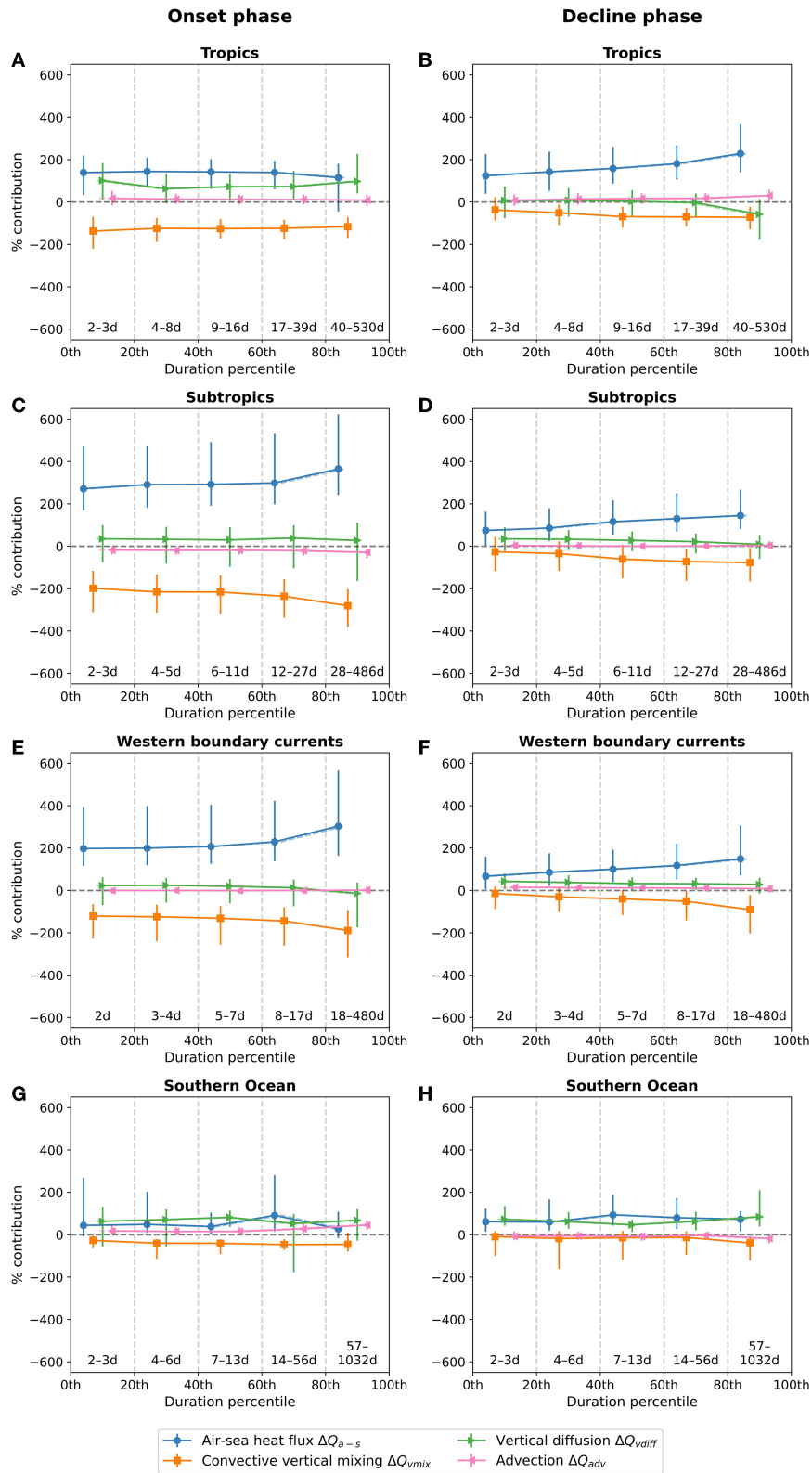
FIGURE 7 | The dependence of the marine heatwave drivers on the duration of marine heatwaves in four selected regions. The panels show the percentage contribution of marine heatwave drivers to the full temperature tendency during the onset and decline phases for different durations (start-to-end) of marine heatwaves in the tropics (A,B), subtropics (C,D), western boundary currents (E,F), and Southern Ocean (G,H). Each point gives the median percentage contribution of a driver to the total temperature anomaly during marine heatwaves with a duration within 10 percentage points of the duration percentile indicated on the x-axis. The vertical error bars show the interquartile range. For visual clarity, points within each duration bin are separated by a small horizontal distance. The regions are defined in Figure 8.
