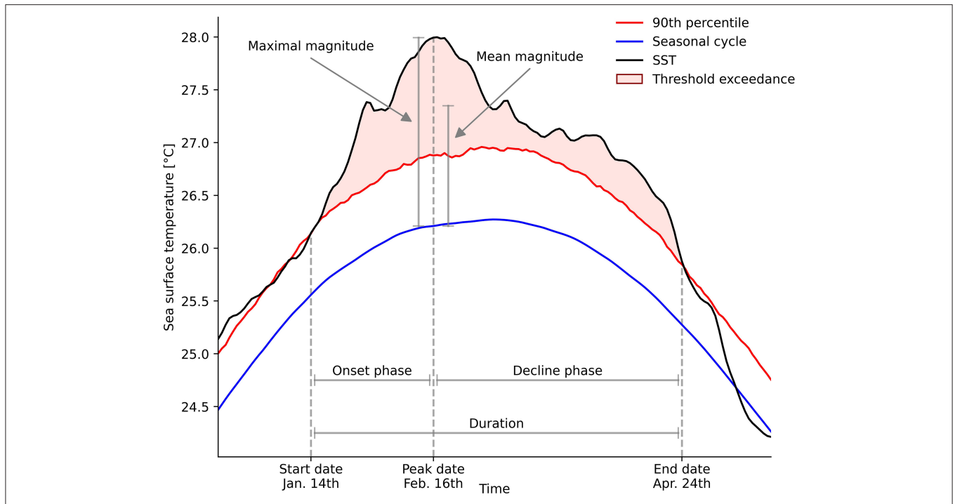
FIGURE 1 | Schematic figure illustrating the definition of a marine heatwave (MHW) and associated characteristics used in this study. The time series of simulated sea surface temperature (SST) averaged over the 55°E–105°E and 15°S–30°S region in the subtropical Indian Ocean for year 175 of the preindustrial control simulation is shown in black. The climatological seasonal cycle is shown in blue and the 90th percentile threshold in red. The red shaded area indicates the occurrence of the MHW. The period between the start (Jan 14th) and the peak (Feb 16th) of the MHW is labeled as the onset phase. The period between the peak and the end (Apr 24th) is labeled as the decline phase. The time span between start and end indicates the duration. Also shown are the maximum magnitude (maximal SST anomaly relative to the seasonal cycle) and the mean magnitude (SST anomaly averaged over the duration of the event).
