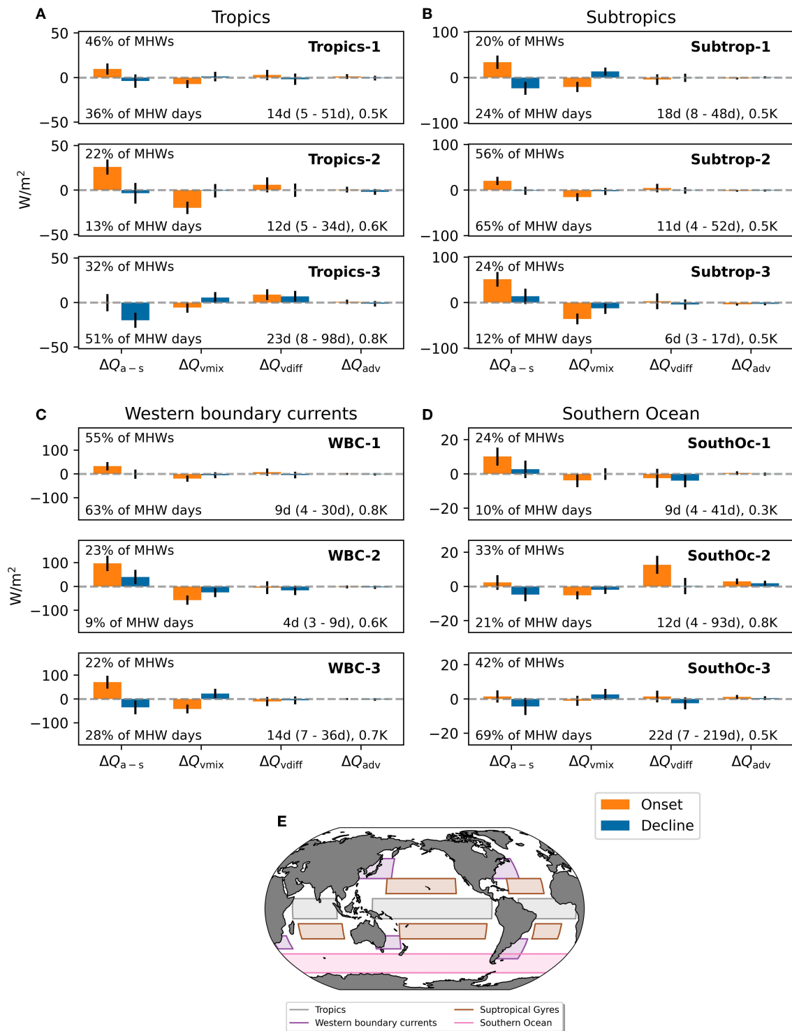
FIGURE 8 | (A–D) Marine heatwave types identified by K-Means clustering in four selected regions. Error bars show the standard deviation of each driver’s anomaly among marine heatwaves of each type. The median duration (in days), median maximal magnitude (in Kelvin) and the percentage of marine heatwaves and marine heatwave days occupied by marine heatwaves of each type are also given. Note the different y-axis scales used for different regions. The bottom panel (E) shows the definition of the regions. The definitions of the western boundary current regions are as in Hayashida et al. (2020), Figures 5, 6 therein.
