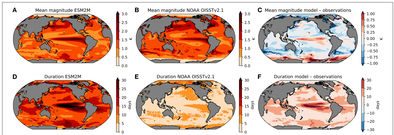
FIGURE 2 | Comparison between simulated and observed marine heatwave mean magnitude (top row) and duration (bottom row). The marine heatwave metrics are calculated from (A,D) the 500-yr preindustrial control simulation and (B,E) the NOAA OISST v2.1 dataset spanning the period from September 1st 1981 to December 24th 2020. The NOAA OISST v2.1 dataset is a blend of satellite and in situ ship, buoy, and Argo float sea surface temperature observations interpolated onto a global 1/4° resolution grid (Huang et al., 2020). (C,F) Differences between simulated and observation-based estimate. The NOAA OISST data was regridded onto the MOM4p1 grid after computing MHW metrics for comparison. Results for the GFDL ESM2M are similar when using a 1981–2021 reference period (not shown).
