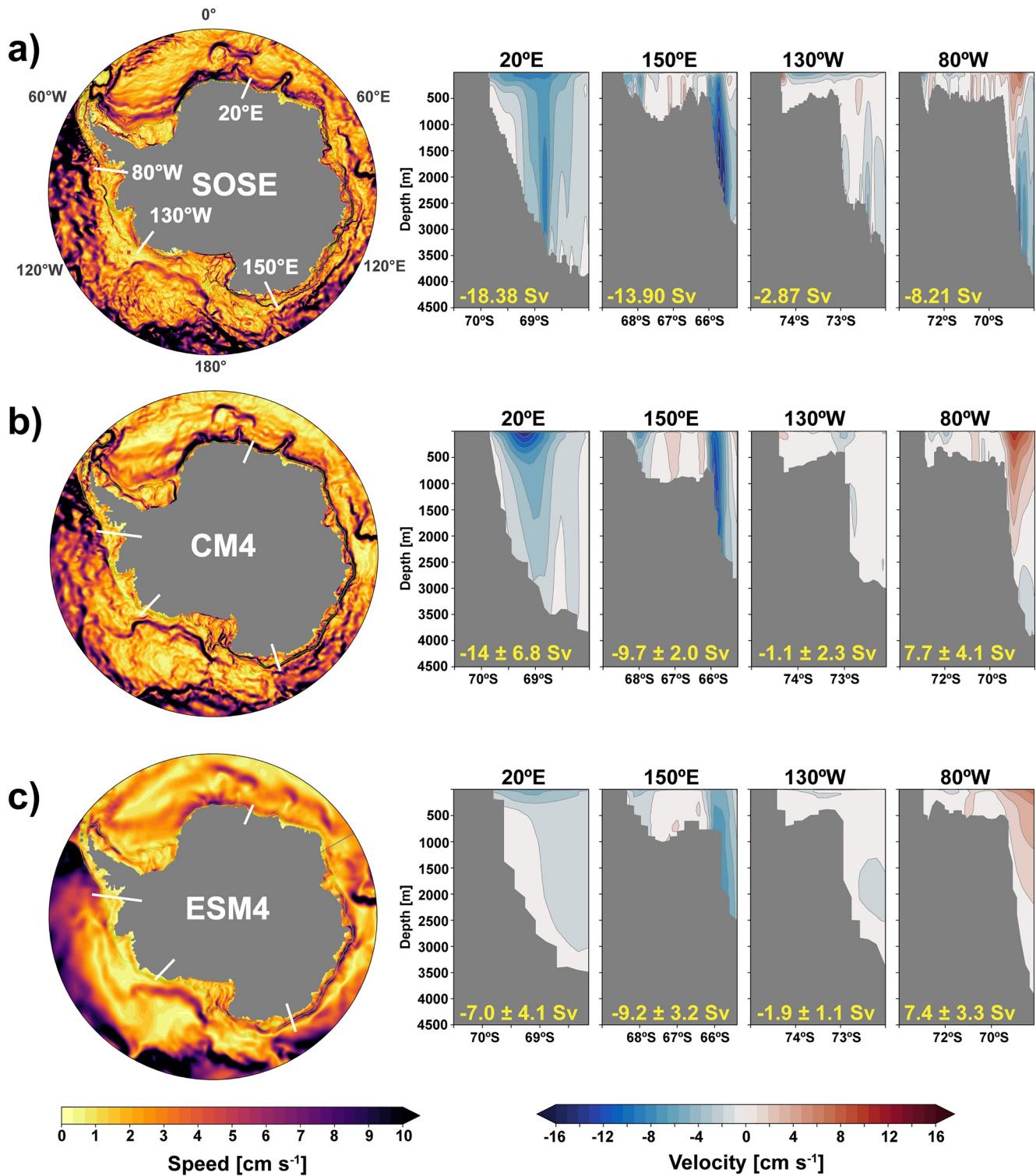
Figure 9. Speed ( \text{cm s}^{-1} ) depth-averaged over the upper 500 m and zonal velocity along the shelf and continental slope at four transects along the Antarctic coast (a) simulated in the 1/12° Southern Ocean State Estimate (SOSE) from 2006 to 2010 and (b)–(c) in the CM4 and ESM4 piControl simulations averaged over a 100-year period that overlaps with the perturbation experiments. The strength of the ASC is computed at four regions indicated by the white markers in each panel (20°E, 150°E, 130°W, 80°W). The mean strength for SOSE and the mean and interannual variability ( 1\sigma ) for the 100-year period of the piControl simulation are listed in yellow on the velocity panels. For both speed and velocity, negative transports and velocities indicate net westward flow. Positive transports and velocities indicate net eastward flow. The 1,000 m isobath is contoured in green.
