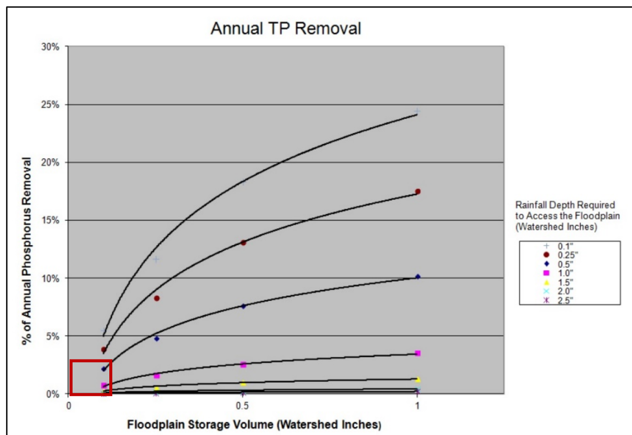
Figure 8. Protocol 3 annual TP removal.
