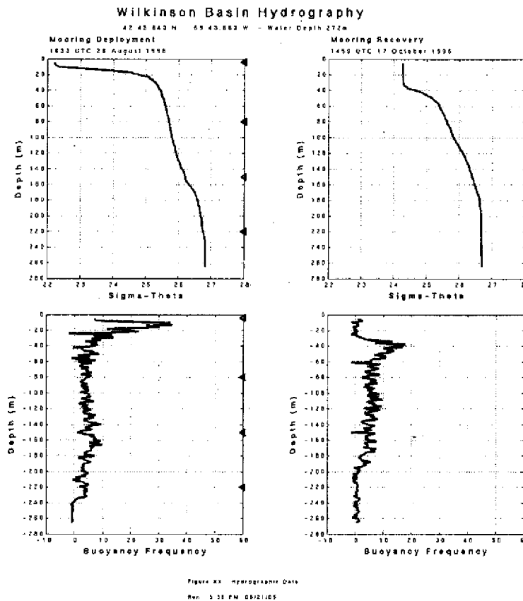
Figure 4 The sigma-theta and buoyancy frequency (cph) profiles derived from CTD measurements of water column properties (left) on 28 August 1996 at the mooring deployment and (right) on 17 October 1996 mooring recovery.
