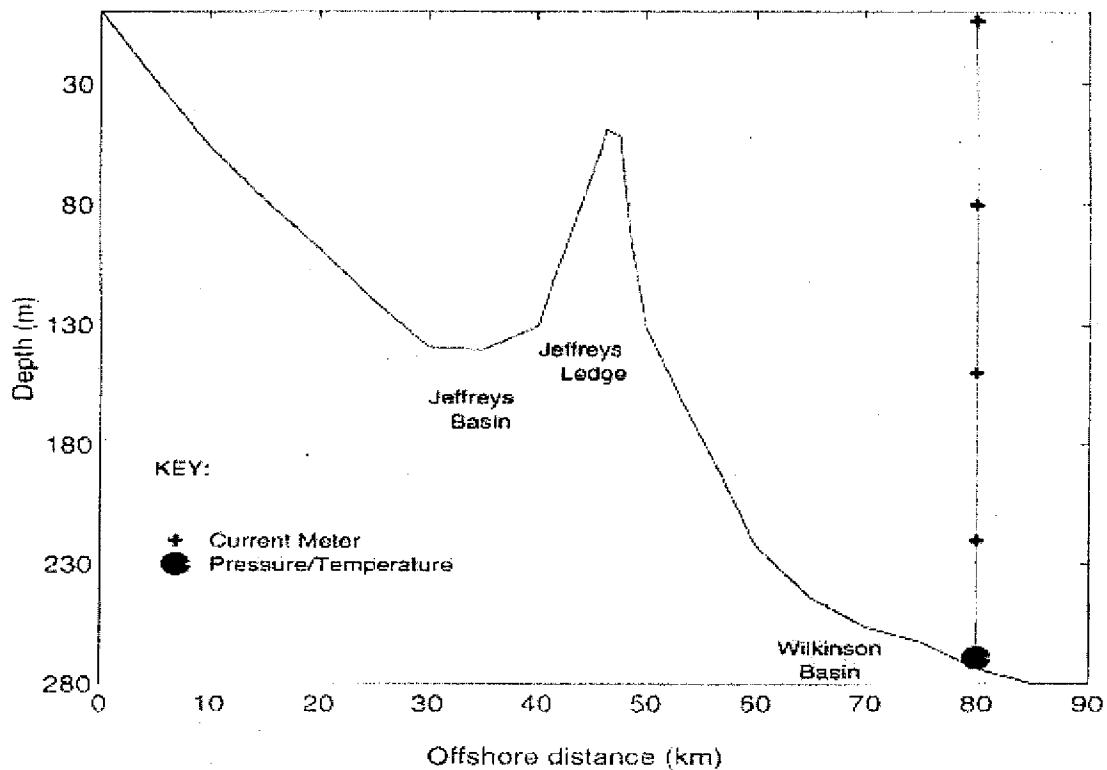
Figure 2 The bathymetry along a north-south transect from Cape Porpoise, ME on the left through Jeffreys Basin to northern Wilkinson Basin – marked by the location of the mooring on the right.
