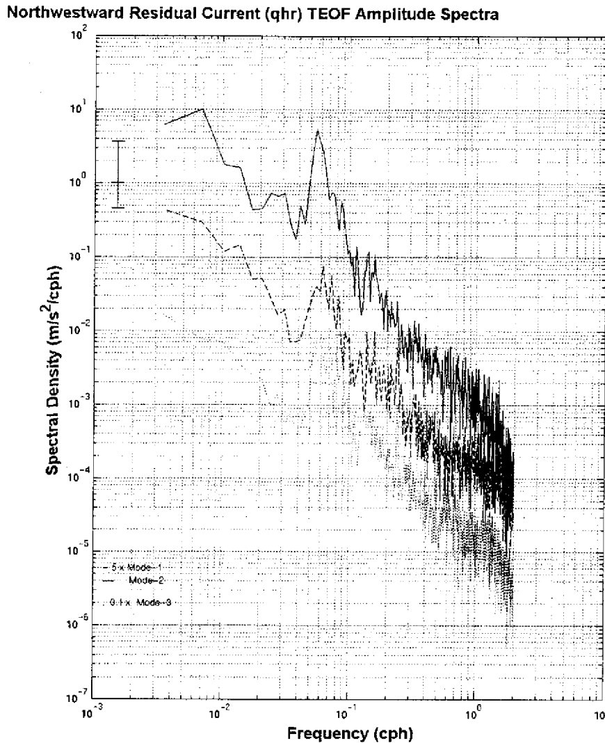
Figure 11 The spectral energy density functions of the three most energetic residual across-isobath current TEOF modes. Modes 1 (5x \text{---} ) and 3 (0.1x \text{-}\cdot\cdot\cdot\text{-} ) have been adjusted vertically relative to an unmodified mode 2 ( \text{-}\text{-}\text{-} ) for clarity. The 95% confidence intervals are indicated.
