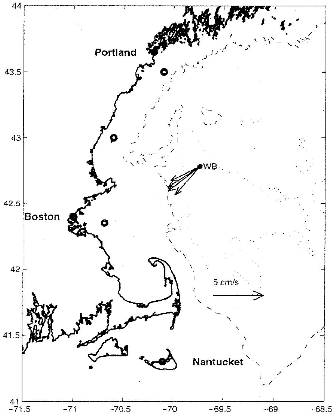
Figure 1 Location map of the August-October 1996 measurements in the Gulf of Maine (Boston and Portland NOS coastal sea level (solid circle); Boston, and Portland NDBC buoy meteorology (open circle); Wilkinson Basin moored currents and bottom pressure (cross). The series mean currents in Wilkinson Basin (WB) are shown.
