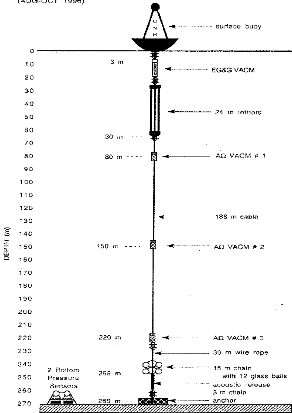
Figure 3 Schematic of the mooring deployed in Wilkinson Basin during Fall 1996.
