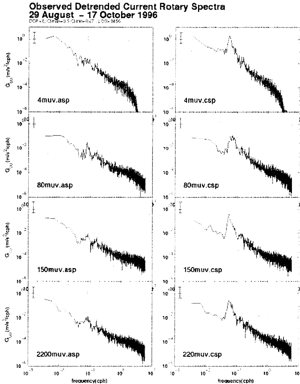
Figure 6 The clockwise (right) and anti-clockwise (left) rotary spectral energy density functions of the full (dotted) and residual (solid) 5-minute currents in Wilkinson Basin during Fall 1996. The more rapid roll-off
