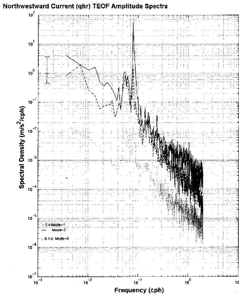
Figure 9 The spectral energy density functions of the three most energetic 15-minute across-isobath current TEOF modes. Modes 1 ( 5\times —) and 3 ( 0.1\times - - -) have been adjusted vertically relative to an unmodified mode 2 (—) for clarity. The 95% confidence intervals are indicated.
