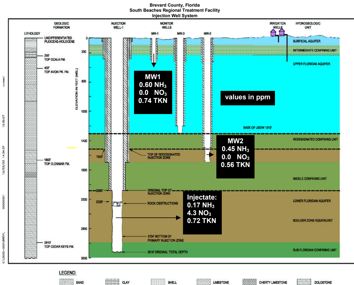
Figure 7. Diagram of the South Beaches Regional Treatment Facility injection and monitoring wells. Values (ppm) are averaged measured nutrient concentrations from January 2004 through January 2005. Data and diagram courtesy of Brevard County.
