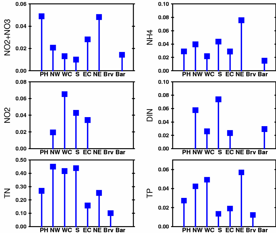
Figure 3. Nutrient concentrations (average, mg/L) reported by the FDEP for six Florida regions, for Brevard County alone (“Brv”), and by Barile (2004) (“Bar”). The Brevard data are also included within the EC region data set.
