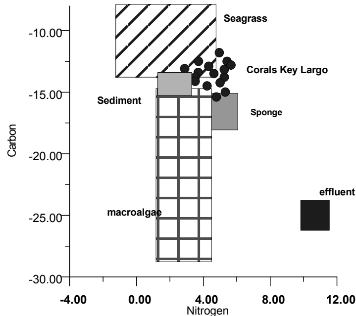
Figure 11. Ranges of C and N isotopic compositions measured in the study by Hoch et al. (2004). Additional coral data from Swart et al. (2005). Units are parts per thousand (‰).
