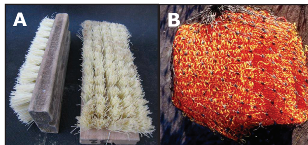
Figure 13. Artificial filamentous substrates used for monitoring young mussels and other invertebrates. A. Scrub brushes. B. Scrub pads (Tuffy®). Photographs by Carolyn Culver.
