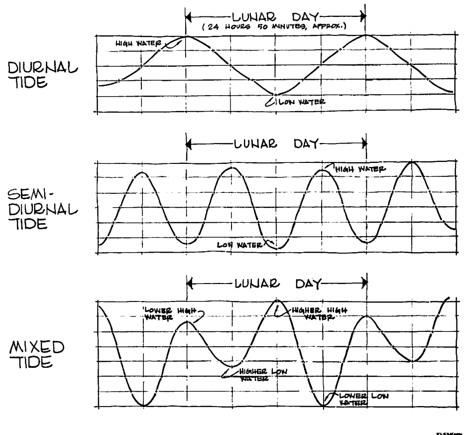
Figure 7.—Examples of marigram types.
