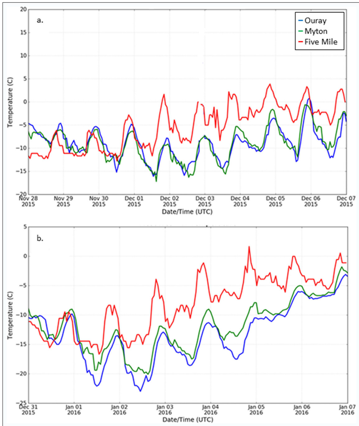
Figure 3: Time series of 2-m air temperature at supplementary stations. Time series of 2-m air temperature from Mesowest at station Ouray (blue line, elevation 1411 m), station Myton (green line, elevation 1411 m) and station Five Mile (red line, elevation 2280 m) for (a) 28 November – 6 December 2015. (b) 31 December 2015–6 January 2016. DOI: https://doi.org/10.1525/elementa.362.f3
