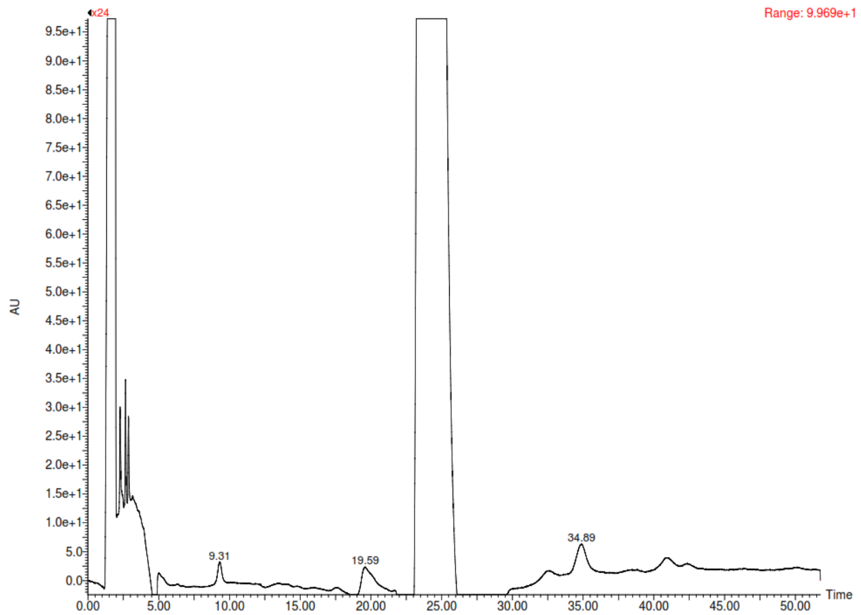
Figure 8: Chromatogram of Dye 8
