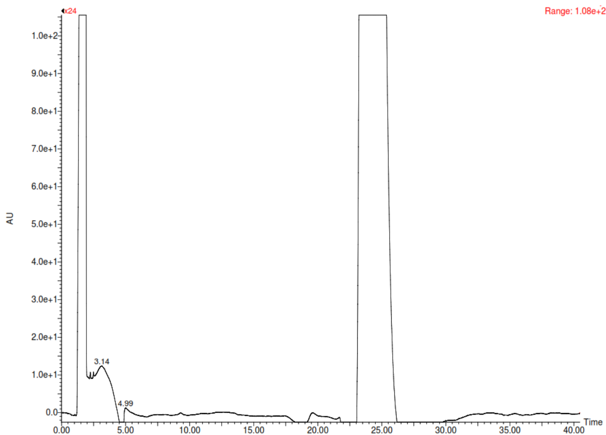
755 Figure 1: Chromatogram of Dye 1.
