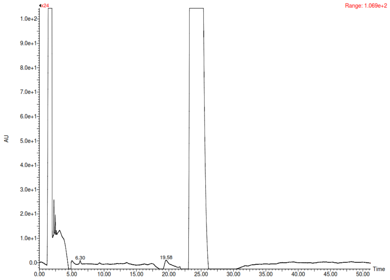
766 767 Figure 5: Chromatogram of Dye 5 768
