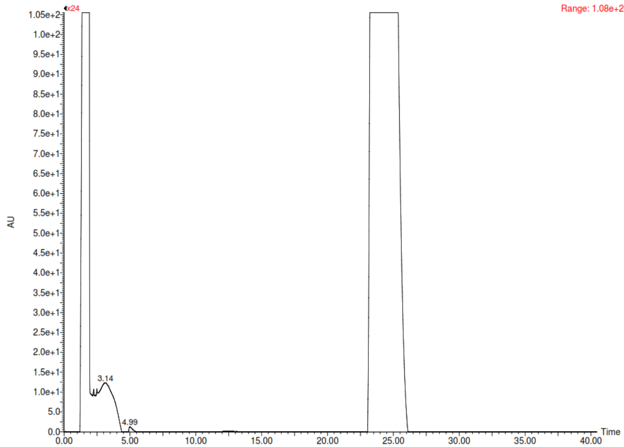
758 Figure 2: Chromatogram of Dye 2
