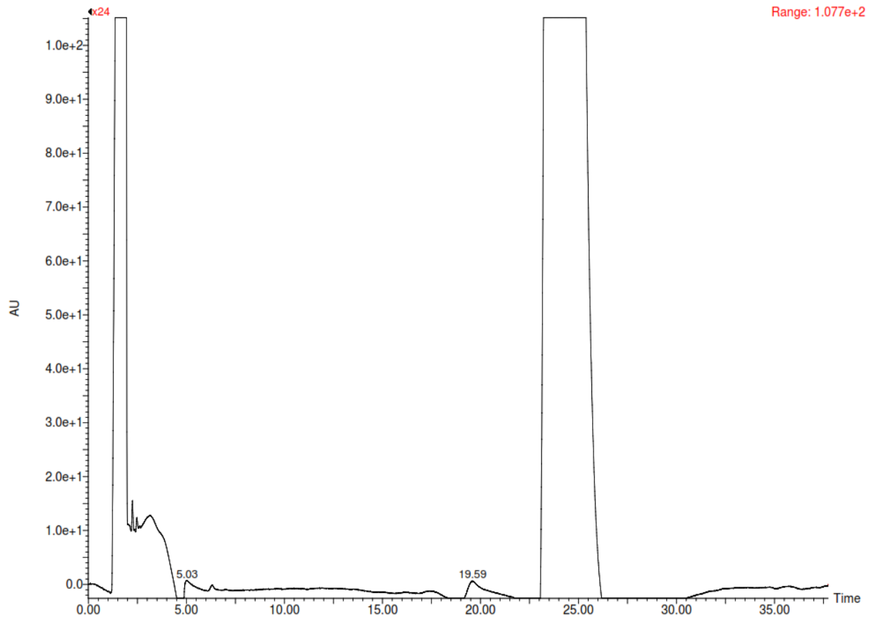
Figure 6: Chromatogram of Dye 6
