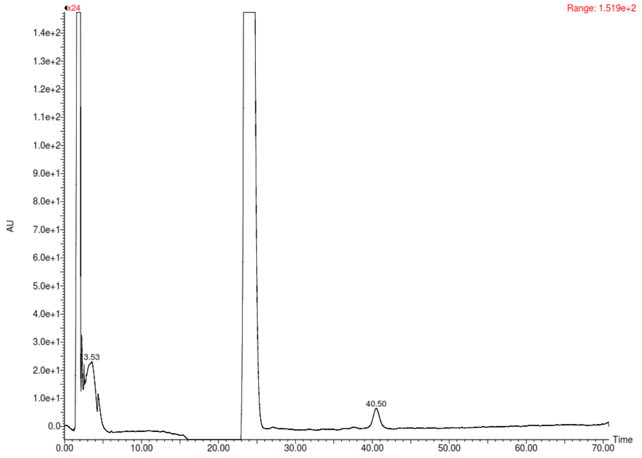
776 Figure 9: Chromatogram of Dye 9
