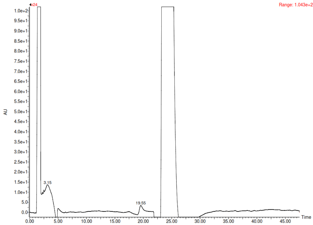
Figure 4: Chromatogram of Dye 4
