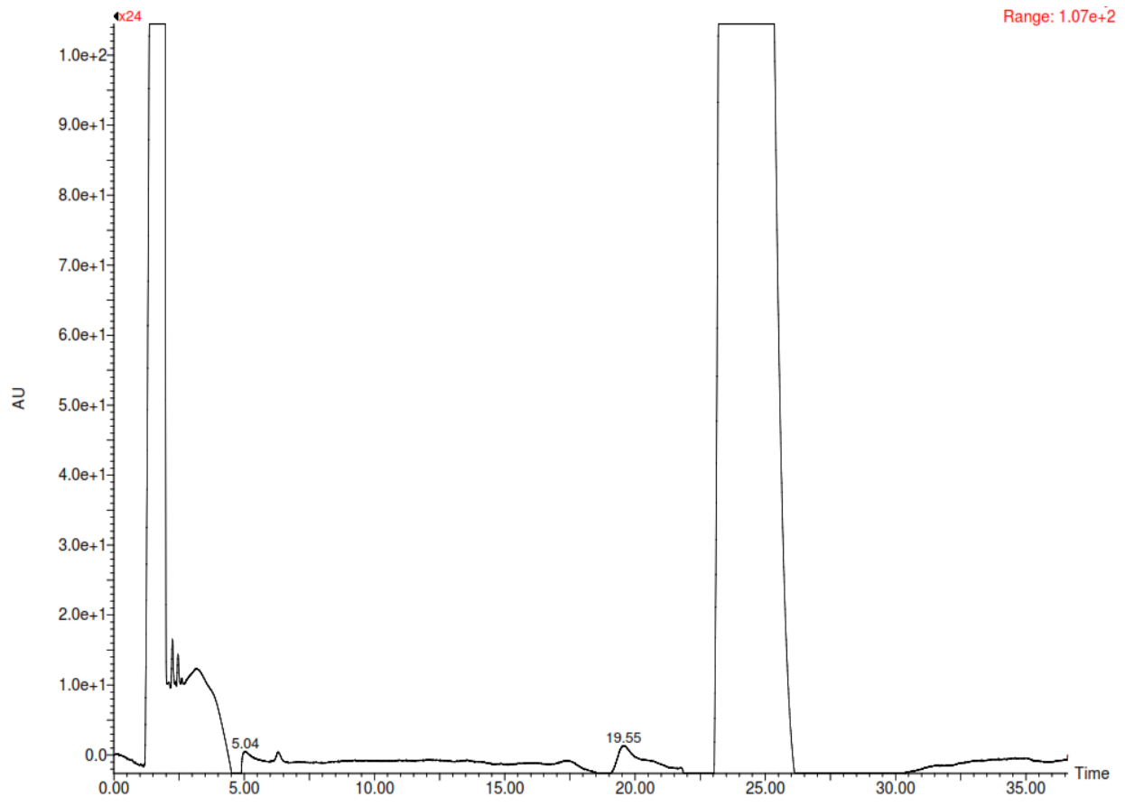
761 Figure 3: Chromatogram of Dye 3
