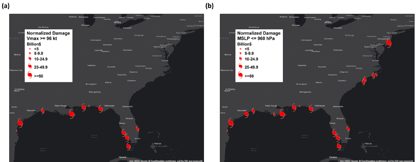
Fig. 3. Landfall location of CONUS major hurricane landfalls from 1999 to 2018 using the (a) V_{max} definition ( \geq 96 kt) and the (b) MSLP definition ( \leq 960 hPa). Larger hurricane symbols represent more normalized hurricane damage.
