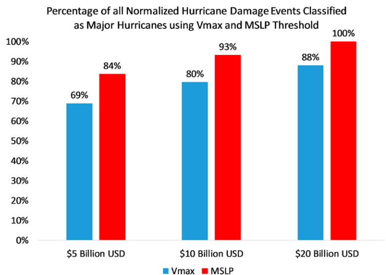
Fig. 5. Percentage of landfalling hurricanes where the major hurricane threshold was met using the V_{max} and MSLP definitions when normalized damage exceeded $5 billion, $10 billion, and $20 billion, respectively.
