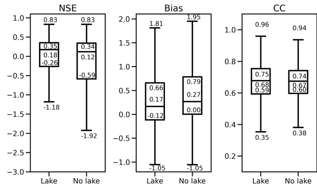
Figure 5. Boxplot of model performance comparing results with lake routing and without lake routing.
