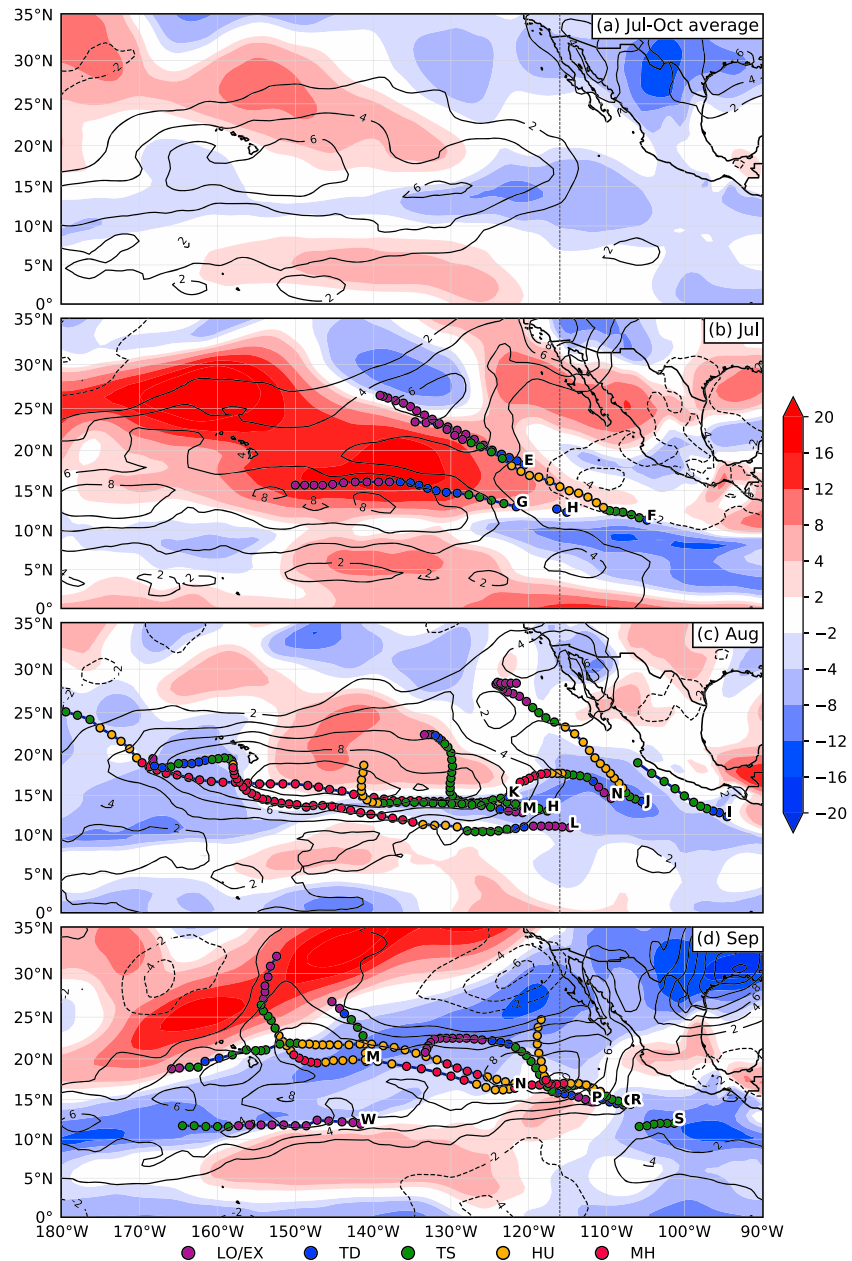
Figure 3. Anomalies (relative to 1998–2017) of 200–850-hPa vertical wind shear (kt; shaded) and total precipitable water ( \text{kg}/\text{m}^2 ; contours) during (a) July–October 2018 and in (b) July 2018, (c) August 2018, and (d) September 2018, individually. Dots in panels (b)–(d) indicate 6-hourly tropical cyclone locations and intensities during each month. Letters denote the first storm location in the given month.
