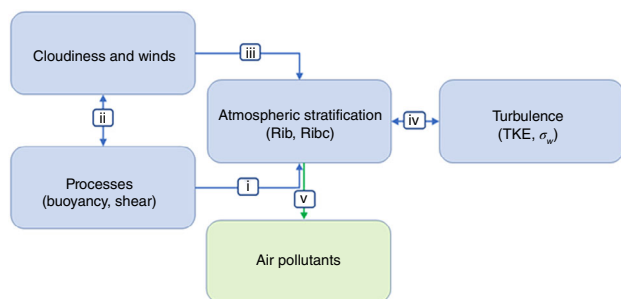
FIGURE 2 Schematic view of the research items outlined in Section 1. (1) Atmospheric state and impact of buoyant suppression and shear generation of turbulence on atmospheric stratification, (2) relation between cloudiness and winds and stratification-related processes, (3) impact of cloudiness and winds on atmospheric stratification, (4) connection between observed turbulence and Rib, and (5) influence of atmospheric stratification on air pollutants
