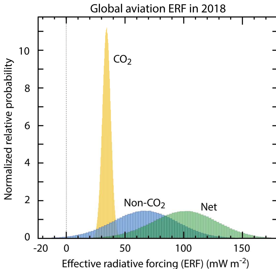
Figure 7. Probability distribution functions (PDFs) for aviation ERFs in 2018 based on the results in Figure 3 and Table 2 . PDFs are shown for separately for CO 2 , the sum of non-CO 2 terms, and the net aviation ERF. Since the area of each distribution is normalized to the same value, relative probabilities can be intercompared. Uncertainties are expressed by a distribution about the best-estimate value that is normal for CO 2 and contrail cirrus, and lognormal for all other components. A one-million-point Monte Carlo simulation run was used to calculate all PDFs.
