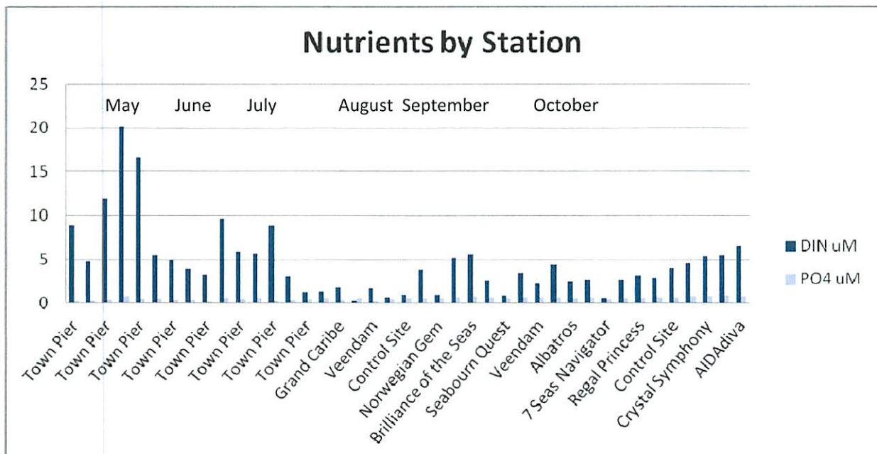
Figure 3. Dissolved Inorganic Nitrogen (DIN) and phosphorus levels over the sampling time period.
