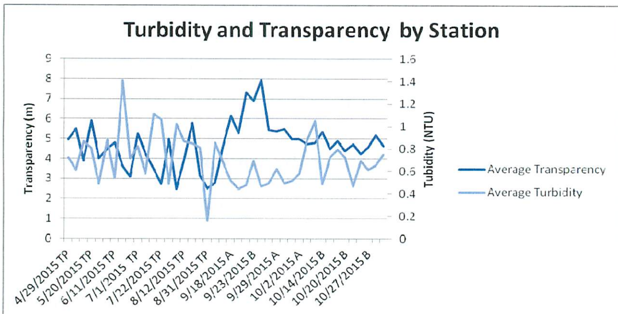
Figure 4. Transparency and turbidity are inversely related at all stations through the 2015 cruise season.
