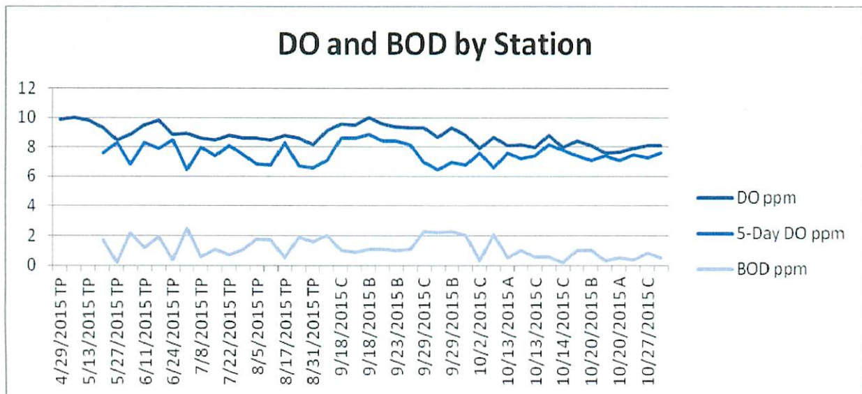
Figure 2. Dissolved oxygen (DO), DO after a five-day hold (5-Day DO), and biochemical oxygen demand (BOD) over the sampling time period.
