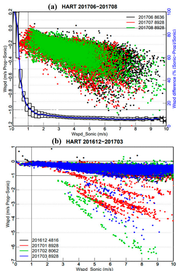
FIG. 3. Wind speed differences (propeller – sonic; in \text{m s}^{-1} ) as a function of sonic wind speed (in \text{m s}^{-1} ) (a) from June to August 2017 and (b) from December 2016 to March 2017 at Hartsville (HART) site. Different colors represent different months. The numbers in the legend represent total number of data points. Note that the scale for the y axis for the top and bottom panels is different. The boxplot in (a) is the relative wind speed difference [(sonic – propeller)/sonic] in % using right y axis for all 3 months.
