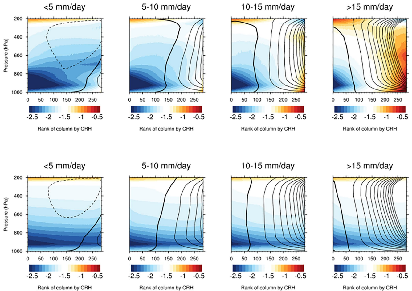
Figure 9. Composites of CRH-sorted stream function (contours; the thicker solid line shows zero values) and radiative cooling rates (colors; \text{K day}^{-1} ) for the Control run (top) and the ClimRad run (bottom) for different domain average precipitation bins.
