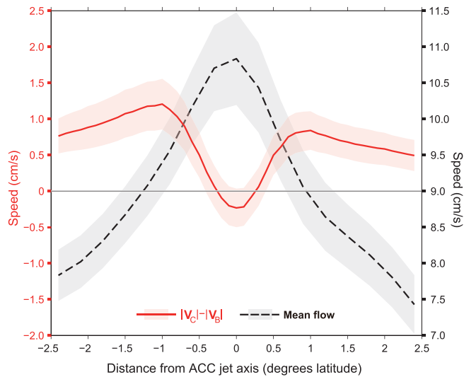
Figure 6. Along-ACC averaged speed changes (calculated from |V_C| minus |V_B| ) as shown in Figure 3a) for floats released in the ACC region (see text for details), plotted as a function of distance from the ACC core. Here the core is defined by the latitude of the maximum zonal velocity. The red line indicates the median acceleration, and the red shading indicates uncertainties representing the 95% confidence intervals computed from the standard error of the mean, using 1,000 realizations of a bootstrapping procedure. The dashed overlaid black line and the gray shading indicate the mean speeds and the associated uncertainties in this same coordinate system.
