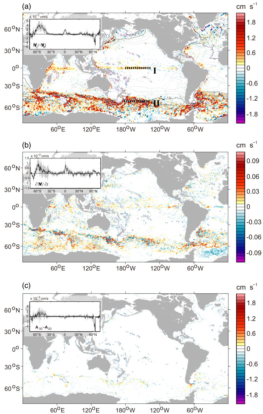
Figure 3. (a) Speed differences between Point B and Point C calculated as |V_C| minus |V_B| . Sections I ( 178\text{--}132^\circ\text{W} , 0^\circ\text{S} ) and II ( 178\text{--}132^\circ\text{W} , 52^\circ\text{S} ) used in Figure 5 are indicated with black dotted lines. (b) Eulerian speed change at fixed Position B, calculated as |V_{B|t_C}| - |V_{B|t_B}| . B denotes the location of parking start (shown in Figure 1), t_B is the parking start time, and t_C is the parking end time. (c) Acceleration obtained with advection by three-dimensional velocity minus acceleration from (a) advecting only with horizontal velocity components. The contours in panel a are the mean pressure isobars at intervals 1,000 \text{ N m}^{-2} to indicate the ACC. Three representative isobars ( -5,000 , 0 , 5,000 ) are indicated in bold. Insets in all panels show the zonal average values.
