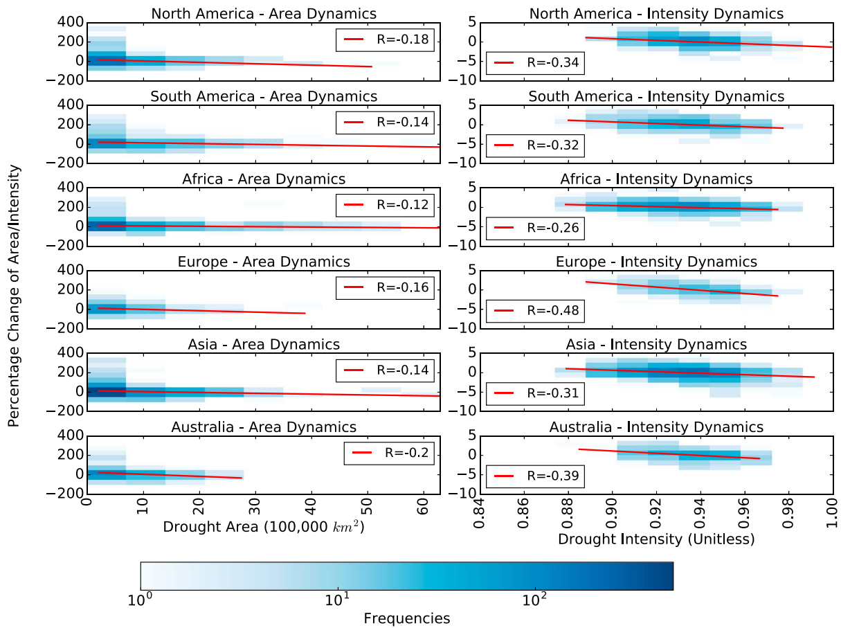
Figure 3. Regional 2-D histograms of rates of change in (left column) area and (right column) intensity as a function of area and intensity, respectively, during the previous month. Red line displays linear regression results. All correlations yielded p < 0.05 .
