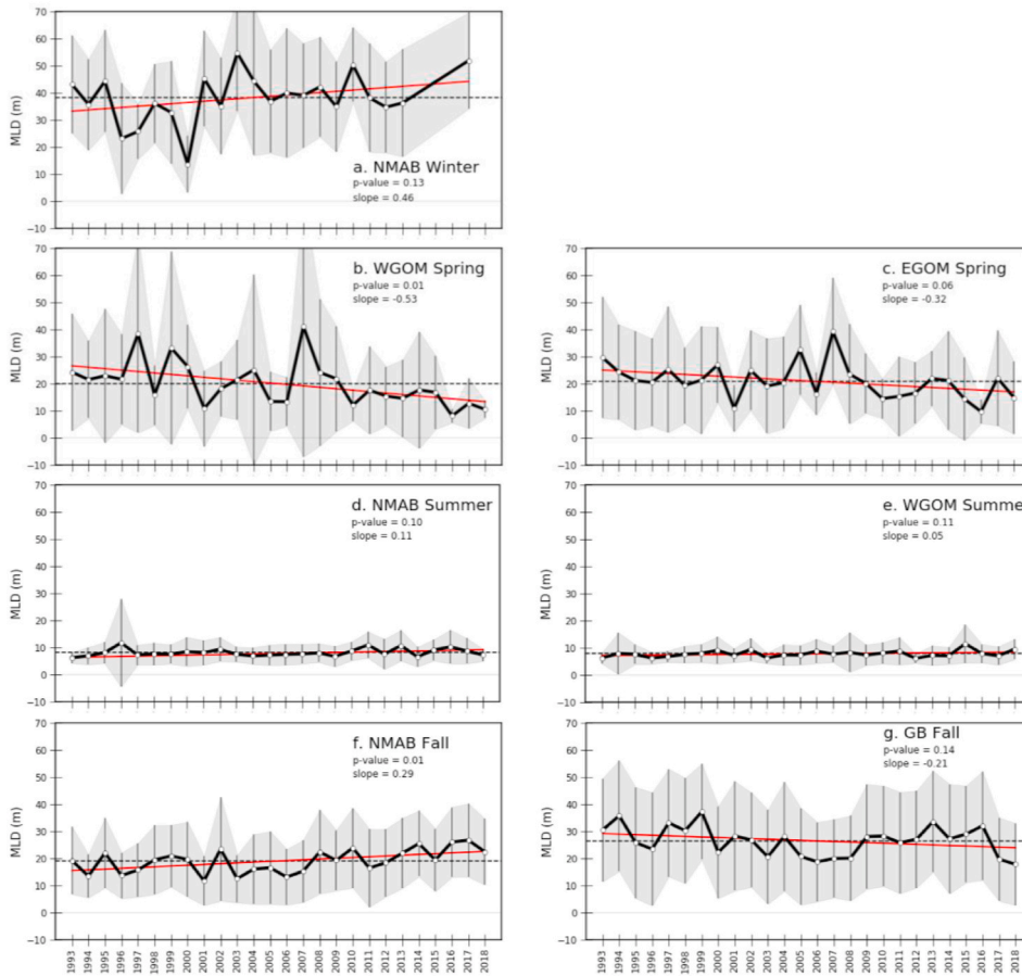
Fig. 16. MLD timeseries from 1993 to 2018 shown for eco-regions (a) NMAB winter, (b) WGOM spring, (c) EGOM spring, (d) NMAB summer, (e) WGOM summer, (f) NMAB fall, and (g) GB fall with trends that are statistically significant (i.e., p \leq 0.15 ). The linear trend is illustrated using a red solid line while the long-term average is shown using a black dashed line. The value of long-term linear trend (m/year) is indicated in each panel along with corresponding p-value. 1 STD is shown using shading.
