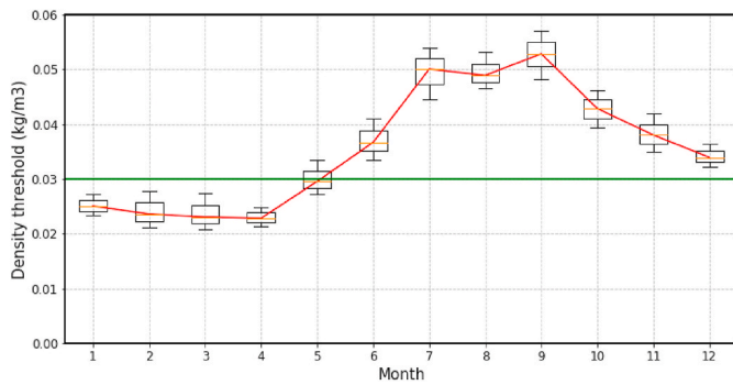
Fig. 3. Boxplot showing the climatological distribution of density threshold used in GLORYS12V1 by month corresponding to a 0.2\text{ }^{\circ}\text{C} temperature decrease from the reference temperature value at 10 m. The green line specifies the 0.03\text{ kg/m}^3 density threshold. The average of the median density thresholds by month used in GLORYS12V1 is 0.036\text{ kg/m}^3 .
