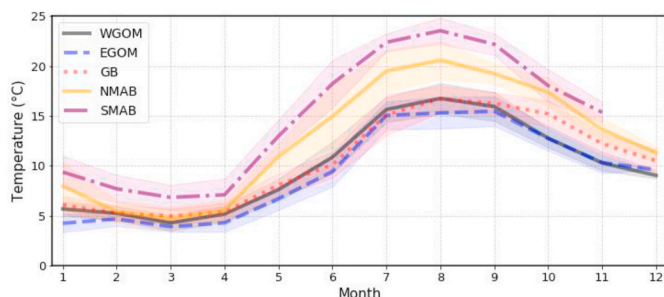
Fig. 9. Mixed layer temperature (MLT) climatological seasonal cycle from in situ observations using density threshold-based MLD with the 1 standard deviation (STD) ranges shaded, for each eco-region. The regional mean MLTs are calculated first for each month/year, and monthly means and STDs are calculated subsequently so that the shading primarily reflects interannual variations.
