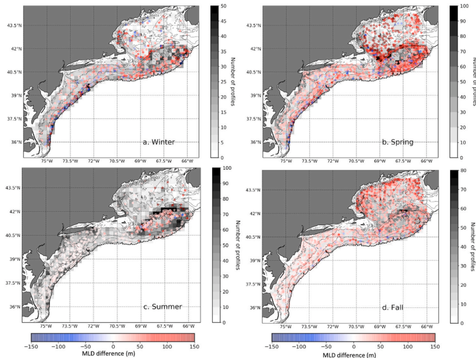
Fig. 15. Locations where the difference between the two methods (temperature-based MLD minus density-based MLD) is greater than 1 standard deviations from zero difference, shown for each season: (a) winter, (b) spring, (c) summer, and (d) fall. The magnitude of differences are shown by the colored dots, while the gray shading indicates data availability for each 0.25^\circ \times 0.25^\circ bin.
