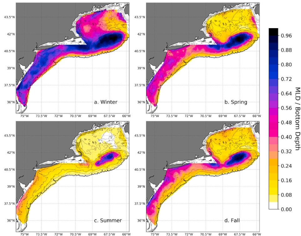
Fig. 8. As in Fig. 7 but showing the mean MLD ratio to bottom depth for each season.
