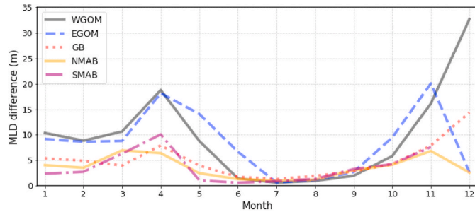
Fig. 14. Spatially averaged and climatological MLD difference (temperature-based MLDs minus density-based MLDs) for the 5 eco-regions in each month. The MLD differences are calculated from regional mean MLDs which are calculated first for each month/year. Note that there are only 247 profiles from 4 years (1993, 1994, 2010, and 2011) in December.
