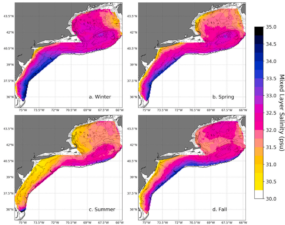
Fig. 12. As in Fig. 7, but for the MLS.
