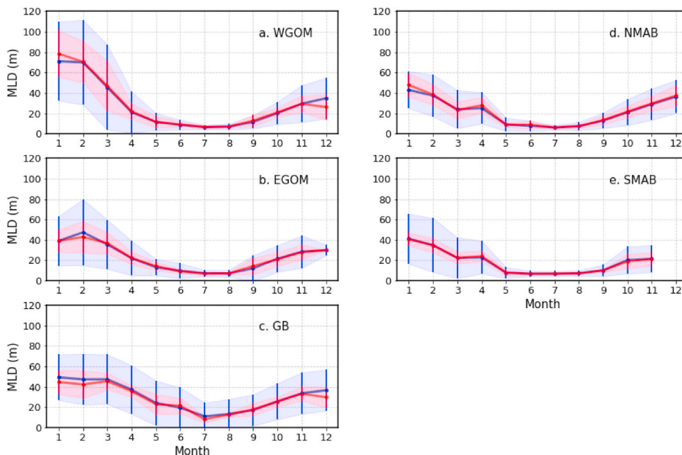
Fig. 6. MLD climatological seasonal cycle from in situ observations using density threshold with the 1 standard deviation (STD) ranges shaded, for each eco-region: (a) WGOM, (b) EGOM, (c) GB, (d) NMAB, and (e) SMAB. For the red curves and shading, the regional mean MLDs are calculated first for each month/year, and monthly means and STDs are calculated subsequently so that the red shading primarily reflects interannual variations. The blue curves and shading are calculated using all data in the region and month at once, therefore also including the variability introduced by variations in the spatial data coverage from year to year. In SMAB, there is no data for December during the study period.
