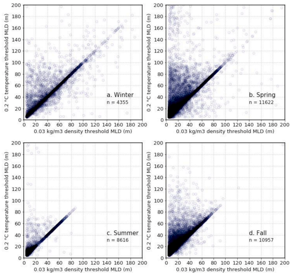
Fig. 13. Comparison of observed MLDs from the density method (threshold: 0.03 \text{ kg/m}^3 ) against MLDs from the temperature method (threshold: 0.2 \text{ }^\circ\text{C} ) for the entire NEUS continental shelf in each season: (a) winter, (b) spring, (c) summer, and (d) fall.
