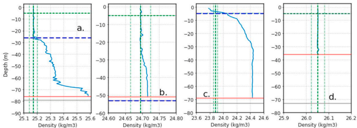
Fig. 4. Examples of the four MLD categories based on the density-threshold MLD detection scheme: (a) a well-defined mixed layer within the profile (61.5% of all profiles), (b) a fully mixed profile (16.4%), (c) a fully stratified profile (16.4%), and (d) an inconclusive profile (5.7%). The red line specifies the depth of the deepest observational measurement. The gray line shows the sea floor depth. The dark blue dashed line indicates the detected MLD. The dark green dashed vertical and horizontal lines show the surface layer density value and the 5-m depth mark, respectively. The light green dashed vertical lines designate the density threshold, i.e., 0.03\text{ kg/m}^3 , from the surface layer density value. In (b), the sea floor depth is considered as the MLD.
