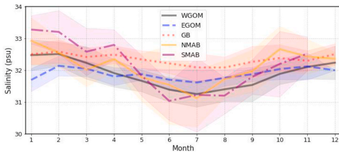
Fig. 11. As in Fig. 9, but for the mixed layer salinity (MLS).
