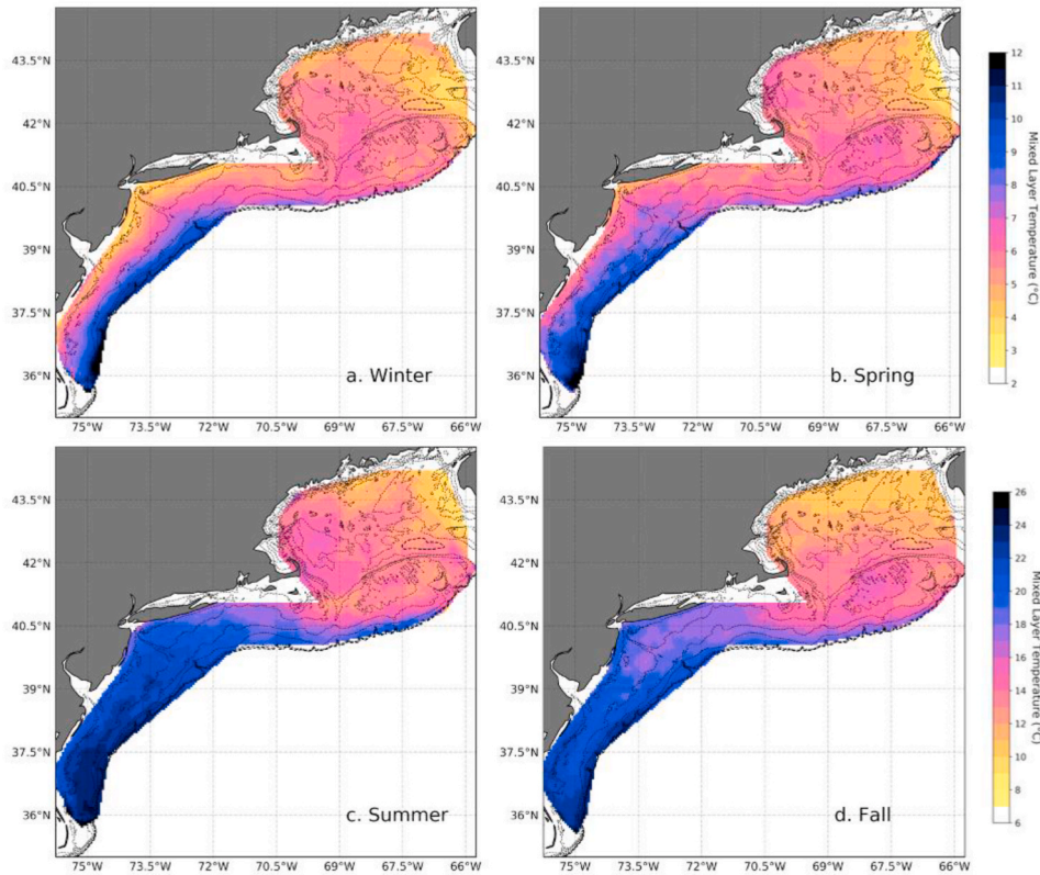
Fig. 10. As in Fig. 7, but for the MLT. Note that the (a–b) and (c–d) use different color ranges.
