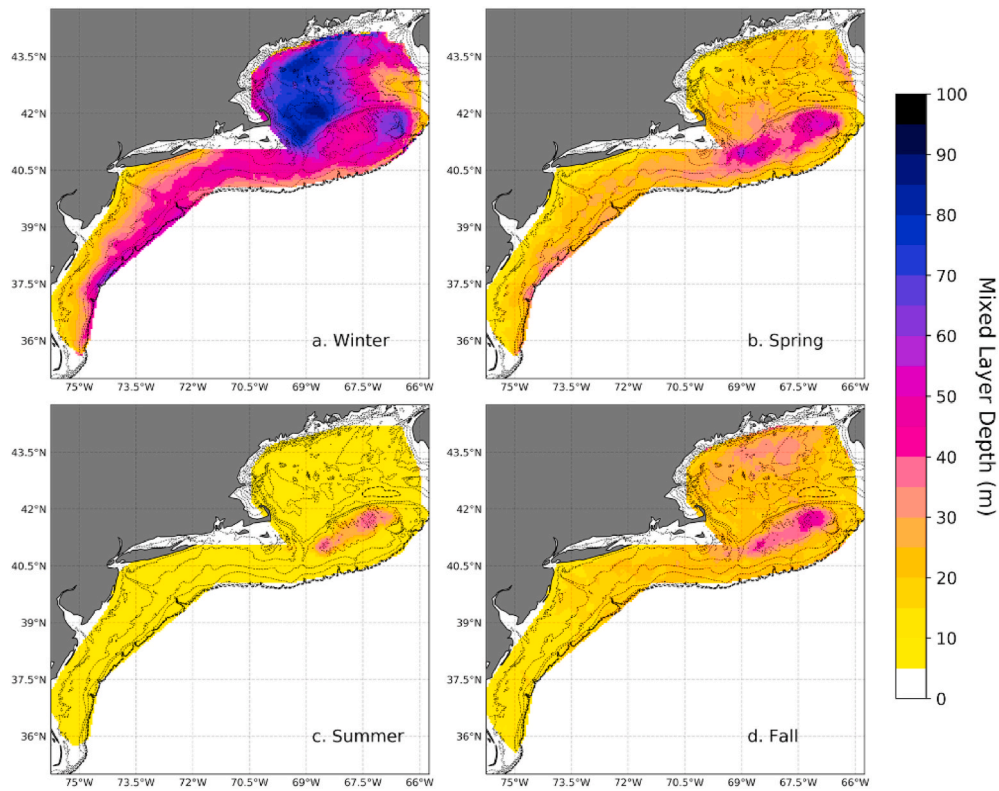
Fig. 7. Spatial patterns of mean MLDs from observations using the density threshold for each season at 0.05-degree resolution: (a) winter (December–February), (b) spring (March–May), (c) summer (June–August), and (d) fall (September–November). Bathymetry contours at 25, 50, 75, 100, 200, and 300 m are shown using black dashed lines, and the 300-m contour is thickened.
