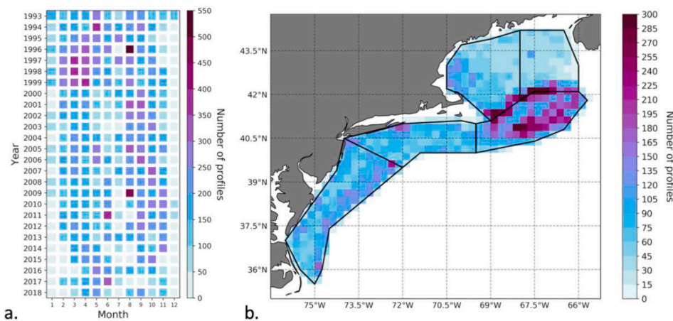
Fig. 2. Temporal and Spatial coverage of the observational profiles from NEFSC. (a) Monthly data coverage from 1993 to 2018 on the NEUS continental shelf from the NEFSC hydrographic dataset and (b) spatial distribution of number of profiles within each 0.25^\circ \times 0.25^\circ bin (horizontal resolution) from 1993 to 2018 of all seasons compiled together. The black lines indicate the boundaries for the 5 eco-regions shown in Fig. 1.
