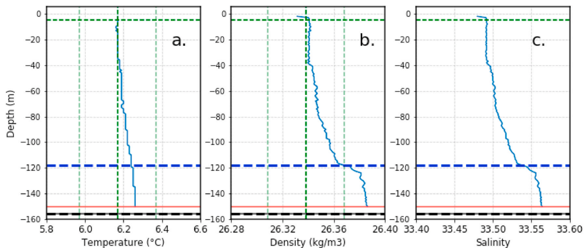
Fig. 5. An example of (a) temperature, (b) density, and (c) salinity profiles where the temperature-based MLD differs from the density-based MLD. This profile was collected at 41.46°N, 69.17°W near the Great South Channel, 2003-01-30. The profile is fully mixed based on the temperature-based detection. The black dashed line shows the temperature-based MLD at 156 m, which is also the sea floor depth, while the blue dashed line shows the density-based MLD at 118 m. In order for the density threshold method to detect the MLD at the bottom (as in the temperature-based case), the density threshold would need to be increased to 0.05 kg/m 3 .
