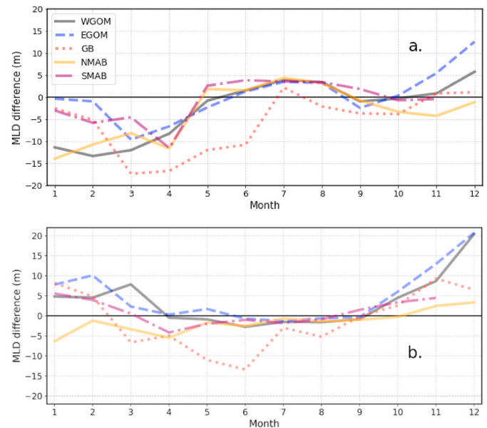
Fig. 17. Spatially averaged and climatological MLD difference of (a) GMLD minus observational density based MLDs and (b) GMLD03 minus observational density-based MLDs for the 5 eco-regions.
