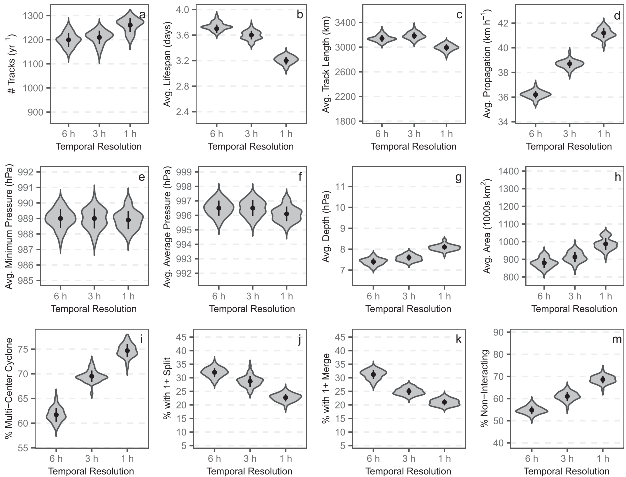
FIG. 9. As in Fig. 5, but with a dynamic maximum propagation speed of 125, 192, and 300 km h -1 for 6-, 3-, and 1-h resolutions, respectively. (b)–(d),(g)–(m) All means are significantly different ( p < 0.05 ). In other panels, no significant difference exists (e) between any mean or (a),(f) between 6 and 3 h.
