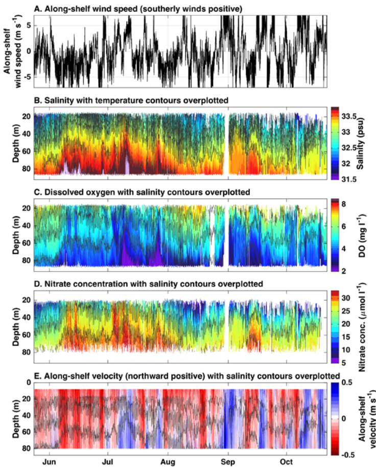
Figure 8. 2015 conditions at the NANOOS coastal mooring site: (A) along shore winds, with southerly winds positive (to north) and northerly winds negative (to south), (B) salinity with temperature contours over-plotted, (C) dissolved oxygen with salinity contours over-plotted, (D) nitrate concentration with salinity contours over-plotted, (E) along-shore velocity (positive to north) with salinity contours over-plotted.
