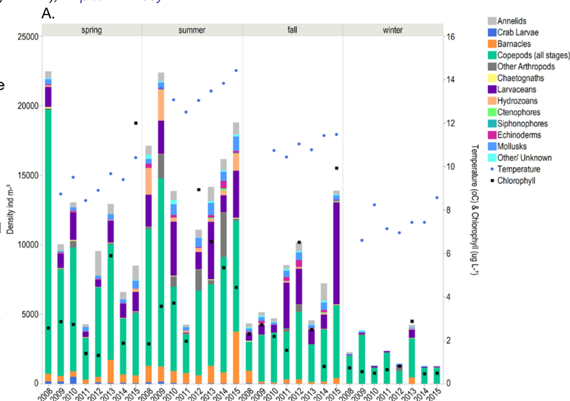
Figure 30. (A) Annual seasonal means of zooplankton density by identification group and mean seasonal water temperature and chlorophyll concentrations (right axis).
