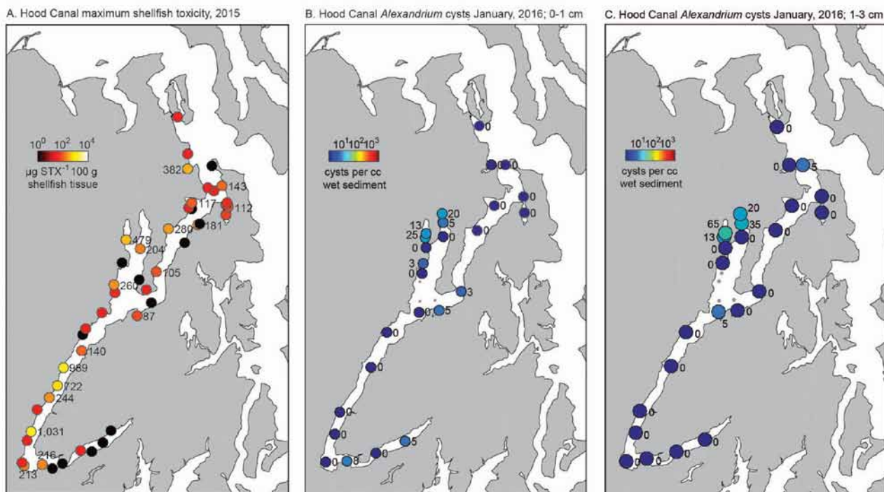
Figure 32. (A) Maximum shellfish toxicity ( \mu\text{g} saxitoxin equivalents 100 \text{ g}^{-1} shellfish tissue) in Hood Canal from January-October 2015 (WDOH), (B) Alexandrium cysts/cc wet surface sediment (0-1 cm) in Hood Canal from January 2016, and (C) Alexandrium cysts/cc wet sediment (1-3 cm) in Hood Canal from January 2016.
