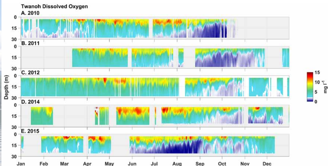
Figure 18. Time-series of DO at the Twanoh ORCA mooring from 2010 to 2015.
