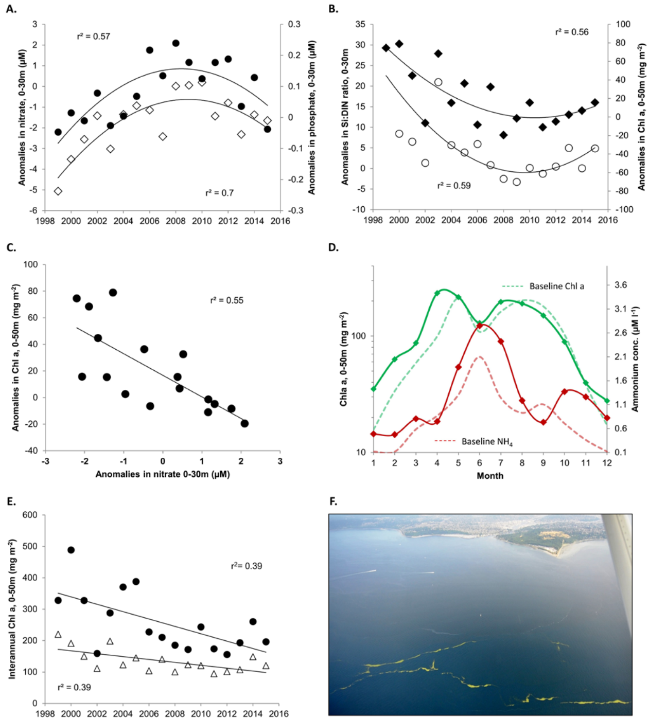
Figure 14. Puget Sound-wide annual anomalies of (A) nitrate (black circles) and phosphate (open diamond), (B) the ratio of Si:DIN (open circles) and chlorophyll-a (black diamonds) over the period of 1999-2015. (C) Puget Sound-wide long-term anomalies of nitrate plotted against chlorophyll-a. (D) Puget Sound-wide monthly averages of chlorophyll-a (green circles) and ammonium (red circles) for 2015, and the mean seasonal cycle based on 1999-2013 values (faint green line, chlorophyll-a; faint red line, ammonium). (E) Long-term trends in Puget Sound-wide average phytoplankton biomass, with annual averages (triangles) and maxima specific to the July - December period (circles), highlighting a distinctive decline in late summer. (F) Example of macroalgae occurring in Central Sound in July 2015.
