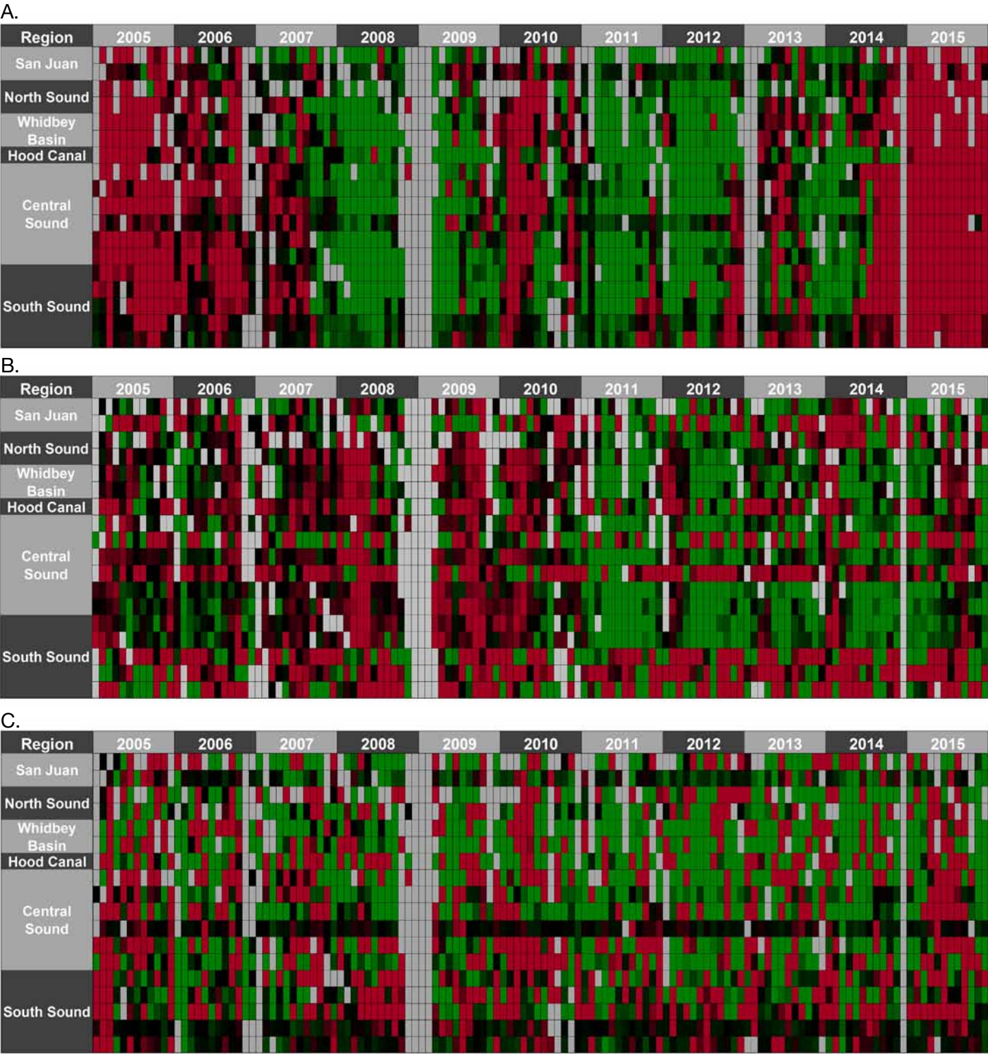
Figure 12. Heat maps of Puget Sound thermal energy (A) salt content (B) and potential energy (C) anomalies for the 0-50 m water layer for 2005-2015. Anomalies are calculated from site-specific monthly averages using a reference baseline established for 1999-2008. Green = lower, red = higher, black = expected, gray = no data.
