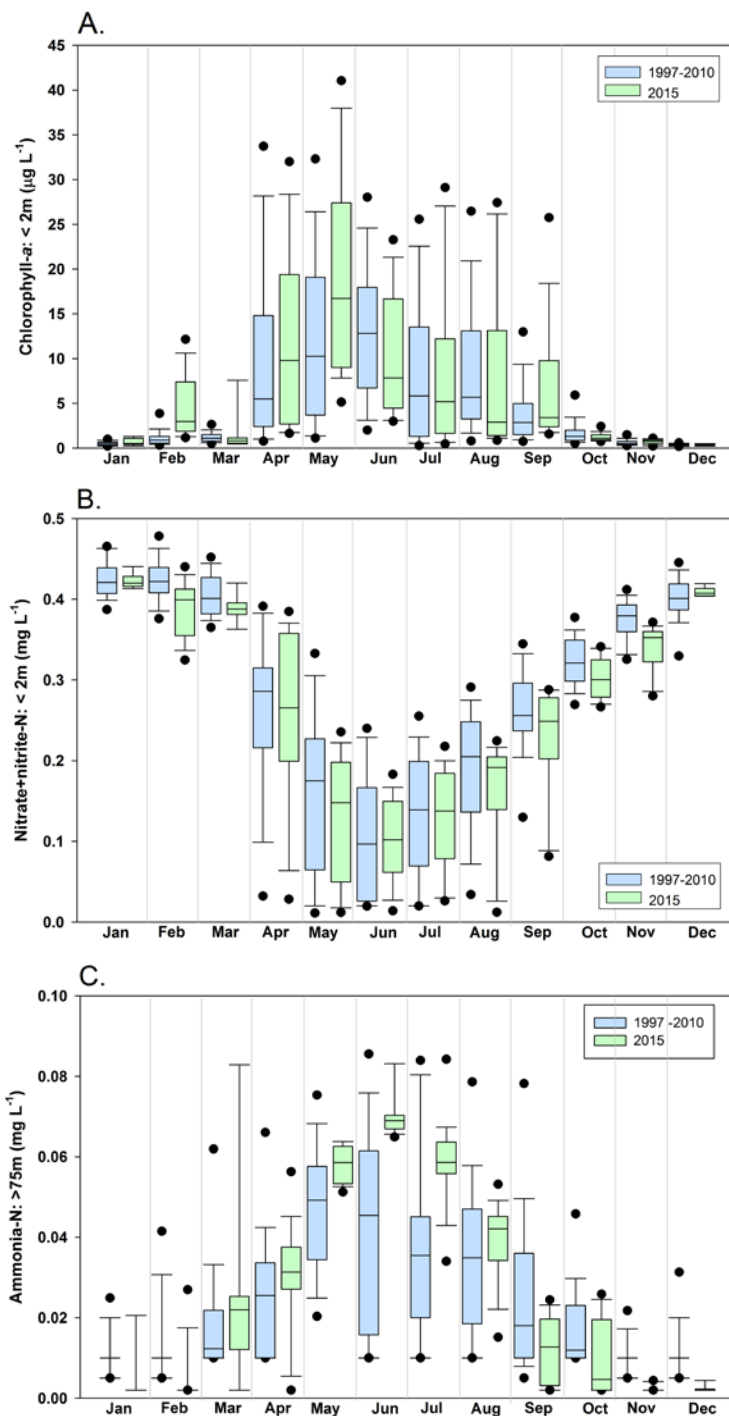
Figure 22. 2015 surface water (A) chlorophyll-a and (B) nitrate levels, and (C) deep water ammonia levels at 12 sites in the Central Basin compared to the long-term baseline. The line within the box denotes the median, box boundaries are 25th and 75th percentiles, whiskers are 10th and 90th percentiles, and points are 5th and 95th percentiles.
