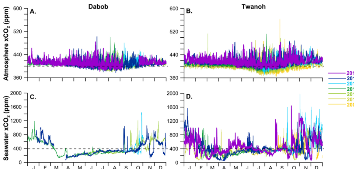
Figure 19. The mole fraction of carbon dioxide (xCO 2 ) in air at 1.5 m above seawater and surface seawater at 0.5 m depth in Dabob Bay and Twanoh in 2015. Data from previous years are included for comparison. Approximate 2015 global average atmospheric xCO 2 of 399 ppm is indicated with dashed line in each panel. Typical uncertainty associated with quality controlled xCO 2 measurements from these systems is < 2 ppm for the range 100–600 ppm, increase for values between 600 and 1000 ppm, and is not well constrained above 1000 ppm.
