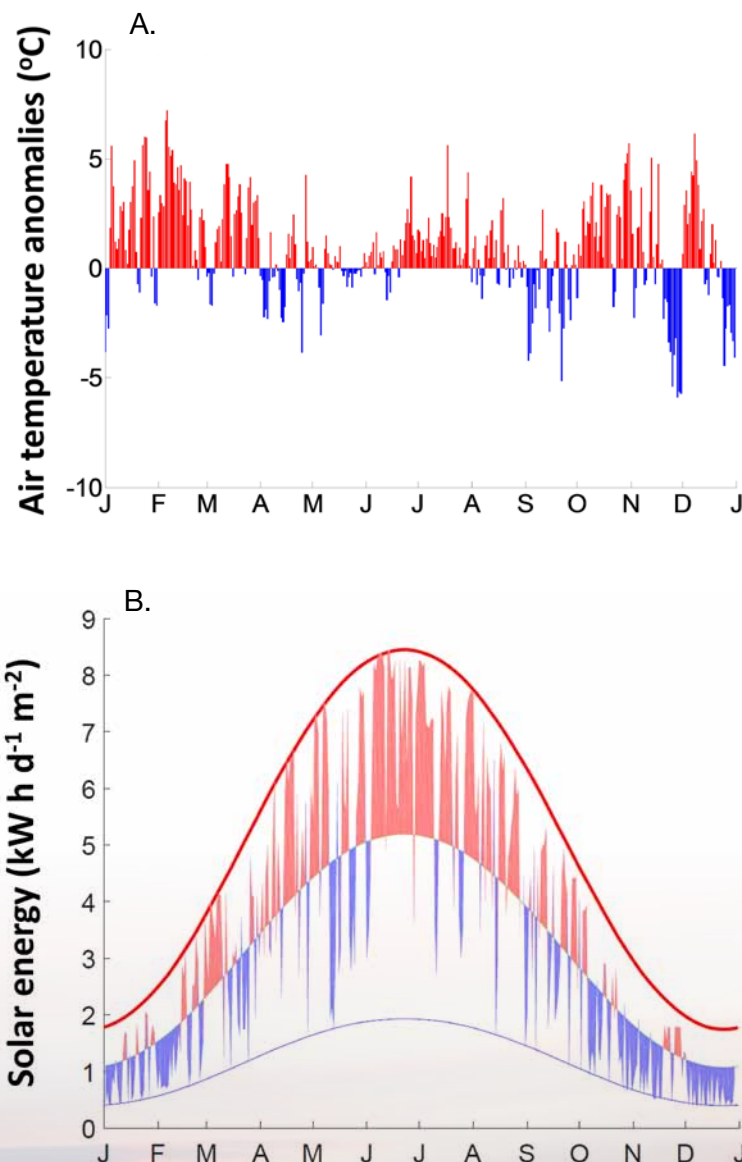
Figure 6. Air temperature anomalies (A) and daily solar energy flux (B) at Sea-Tac Airport and UW, respectively, in 2015. Red shading in (A) indicates higher than average and blue indicates lower than average air temperature. The solid red line on the solar energy panel (B) shows the highest theoretical solar energy for this latitude, and the blue line is the solar energy if completely overcast. Red shading indicates when the sky is more than 50% clear (sunnier) and blue shading indicates when it is less than 50% clear (cloudier).
