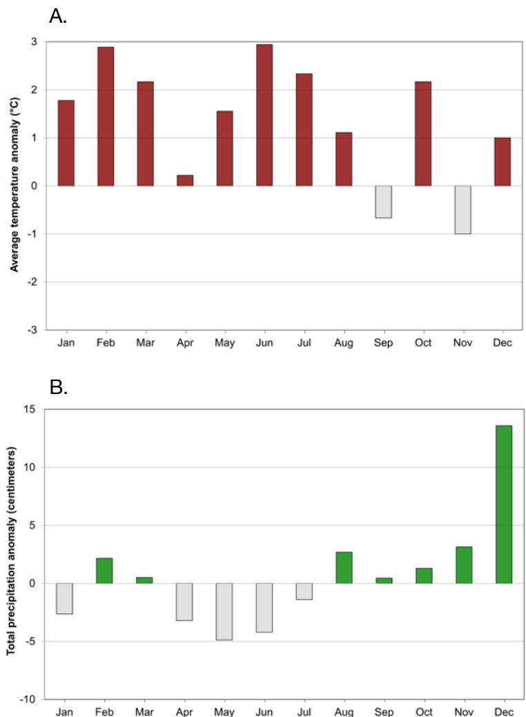
Figure 5. Monthly anomalies for (A) temperature (Celsius) and (B) precipitation (centimeters) for the Puget Sound Lowlands climate division in Washington State for the 2015 calendar year. Anomalies are relative to 1981-2010 climate normals.
