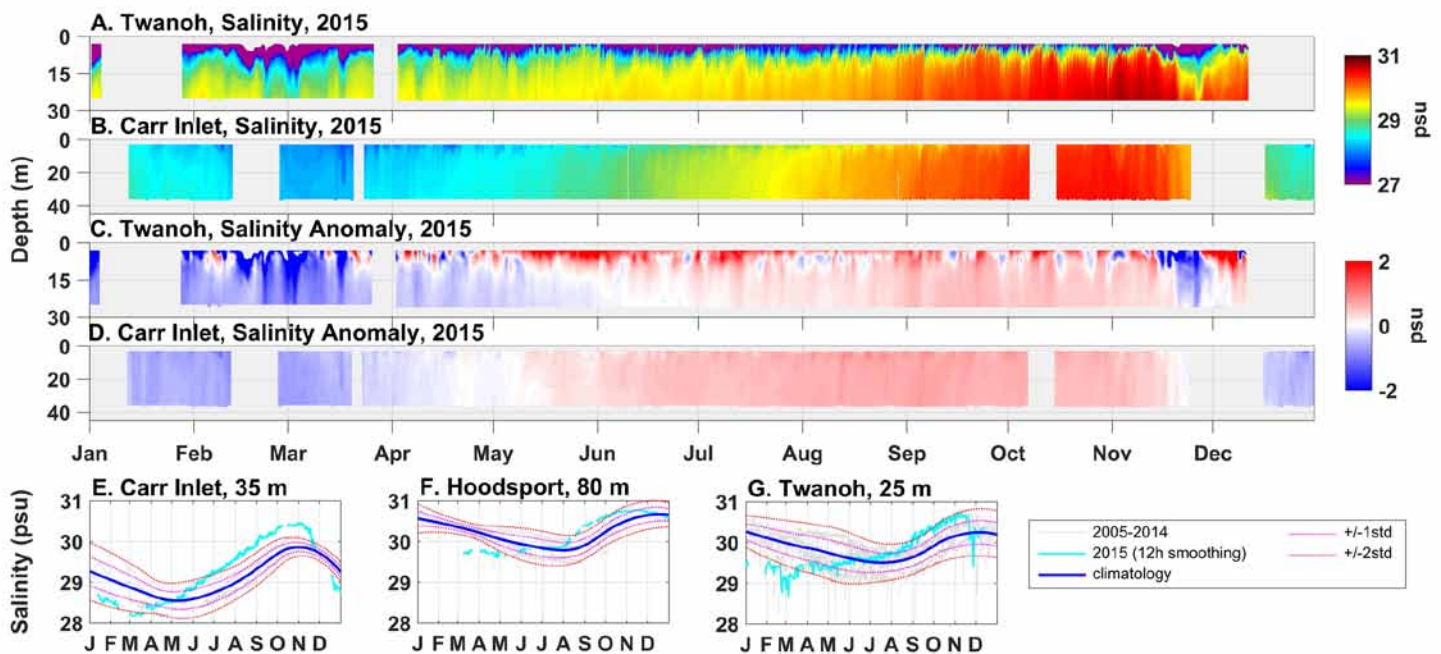
Figure 17. (A) and (B): Salinity data for Twanoh and Carr Inlet for 2015. (C) and (D): Salinity anomalies (2015 – climatology) for Twanoh and Carr Inlet. Data are colored by a white threshold at 0, with red indicating saltier and blue fresher than historical average conditions. (E), (F), (G): 2015 data (cyan line), climatology (dark blue line), and all historical data (grey lines) for near bottom salinity at Carr Inlet, Hoodsport, and Twanoh; also shown are \pm 1 SD from the climatology (pink dotted line) and \pm 2 SD from the climatology (red dotted line).
