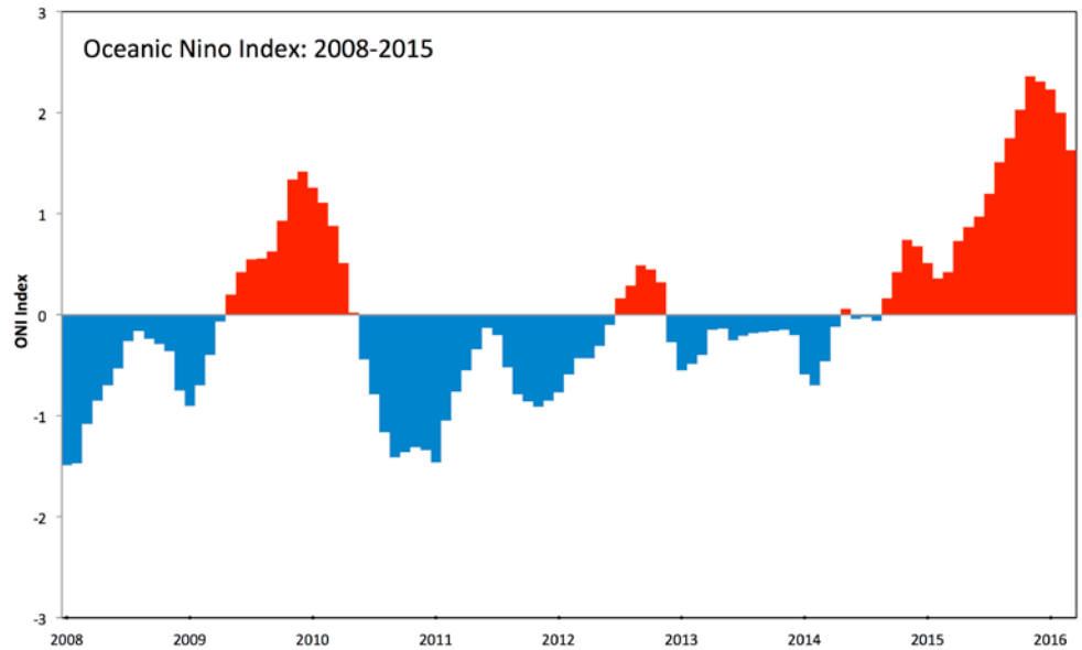
Figure 1B. Oceanic Niño Index (ONI) values from 2008-2015.
