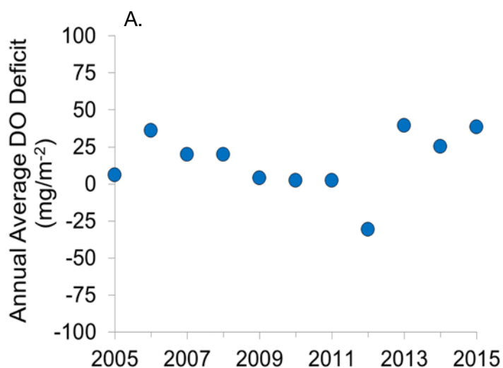
Figure 13A. Puget Sound monthly dissolved oxygen (DO) deficit anomalies from 2005-2015 for water deeper than 20 m using a reference baseline established from 1999- 2008. (A) Puget Sound-wide annual anomaly of the DO deficit from 2005-2015.
