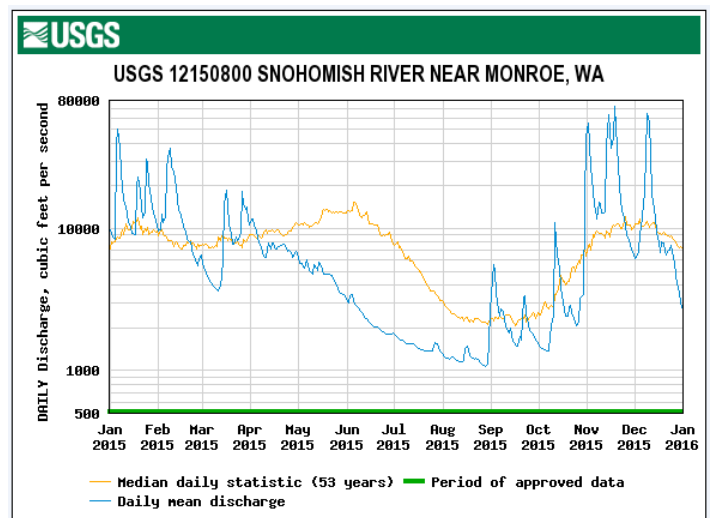
Figure 11. Daily discharge (cfs) at stations in Nooksack, Skagit, Snohomish, Puyallup, Nisqually, and Skokomish Rivers in 2015, compared to long-term median values. Note the period of record varies and is indicated separately for each station.
