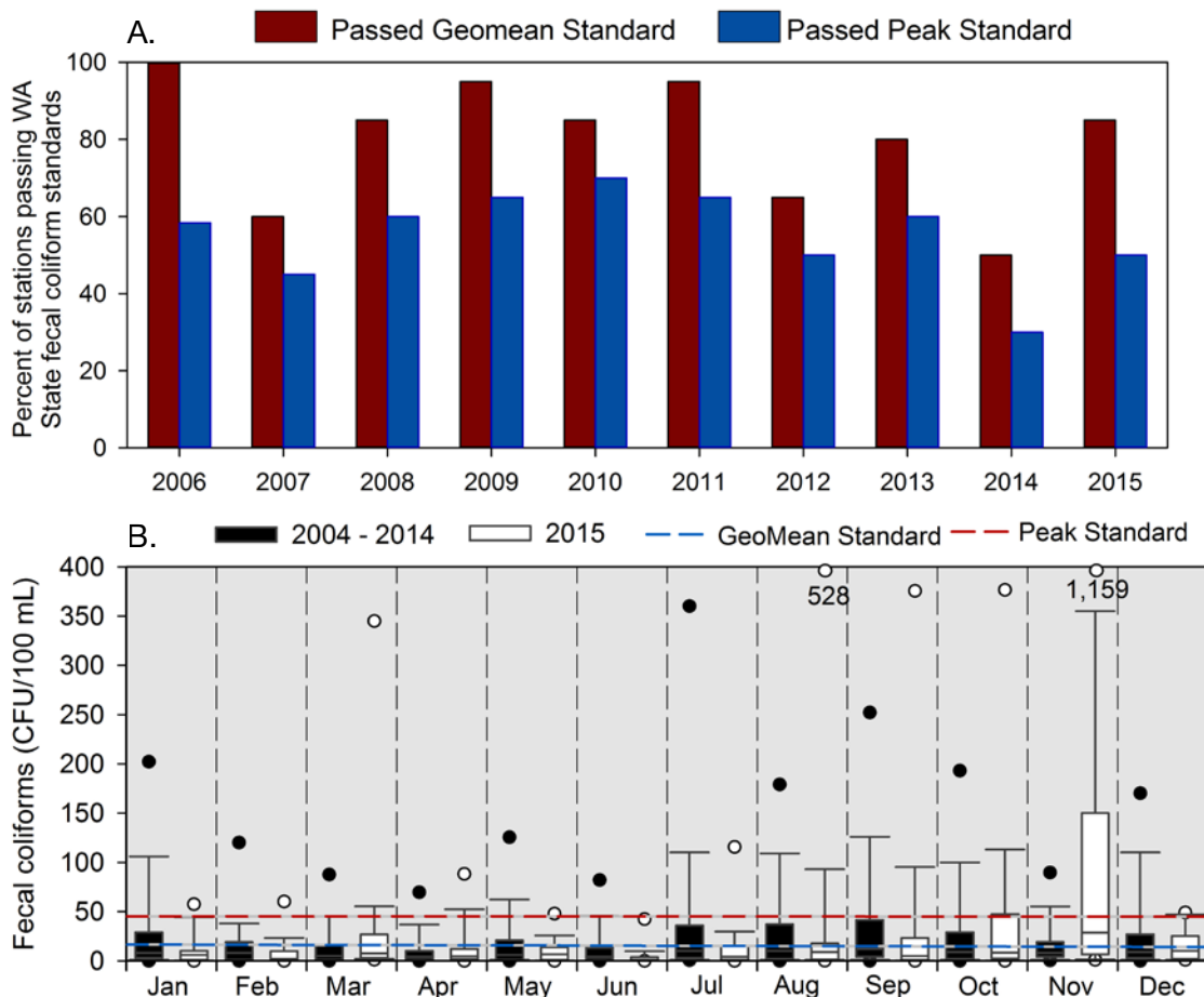
Figure 34. King County marine beach fecal coliform data: (A) Proportion of beach stations passing fecal coliform standards annually in 2006 – 2015; (B) Monthly fecal coliform concentrations at all beach sites in 2015 compared to 2004 to 2014 data.
