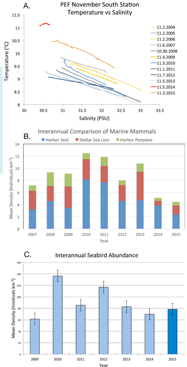
Figure 25. (A) Temperature versus salinity from 80 m to the surface at the South station in the eastern Strait of Juan de Fuca during the first week of November. Deep waters (coldest and saltiest) are found on the right. Color coding shows: yellow=El Niño years; blue=La Niña years; gray=neutral years. (B) Marine mammal density from 2007 to 2015. (C) Marine bird density from 2009 to 2015.
