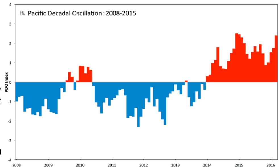
Figure 2. Monthly values of the Pacific Decadal Oscillation (PDO) Index from (A) 1950-2015 and (B) 2008-2015.
