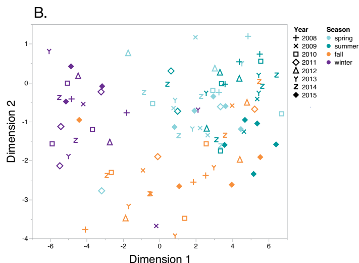
Figure 30. (B) Multi-dimensional scaling ordination of zooplankton community with season coded by color and year coded by symbol.
