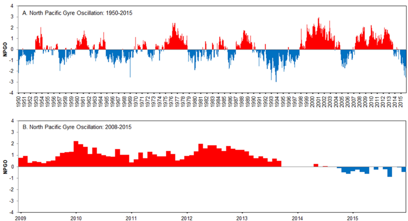
Figure 3. Monthly values of the North Pacific Gyre Oscillation index (NPGO) from (A) 1950-2015 and (B) 2008-2015.
