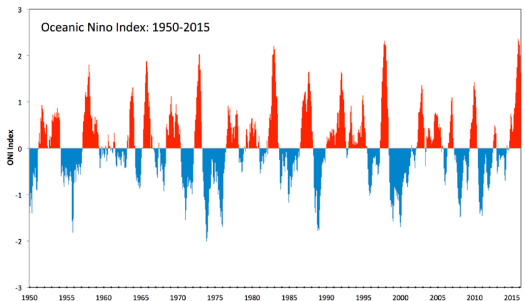
Figure 1A. Oceanic Niño Index (ONI) values from 1950-2015.
