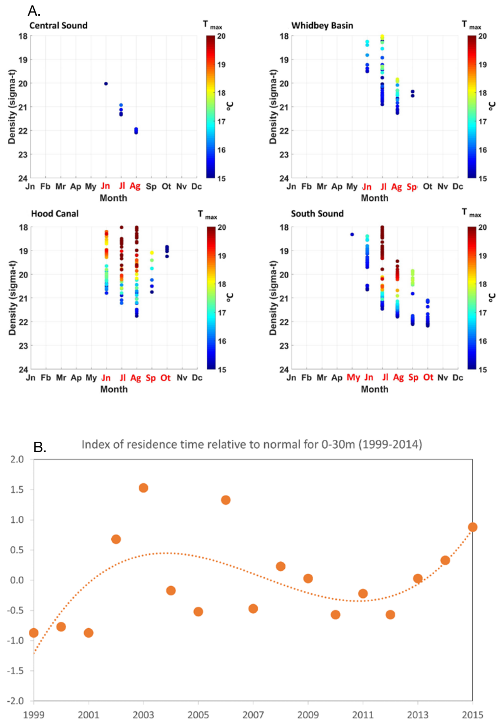
Figure 15. (A) Monthly plots of water temperatures exceeding 15^{\circ}\text{C} versus density with color showing temperature exceedance. Results are shown for Central, Whidbey, Hood Canal, and South basins. (B) Residence time index for Central Basin.
