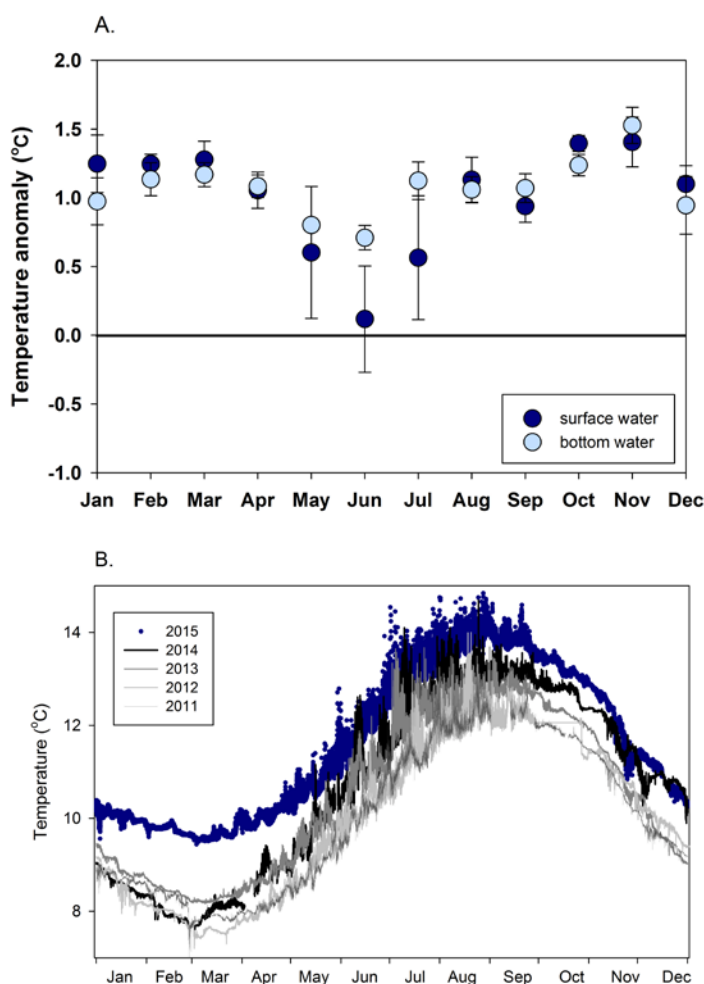
Figure 20. (A) Mean of 2015 temperature anomalies for six sites relative to a baseline average (1999–2010). Negative values indicate colder than baseline temperatures. (B) Water temperature at the Seattle Aquarium mooring (10 m depth, collected at 15-minute intervals). (C) Water column density at East Passage.
