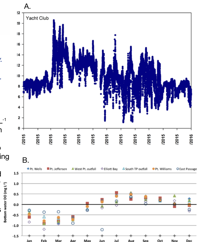
Figure 21. (A) 2015 DO concentrations in inner Quartermaster Harbor (Yacht Club). Data were recorded at 1-m depth every 15-minutes. (B) 2015 DO anomalies in bottom waters at representative sites in the Central Basin. 2015 values are compared to the 1999-2010 baseline.
