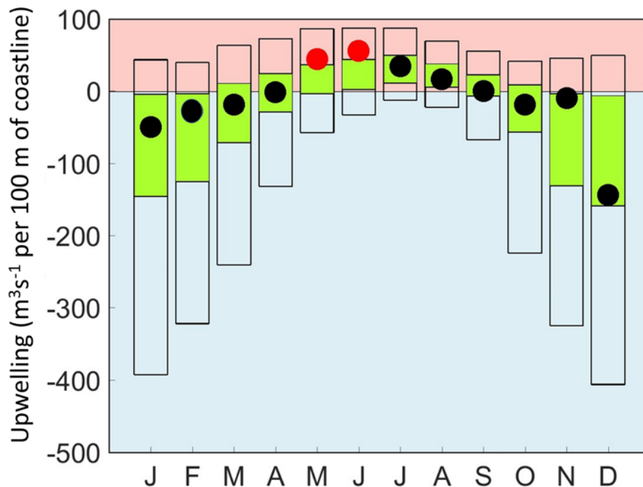
Figure 4. Monthly mean values of the PFEL coastal upwelling index for 2015 (red and black dots) are presented in historical statistical context based on the index values at 48 °N and 125 °W from 1967 to 2014. The box plot extent represents 5 th and 95 th percentiles with the interquartile range between the 25 th and 75 th percentiles shaded green. Values falling outside the interquartile range are colored red. Pink and blue shaded areas indicate upwelling and downwelling conditions, respectively. Data source: www.pfeg.noaa.gov/products/las/docs/upwell.nc.html .
