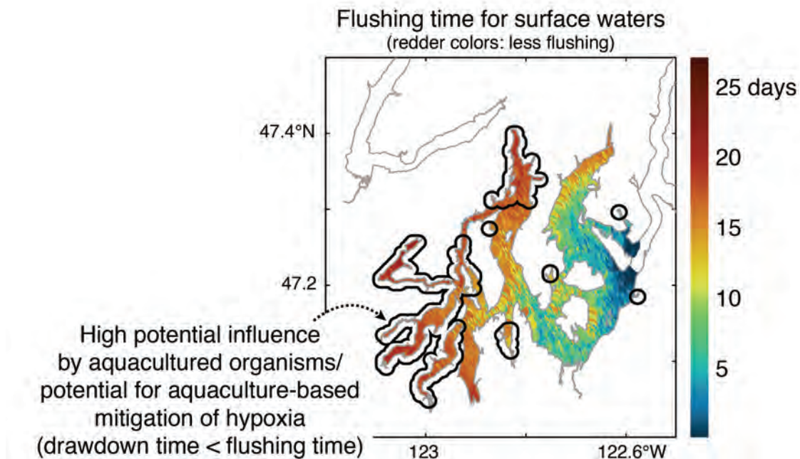
Figure 6. Average flushing time for surface waters in South Puget Sound in preliminary analyses.
