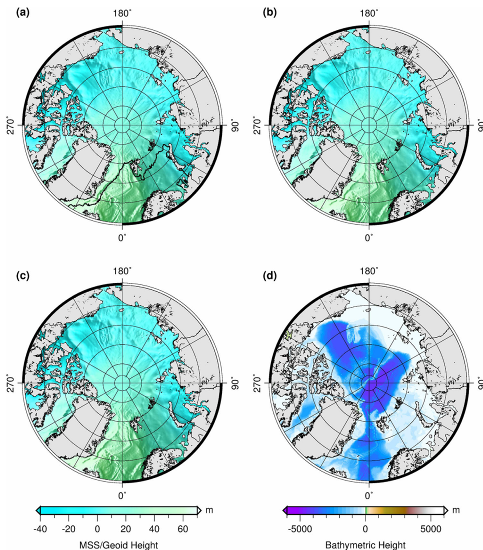
Figure 1. (a) UCL13 mean sea surface (MSS) of the Arctic Ocean, including the 15% sea ice concentration contour for April 2015, (b) DTU15 MSS of the Arctic Ocean, (c) EGM2008 global gravity model (GGM) of the Arctic Ocean, and (d) International Bathymetric Chart of the Arctic Ocean (IBCAO).
