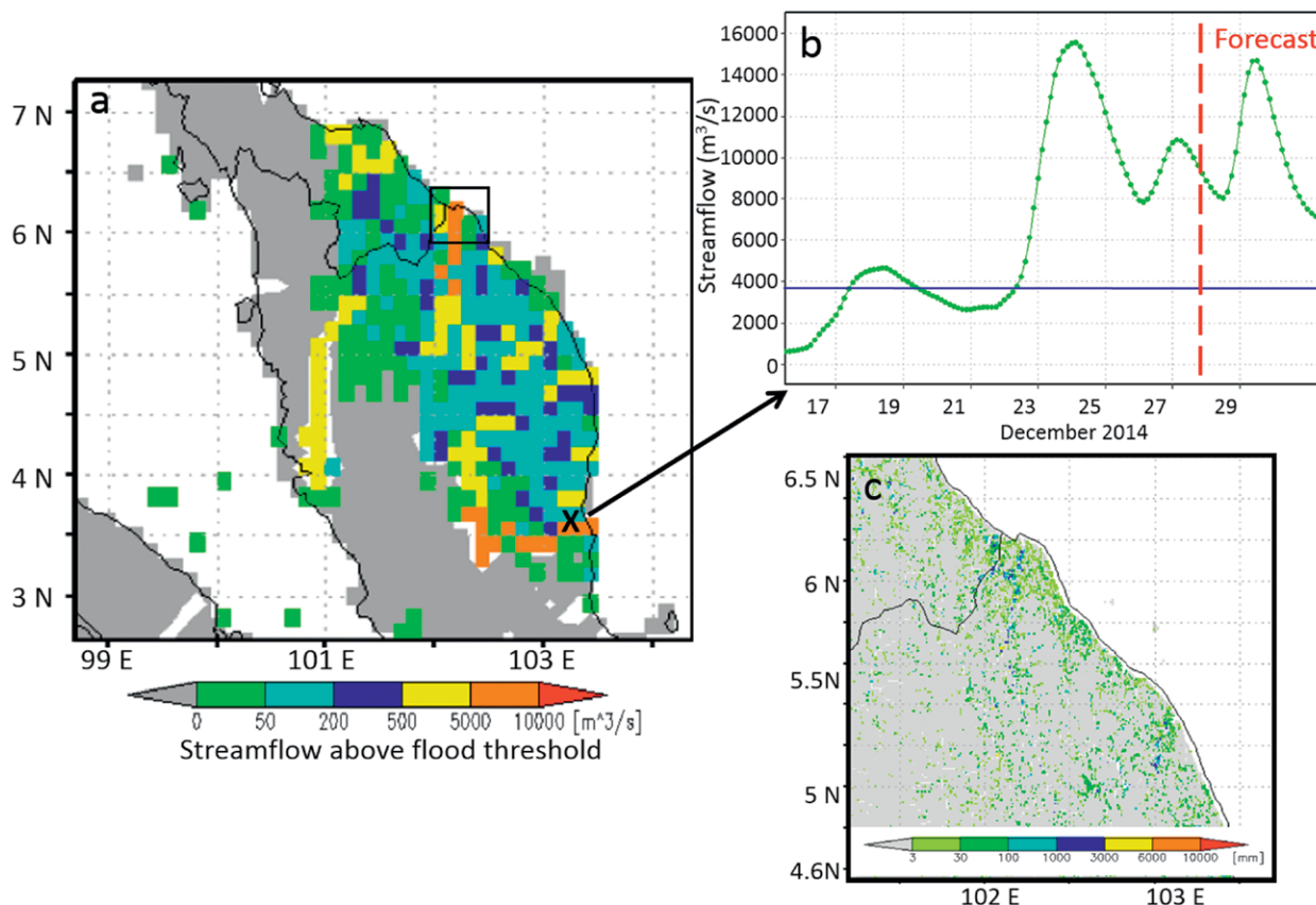
FIG. 5. Malaysia flooding in Dec 2014 as estimated from GFMS, showing (a) a map of streamflow above flood threshold on 27 Dec, (b) streamflow time history (green) at a point (indicated by the X) including the forecast (right side of red vertical line) from 27 to 31 Dec [note the streamflow flood threshold (blue) at the point in question], and (c) 1-km inundation estimate for inset black box shown in (a).
