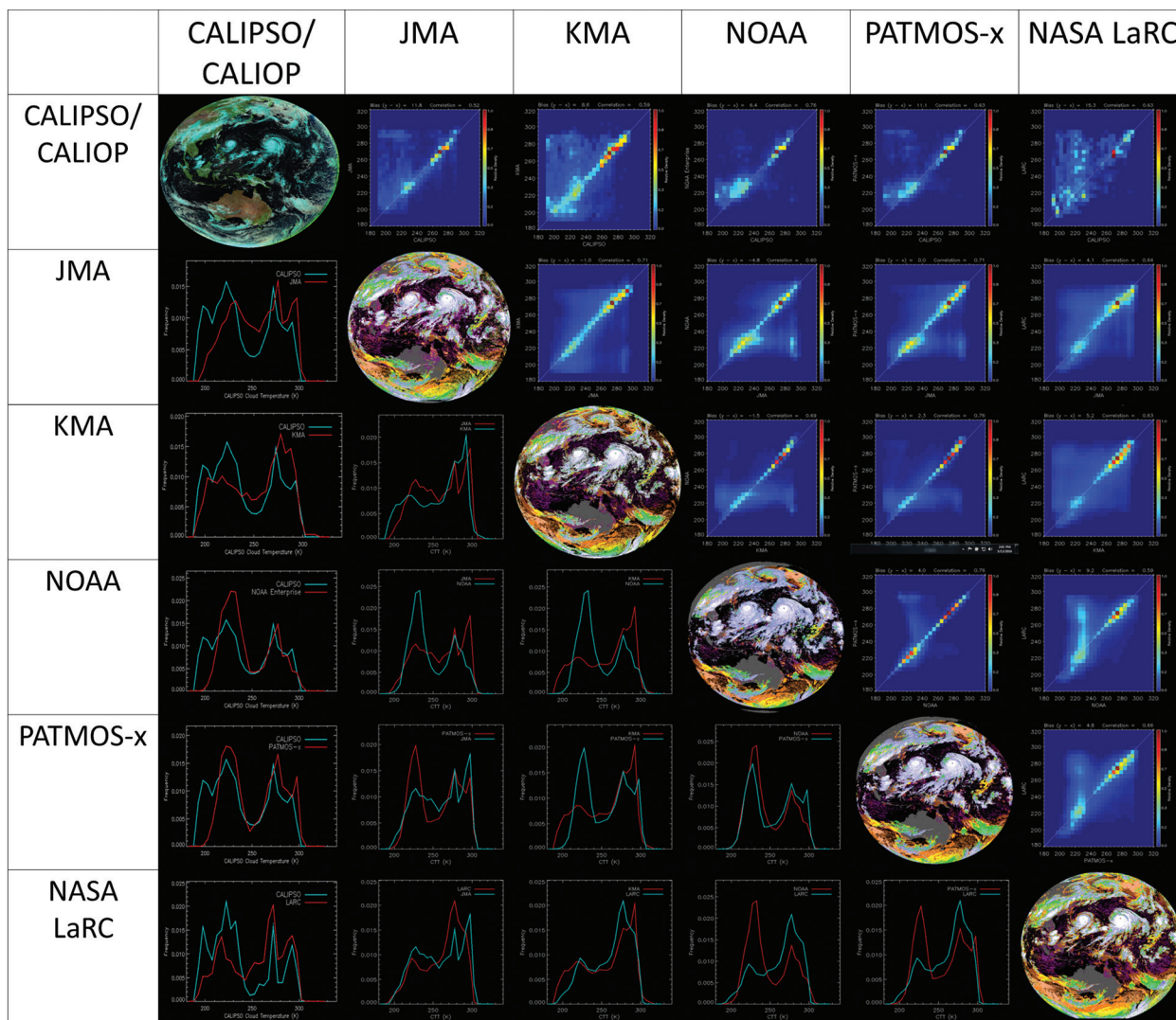
FIG. 1. Intercomparisons of cloud-top temperature (CTT) on the golden day (19 Aug 2015) in terms of 2D histogram (top-right panels) and pdf (bottom panels).
