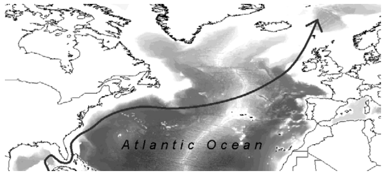
Figure 1: The Gulf Stream current originates in the Gulf of Mexico and carries a current of warmer water through the North Atlantic.
