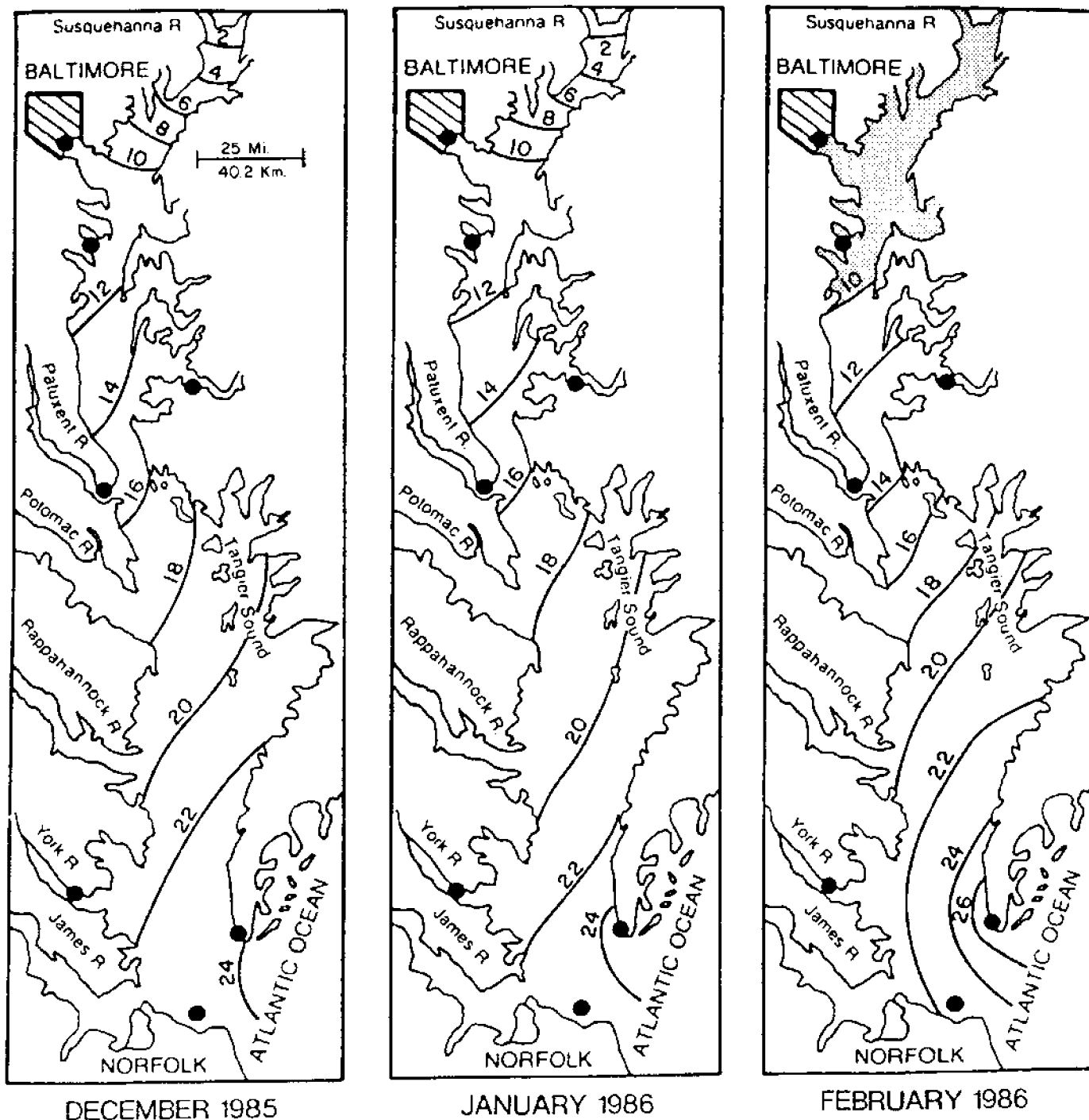
Figure 6--Mean surface salinity distribution, Chesapeake Bay, December 1985 - February 1986. Isohalines (parts per thousands) are linearly interpolated from designated station data from the National Ocean Service, NOAA. Salinities in shaded area could not be interpolated for February due to lack of data (equipment malfunction) at Baltimore.
