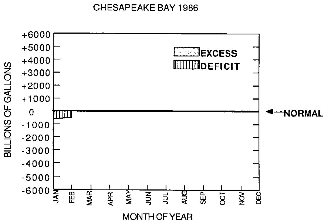
Figure 5--Cumulative monthly streamflow anomaly, Chesapeake Bay, 1985 and 1986.
