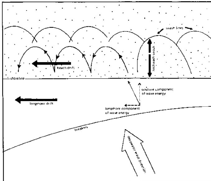
Figure 24. Diagram of littoral drift
