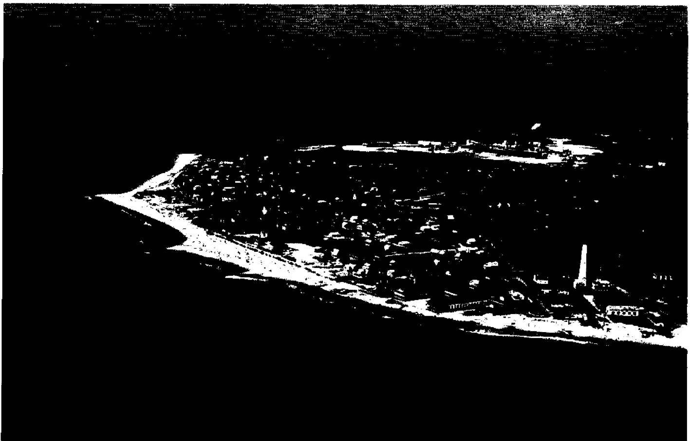
Figure 10. View northwest at Cape May Point (Courtesy of US Army Corps of Engineers, Philadelphia District)
