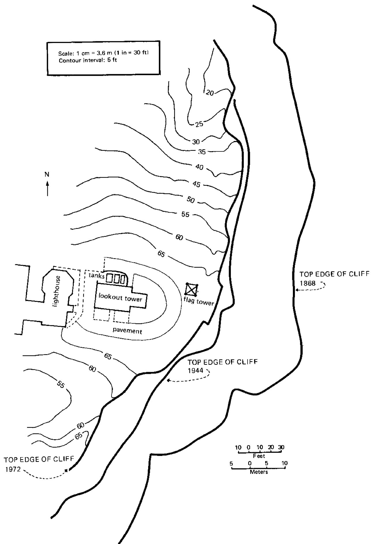
Figure 13. Changes in position of top edge of cliff at Montauk Point, 1868 to 1972 (After Third US Coast Guard District, NY)
