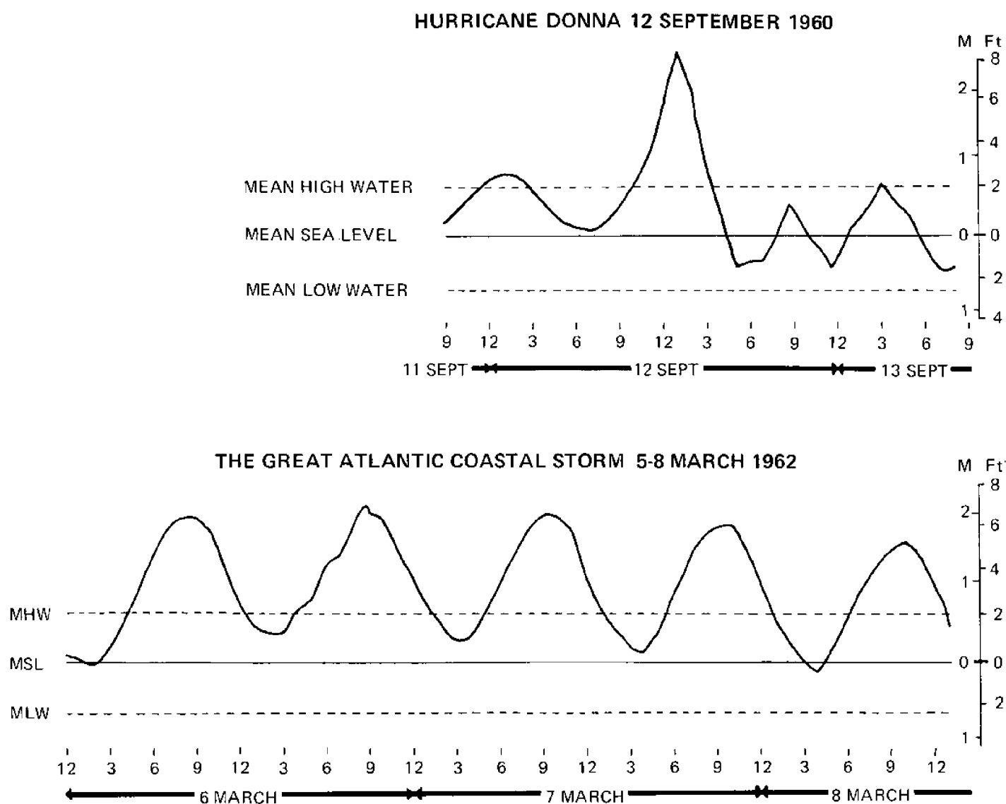
Figure 25. Storm surge superimposed on astronomical tides at The Battery, NY, 12 September 1960 and 5-8 March 1962 (After US Army Corps of Engineers, NY District)
