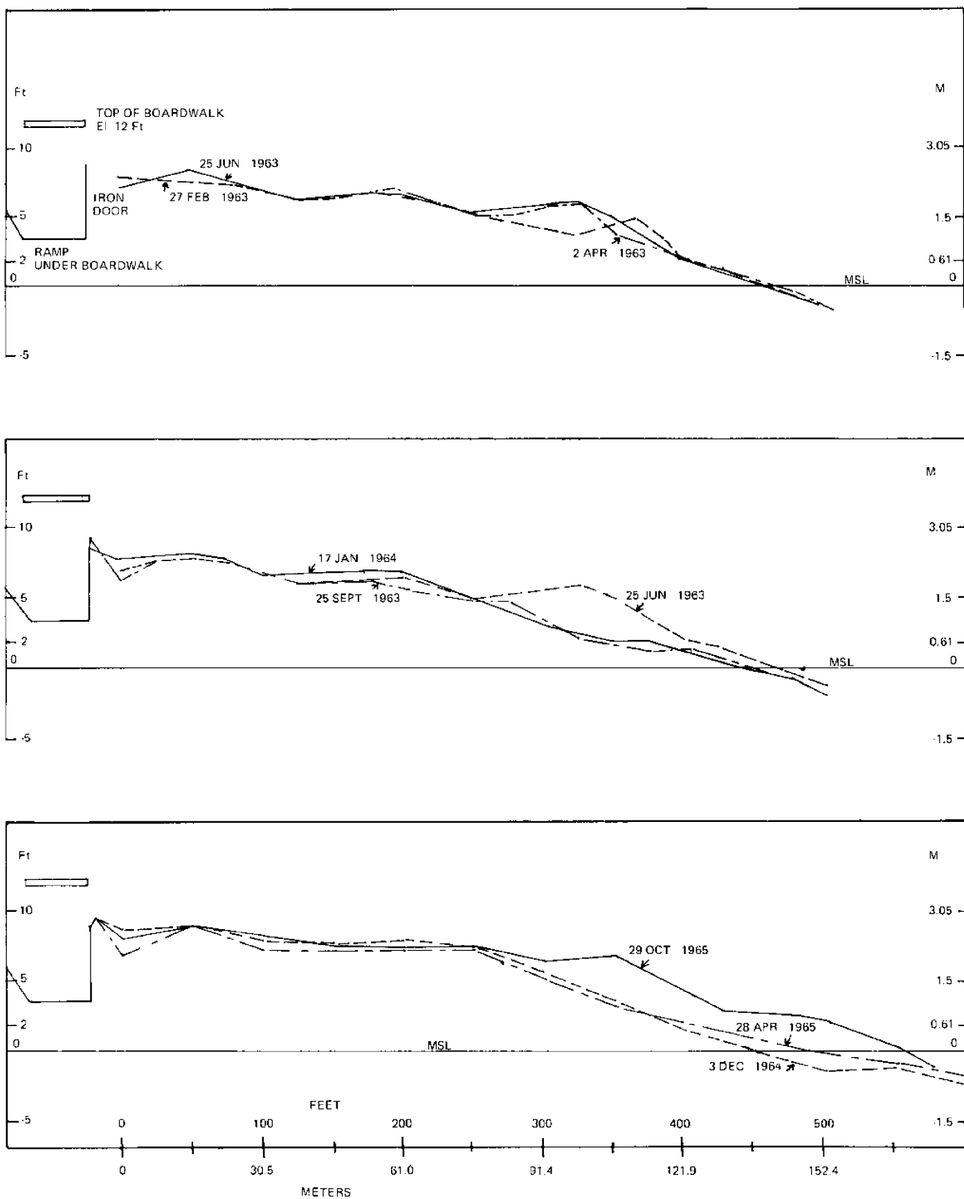
Figure 38. Topographic profiles — California Avenue, Atlantic City, 27 February to 29 October 1965 (After US Army Corps of Engineers, Philadelphia District)
