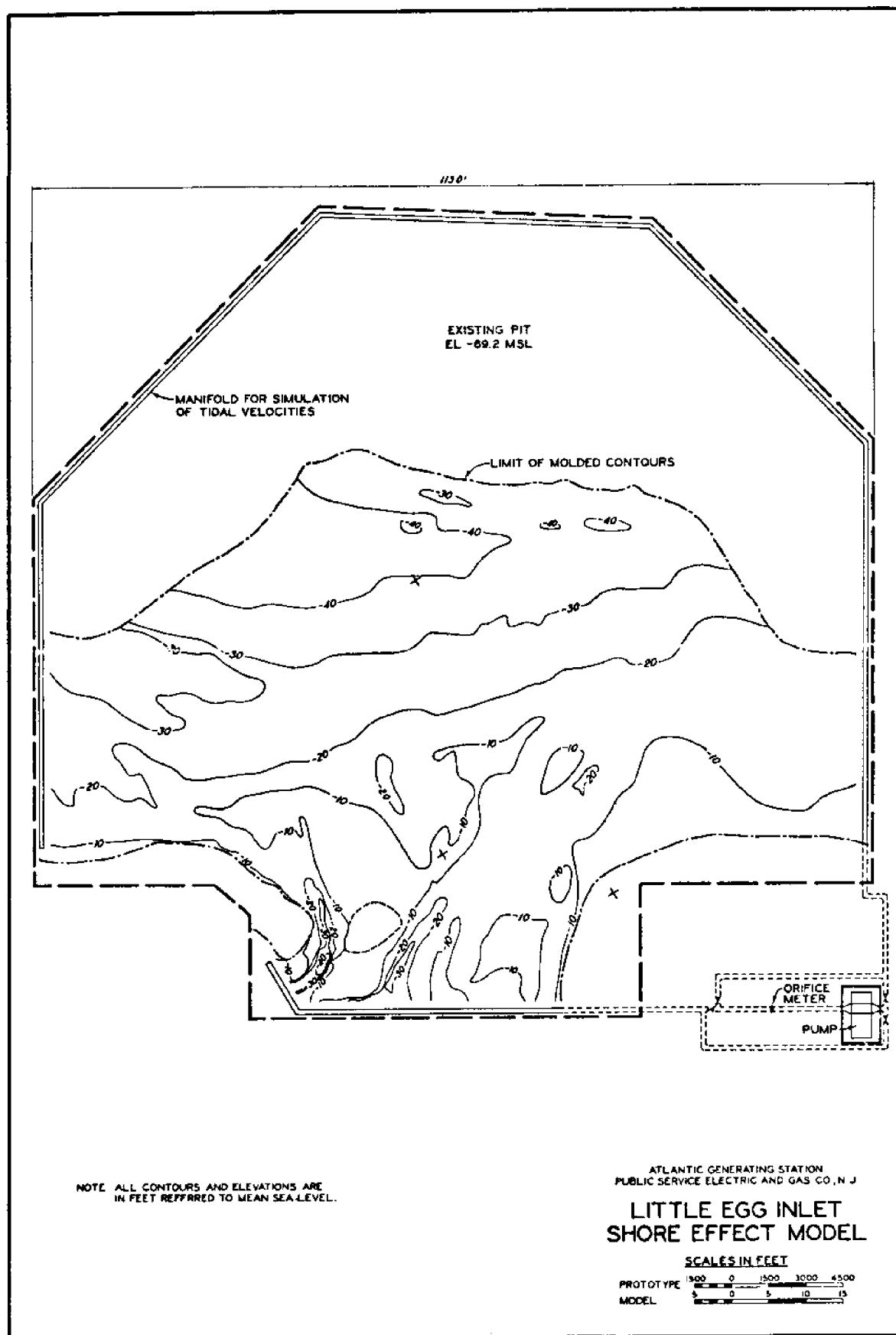
Figure 34. Bottom contours and test basin configuration for Little Egg Inlet model study (Courtesy of US Army Corps of Engineers Waterways Experiment Station, Vicksburg, MS)
