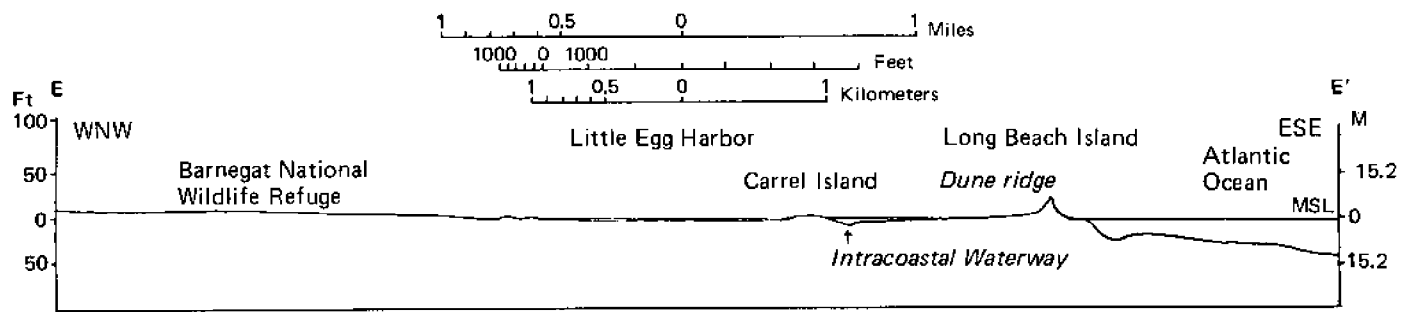
Figure 6. Topographic profile -- Harvey Cedars, NJ (barrier complex)
