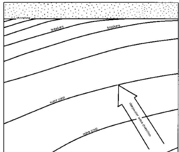
Figure 23. Diagram of wave refraction
