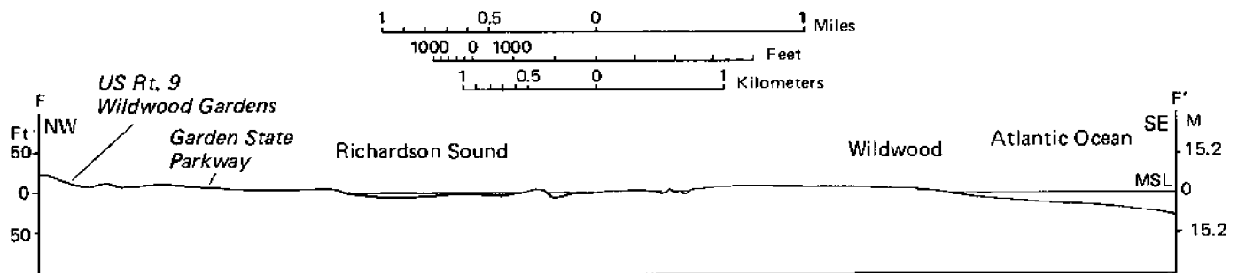
Figure 7. Topographic profile -- Wildwood, NJ (barrier complex)
