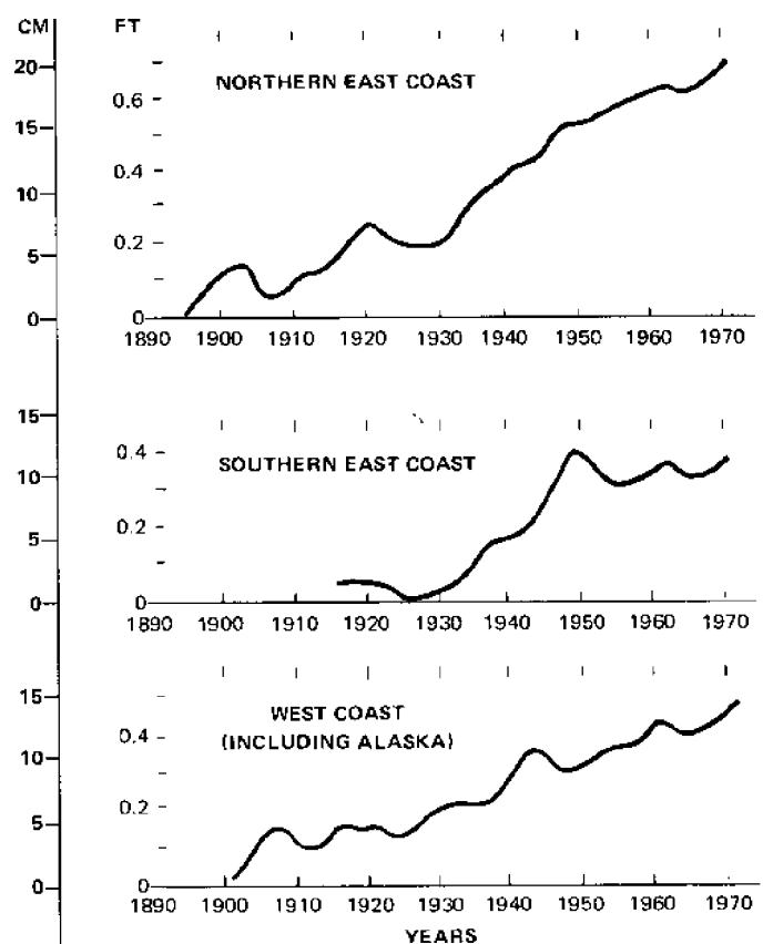
Figure 28. Mean sea-level changes (After Hicks 1972)
