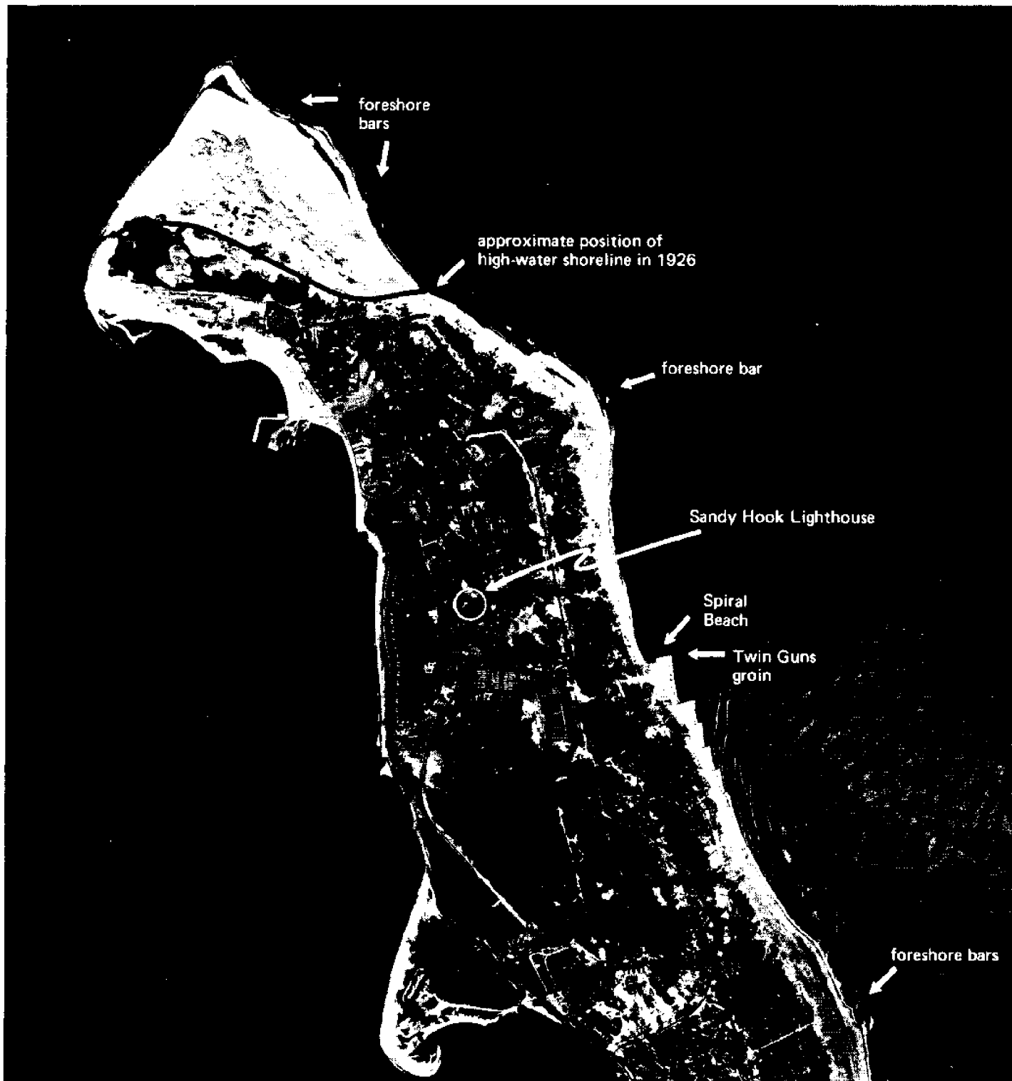
Figure 20. Northern portion of Sandy Hook (US Coast and Geodetic Survey aerial photo No. W4545, 4 May 1962)
