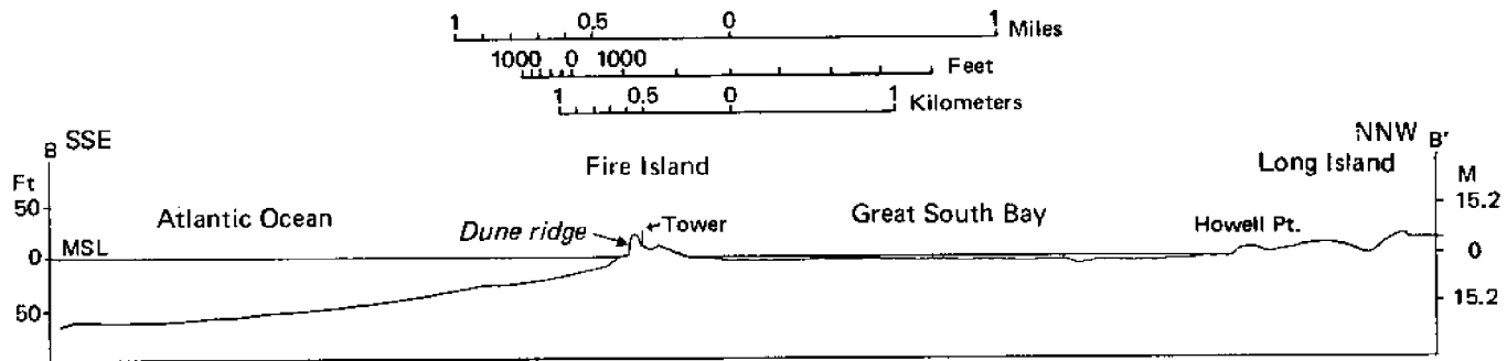
Figure 3. Topographic profile — Fire Island, NY (barrier complex)
