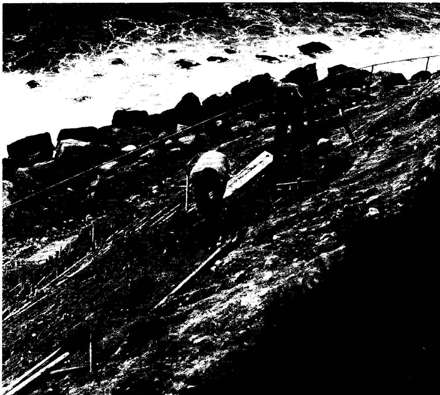
Figure 31. Cliff terracing, Montauk Point, 25 September 1971 (Courtesy of Third US Coast Guard District, NY)
