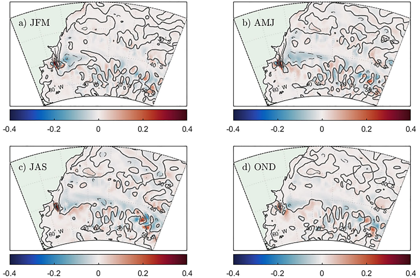
Figure 10. (a–d) Deterministic pressure gradient force Run minus Control Run of indicated 50-year seasonal mean of potential temperature (colormap) and salinity (contour lines in increments of 0.02 psu) at 2.5 m.
