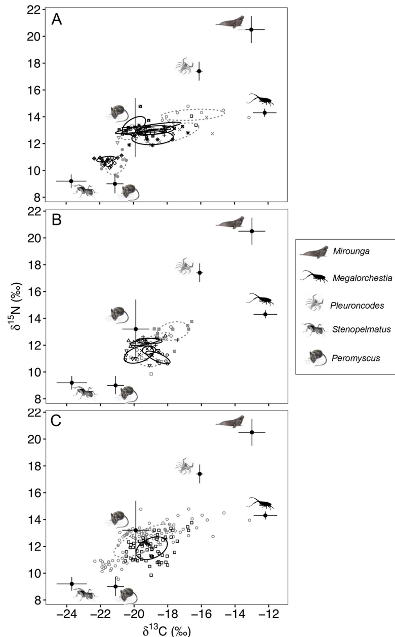
Fig 6. Bivariate plots of island fox whisker segment \delta^{13}\text{C} and \delta^{15}\text{N} values for Soledad and China Camp beaches. (A) Soledad and (B) China Camp beaches, and (C) comparison of populations from the two sites. The two beaches were sampled within two weeks of each other. Isotopic niche width visualized as standard ellipses enclosing 40% of the isotope space for individual foxes and for populations at each site. Dashed gray lines enclosing values for males, solid black lines enclosing females. Standard ellipse areas ( \text{SEA}_C and \text{SEA}_F ) for individuals and each population are given in Table 3. Mean \delta^{13}\text{C} and \delta^{15}\text{N} values of potential foods, included for context, are adjusted upward to account for expected trophic discrimination between fox and food (TDFs: \Delta^{13}\text{C} = 2.6\text{‰} and \Delta^{15}\text{N} = 3.4\text{‰} ).
