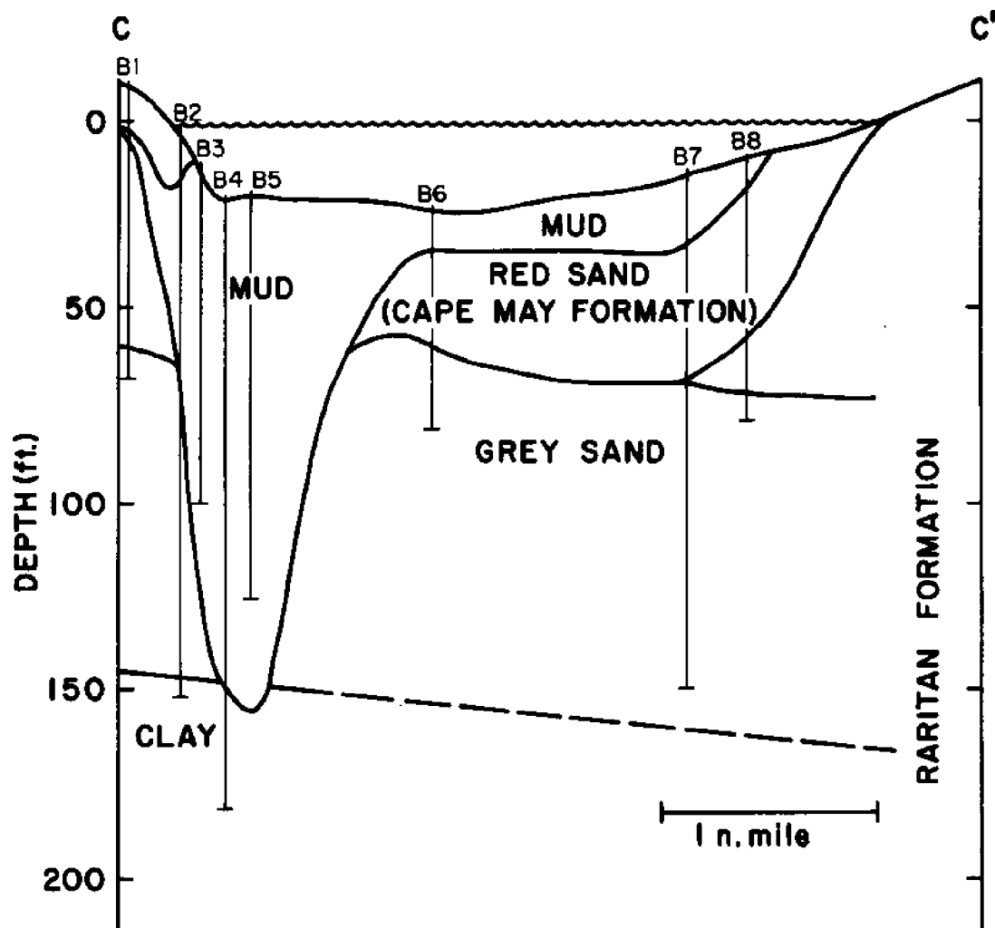
Fig. 7. Section CC' from Staten Island to New Jersey (after MacClintock and Richards, 1936). Thin vertical lines show the positions of borings along this section.
