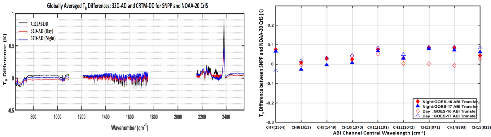
Figure 2. (a) Comparison of SNPP and NOAA-20 CrIS inter-sensor calibration radiometric biases at 2211 channels using the methods of 32D-AD and CRTM-DD, where the data cover the period from September 27 through October 28, 2019. (b) SNPP and NOAA-20 CrIS inter-sensor calibration radiometric biases using the ABI-DD method [Yan et al., 2021].
