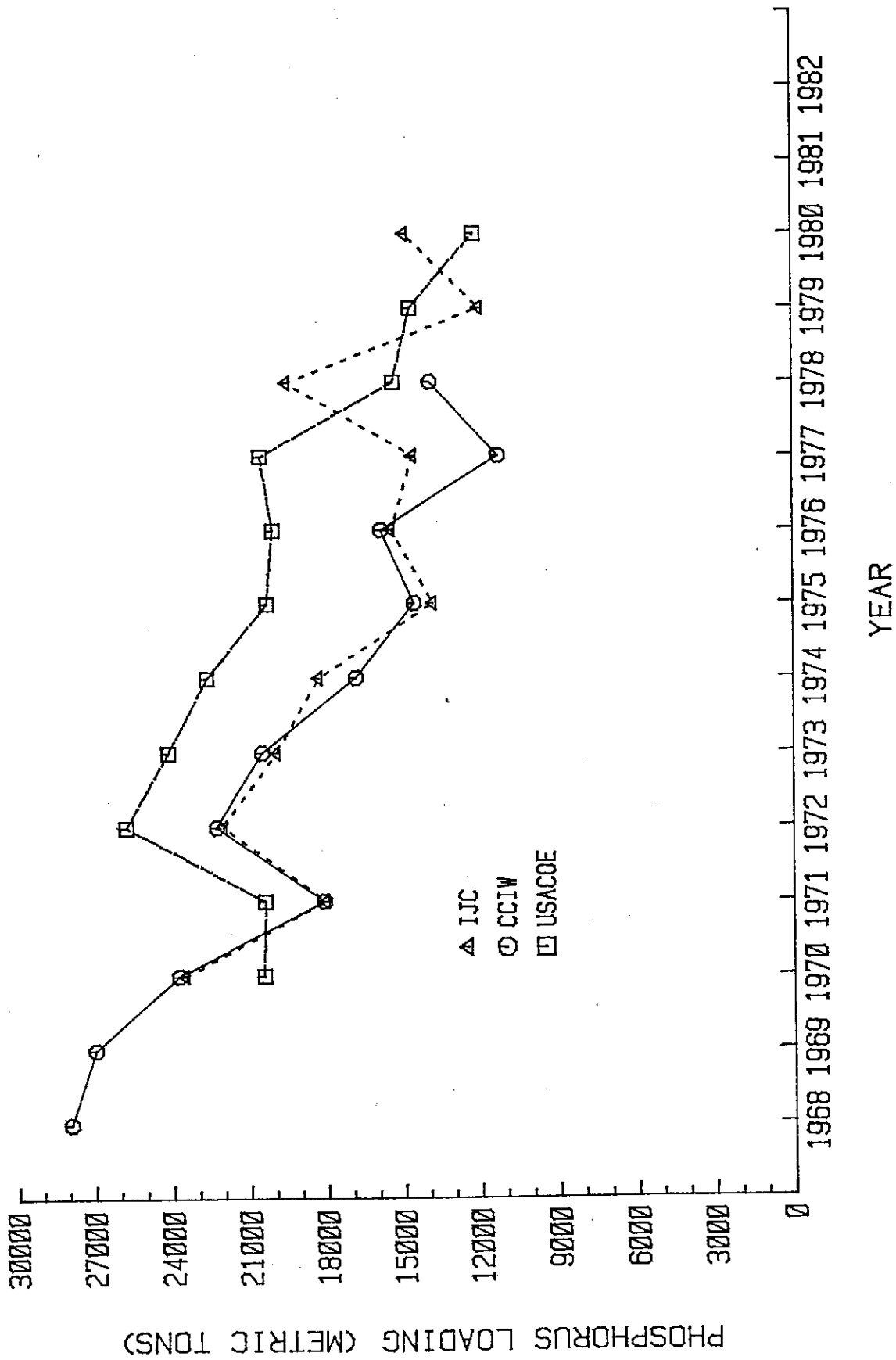
FIGURE 27. COMPARISON OF TOTAL PHOSPHORUS LOADING ESTIMATES TO LAKE ERIE
