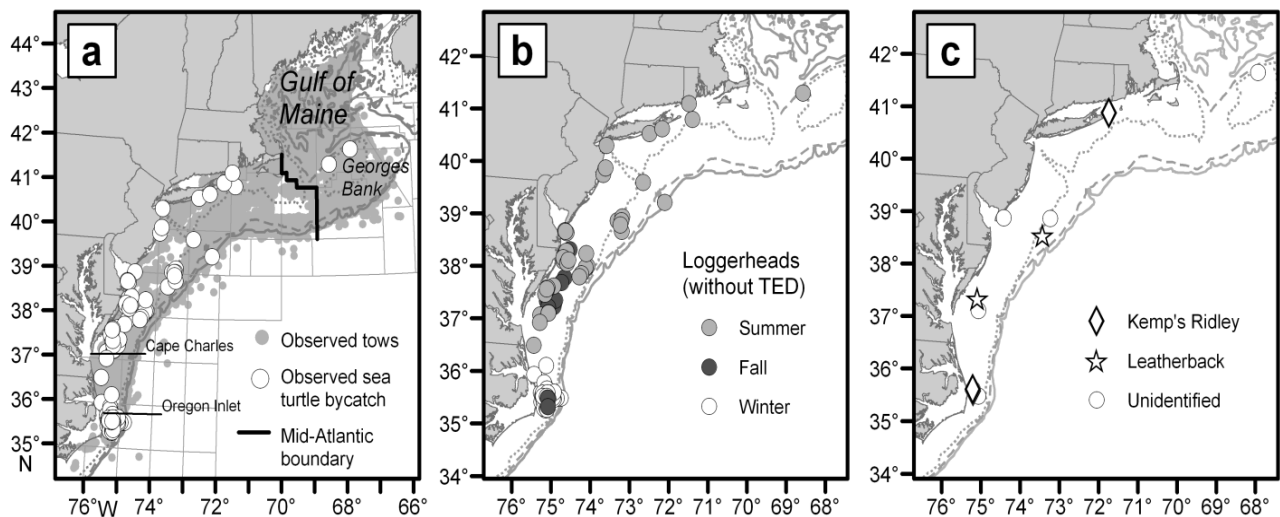
Figure 21 - a) Observed bottom trawls for fish and scallops and observed sea turtle bycatch, June 1994–Dec 2008. The extent of the Mid-Atlantic (thick black line) is delineated along statistical areas (thin gray lines). b) Loggerhead bycatch in non-TED trawls by season: spring (16 Apr–15 May, none observed); summer (16 May–31 Oct, n=44); fall (1 Nov–30 Nov, n=13); winter (1 Dec–15 Apr, n=55). c) Non-loggerhead bycatch. The 50 m (dotted), 100 m (dashed) and 200 m (solid) depth contours are shown. From: Warden (in press).
