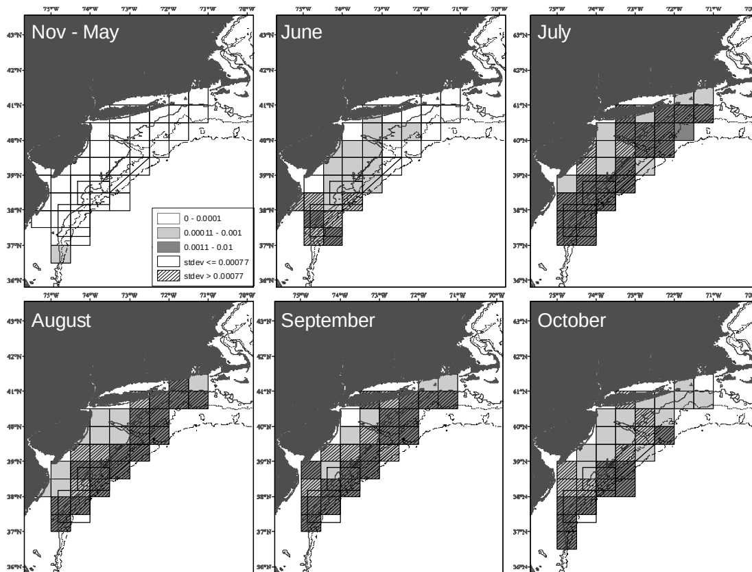
Figure 26 - Distribution over 30' squares of average predicted interaction rates without chain mats on VTR dredge trips, 2001-2008. Squares with fewer than 10 VTR trips have been excluded. The 50m,70m, and 200m bathymetry lines are shown. From north to south, the Hudson Canyon Access Area, Elephant Trunk, and Delmarva scallop management areas are represented by the black rectangles. Median standard deviation around rates over all months = 0.00077. From Murray 2011.
