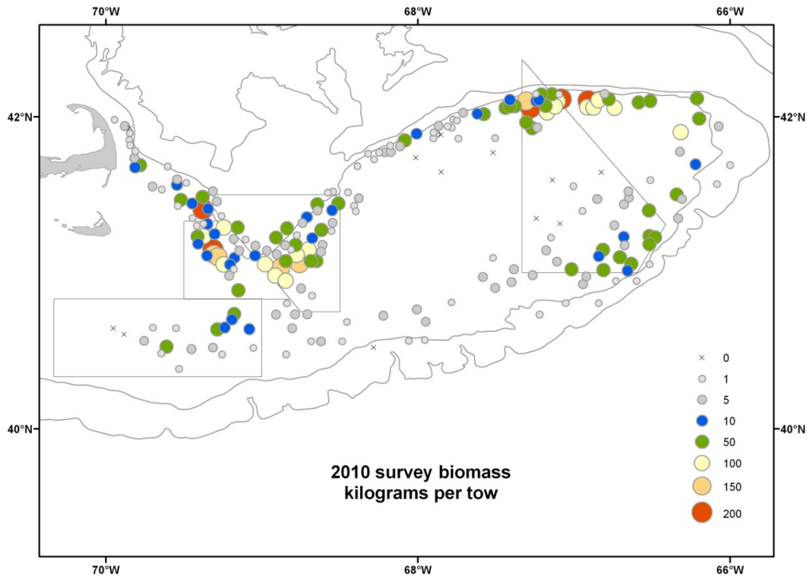
Figure 10 - Biomass chart for Georges Bank from the 2010 NMFS sea scallop survey
