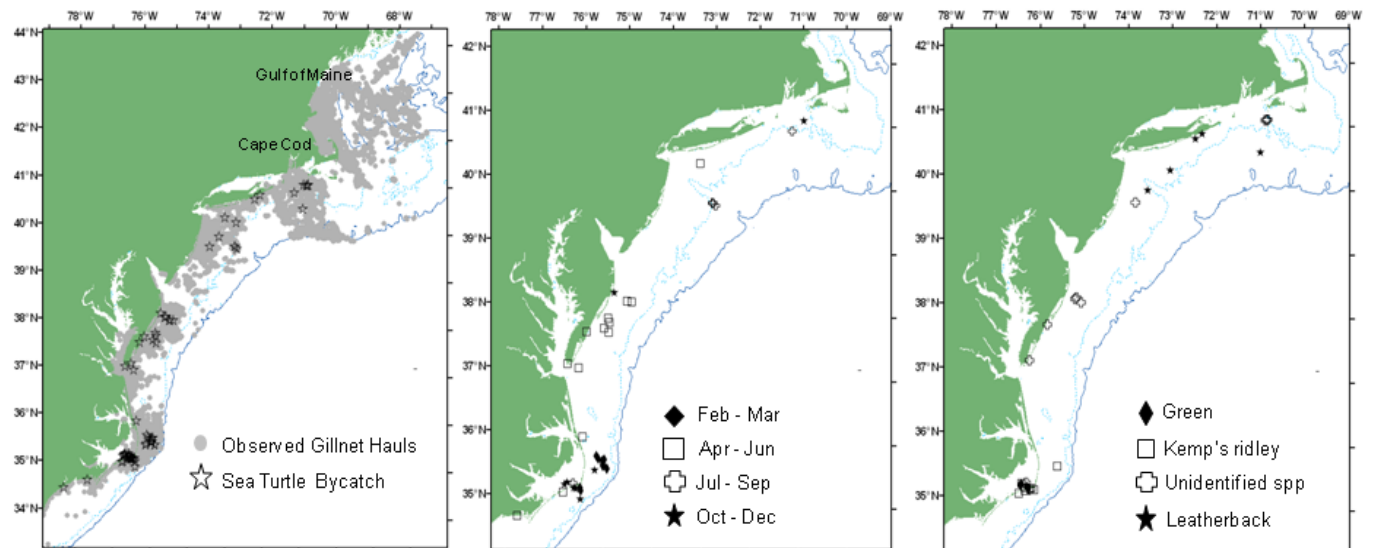
Figure 23 - Locations of observed sink gillnet hauls, 1995-2006. a) Observed hauls and turtle bycatch, b) Observed loggerhead bycatch, c) Observed green, Kemp's ridley, unidentified, and leatherback species bycatch. The 50m and 200m bathymetry lines are also shown. From Murray (2009).
