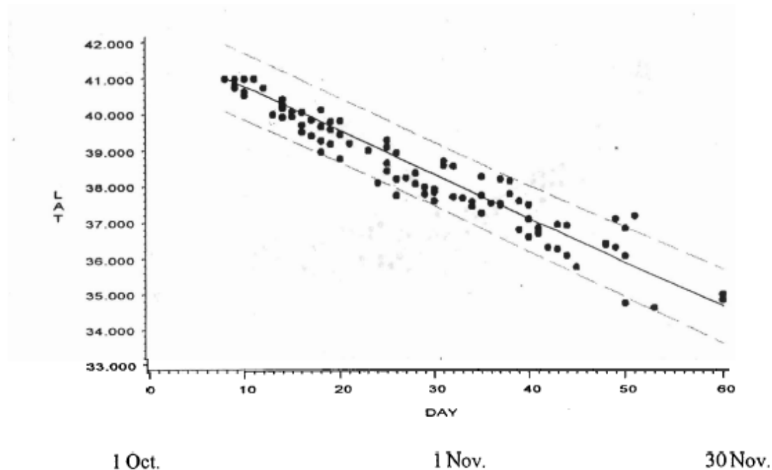
Figure 19 – Relationship between day and latitude of turtles during migration (Morreale, 1999)
