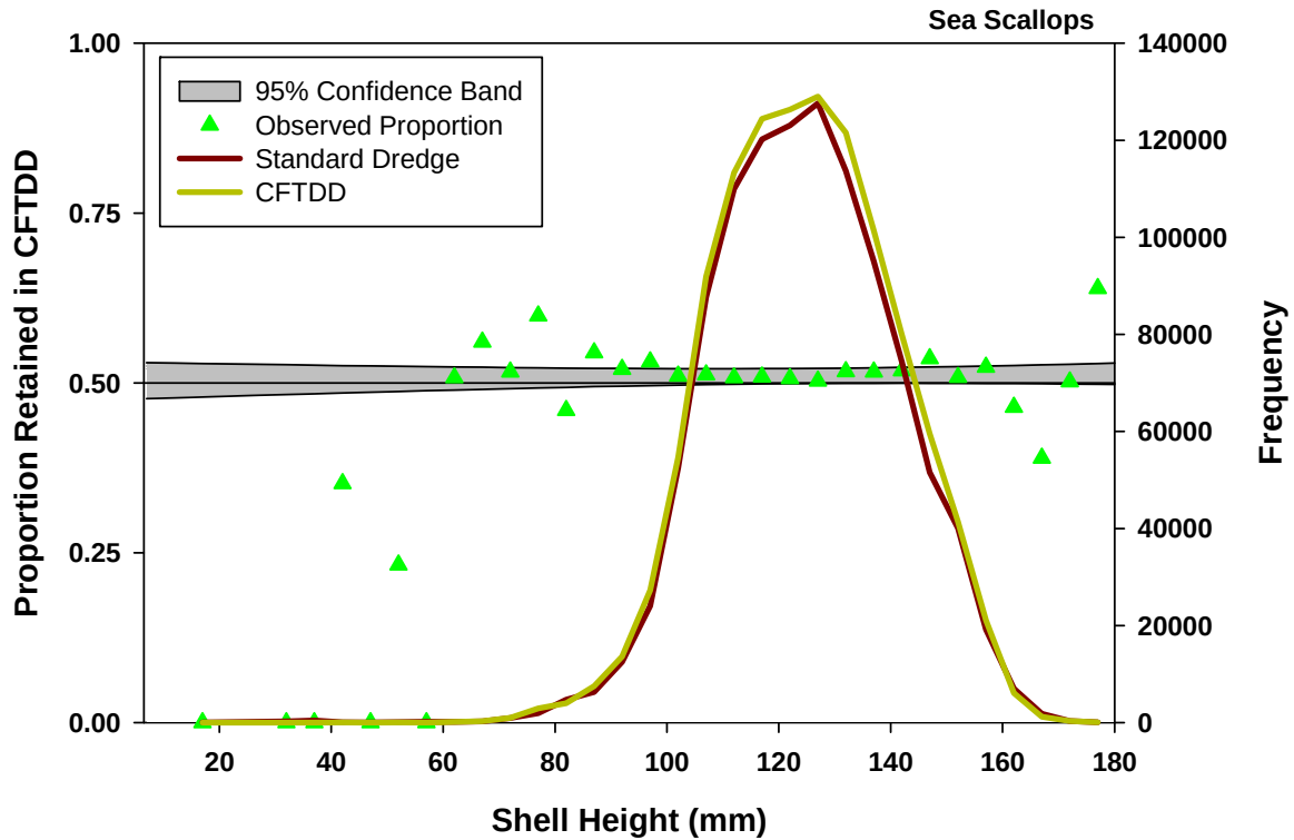
Figure 31 - Observed scaled length frequency distributions for the TDD and the New Bedford style scallop dredge. The green triangles represent the observed proportions ( \text{Catch}_{\text{CFTDD}} / (\text{Catch}_{\text{STAND}} + \text{Catch}_{\text{CFTDD}}) ). The grey shaded area represents the 95% confidence band around the estimated relative efficiency values as estimated by the two parameter (gear and length effect model).
