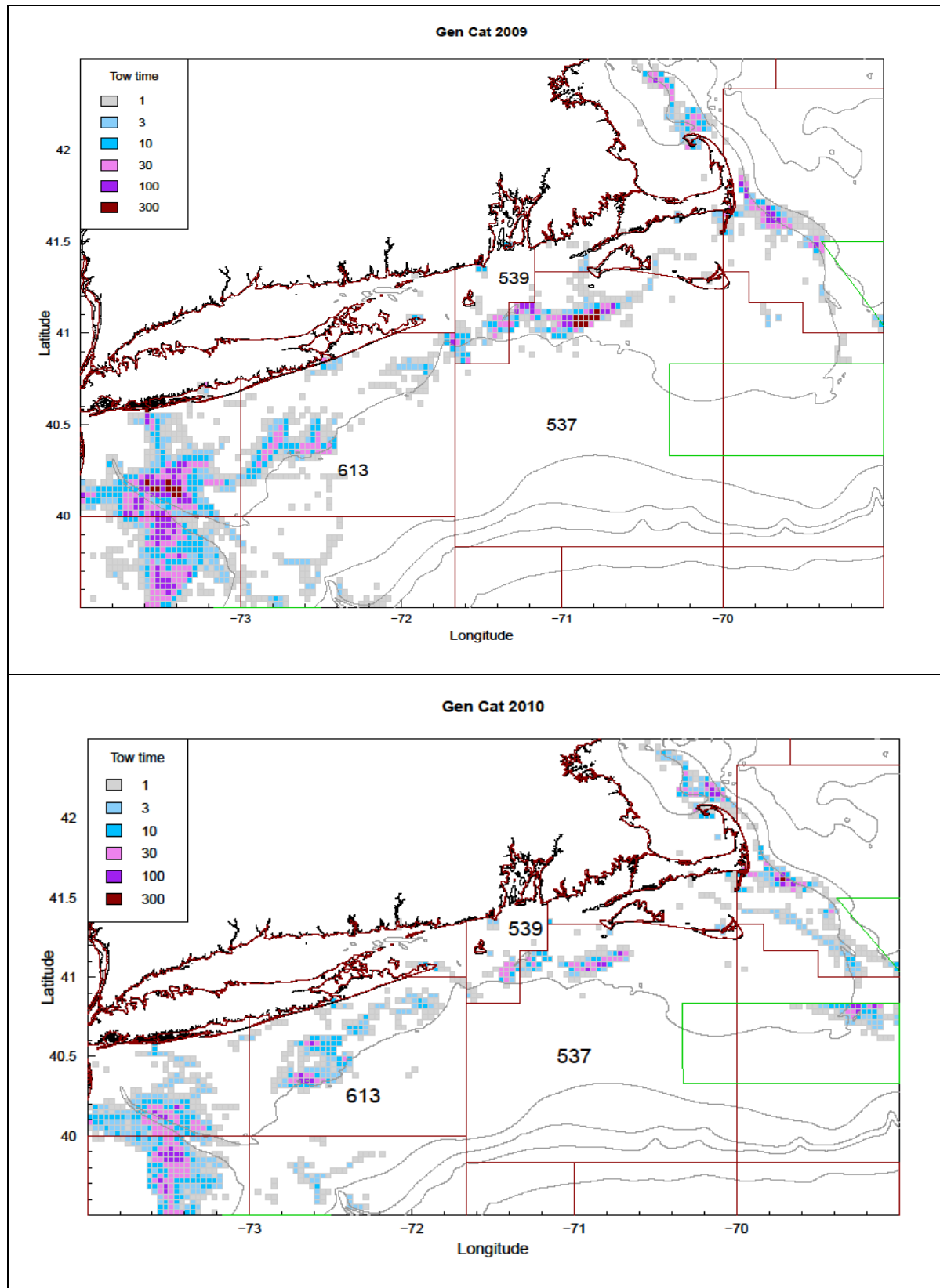
Figure 9 – VMS data for the LAGC fishery in FY2009 and FY2010 with YT AM area identified (statistical areas 537, 539, and 613)
