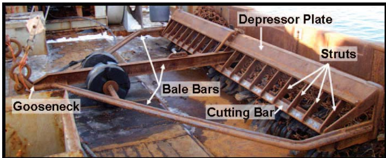
Figure 3 – Turtle deflector dredge with primary elements of gear modifications identified (Source: Smolowitz et al, 2010)
