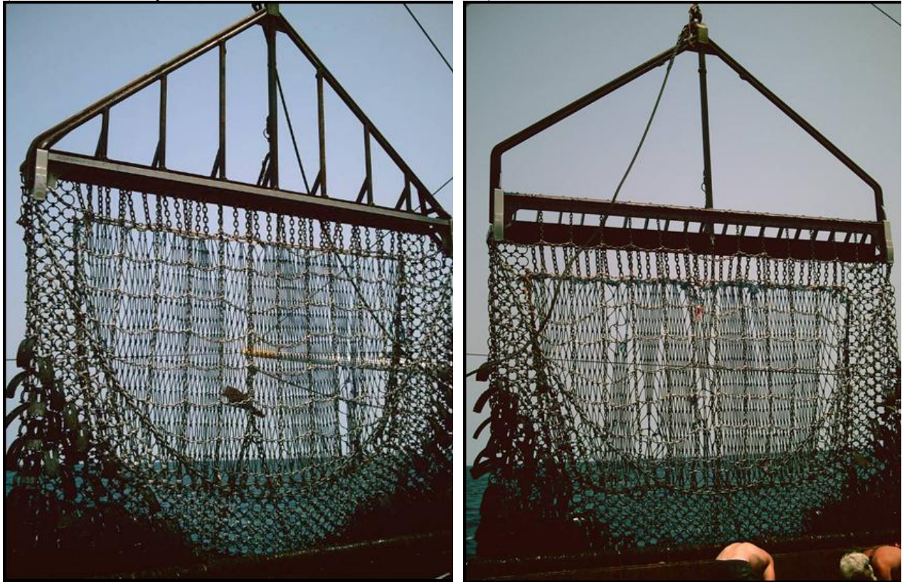
Figure 2 – Comparison of standard commercial scallop dredge (left) and turtle deflector dredge (right) (Photos: Courtesy of Coonamessett Farm Foundation)
