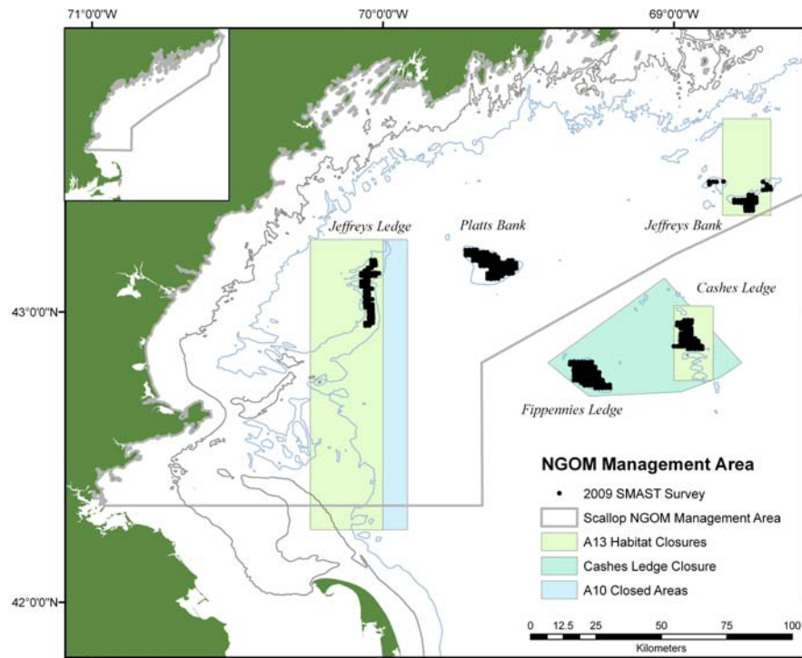
Figure 34 – Location of SMAST survey stations in the NGOM in 2009 and 2010
