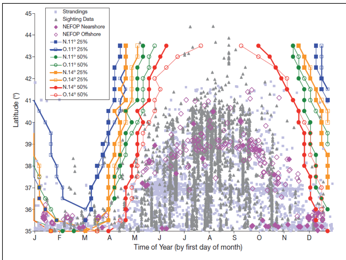
Figure 16 – Loggerhead, Kemp's ridley, green and hawksbill strandings -1998-2004 (Braun-McNeill et al 2008)
