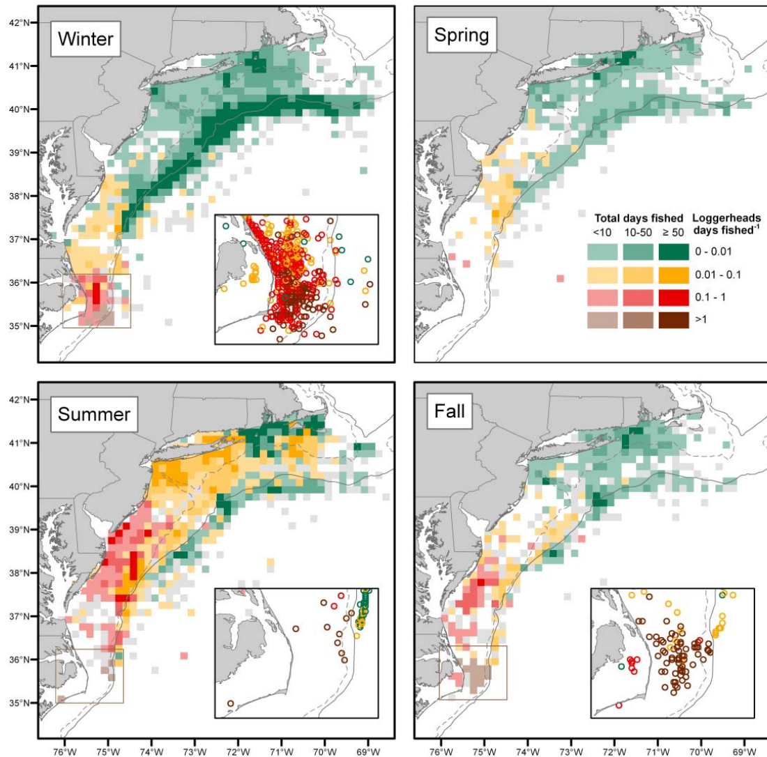
Figure 22 - Mid-Atlantic bottom trawl fisheries for fish and scallops, 2005–2008: predicted observable loggerhead interaction rates aggregated by 10' squares. The highest interaction rates were predicted in the fall (1 Nov–30 Nov; maximum rate = 4.6 loggerheads day fished -1 ), followed by summer (16 May–31 Oct; 3.3), winter (1 Dec–15 Apr; 1.5), and spring (16 Apr–15 May; 0.68). From: Warden (in press).
