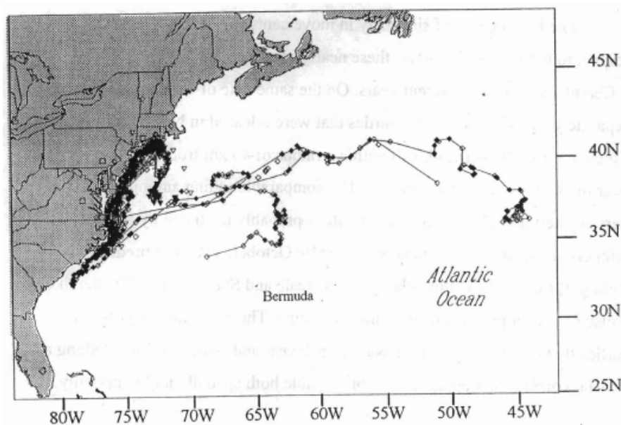
Figure 4.1. The similar migration paths of 15 juvenile sea turtles tracked by satellite transmitter from New York waters beginning in the summer or fall of five different years. Three Kemp's ridleys in 1990 and 1991, along with 4 loggerheads in 1992 were tracked in previous studies (Morreale and Standora 1994); eight more loggerheads were tracked in the present study in 1995 and 1996. Turtles remained in near shore waters, until fall, when they migrated out to sea and southward along coastal shelf waters by early winter. Some overwintered in the Carolinas and others moved into pelagic waters in late winter, traveling with the Gulf Stream to positions thousands of kilometers offshore.
