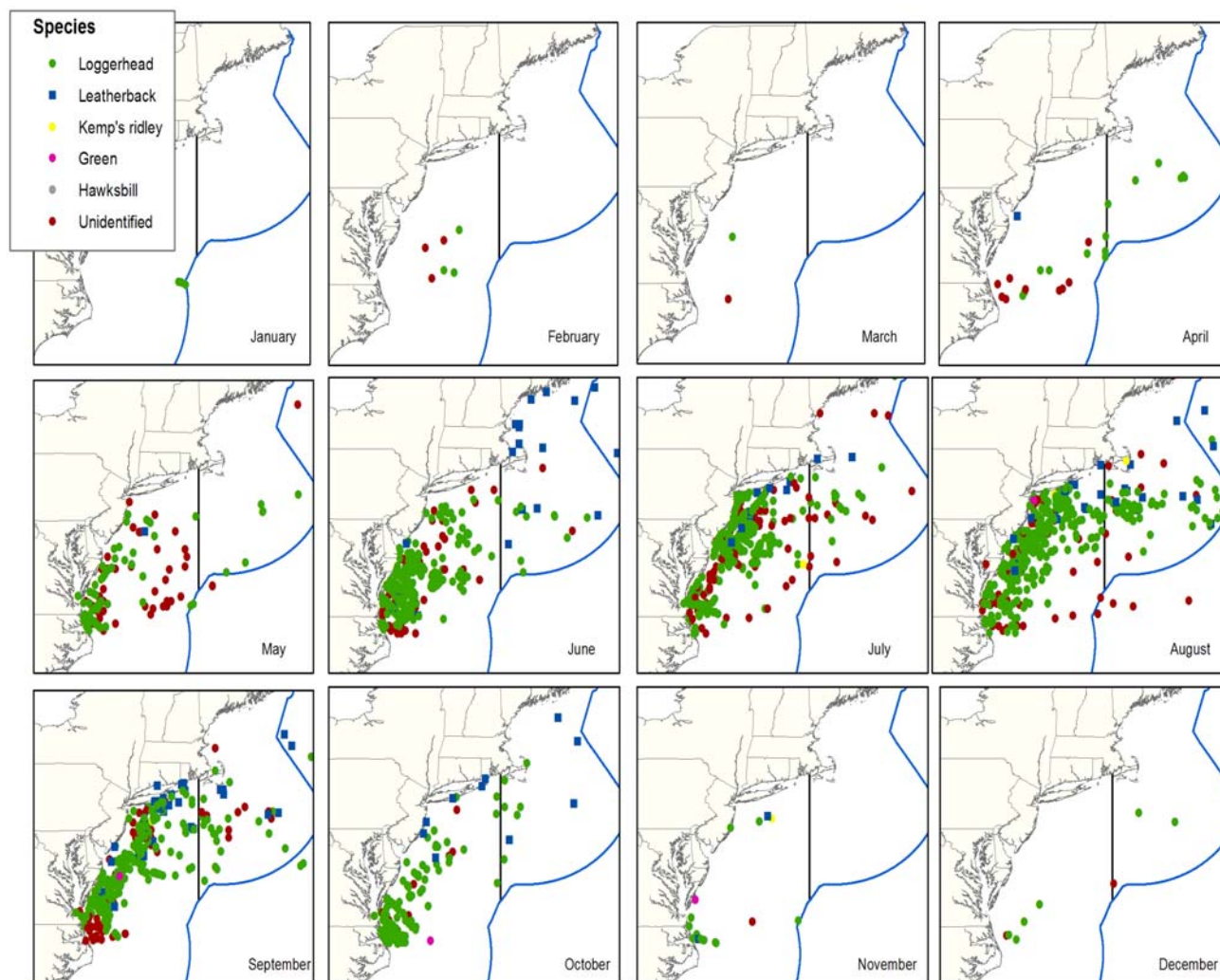
Figure 20 – Sea turtle sightings by month (CETAP aerial and shipboard surveys from 1978-1982)
