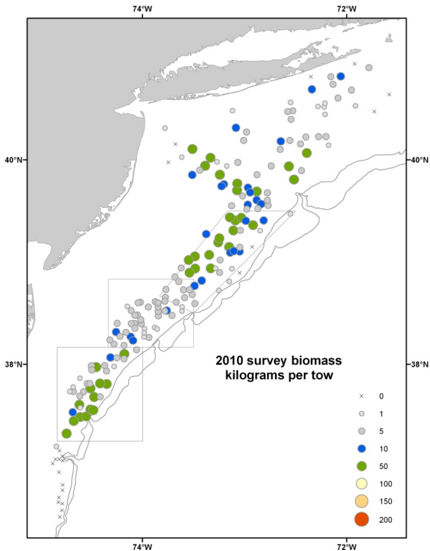
Figure 11. Biomass chart for the Mid-Atlantic from the 2010 NMFS sea scallop survey
