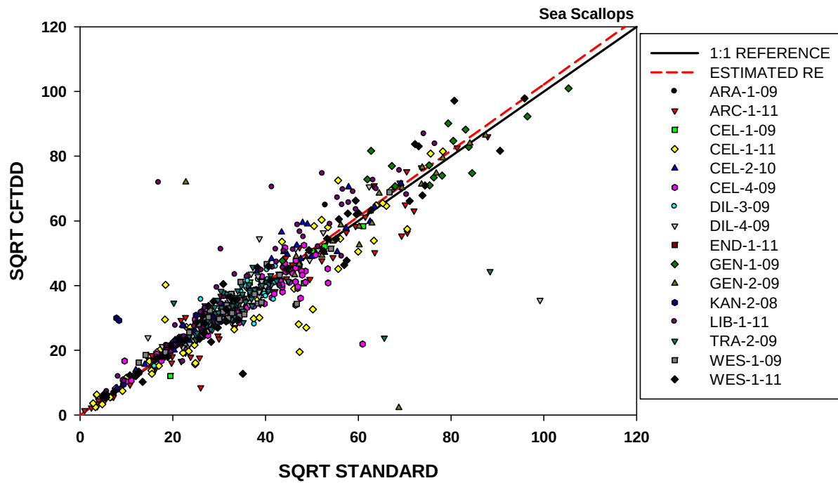
Figure 30 - Total scaled pooled scallop catches for TDD vs. the standard New Bedford style scallop dredge (top panel) The black line has a slope of one. The dashed line has a slope equal to the estimated relative efficiency (from the one parameter gear effect only model).
