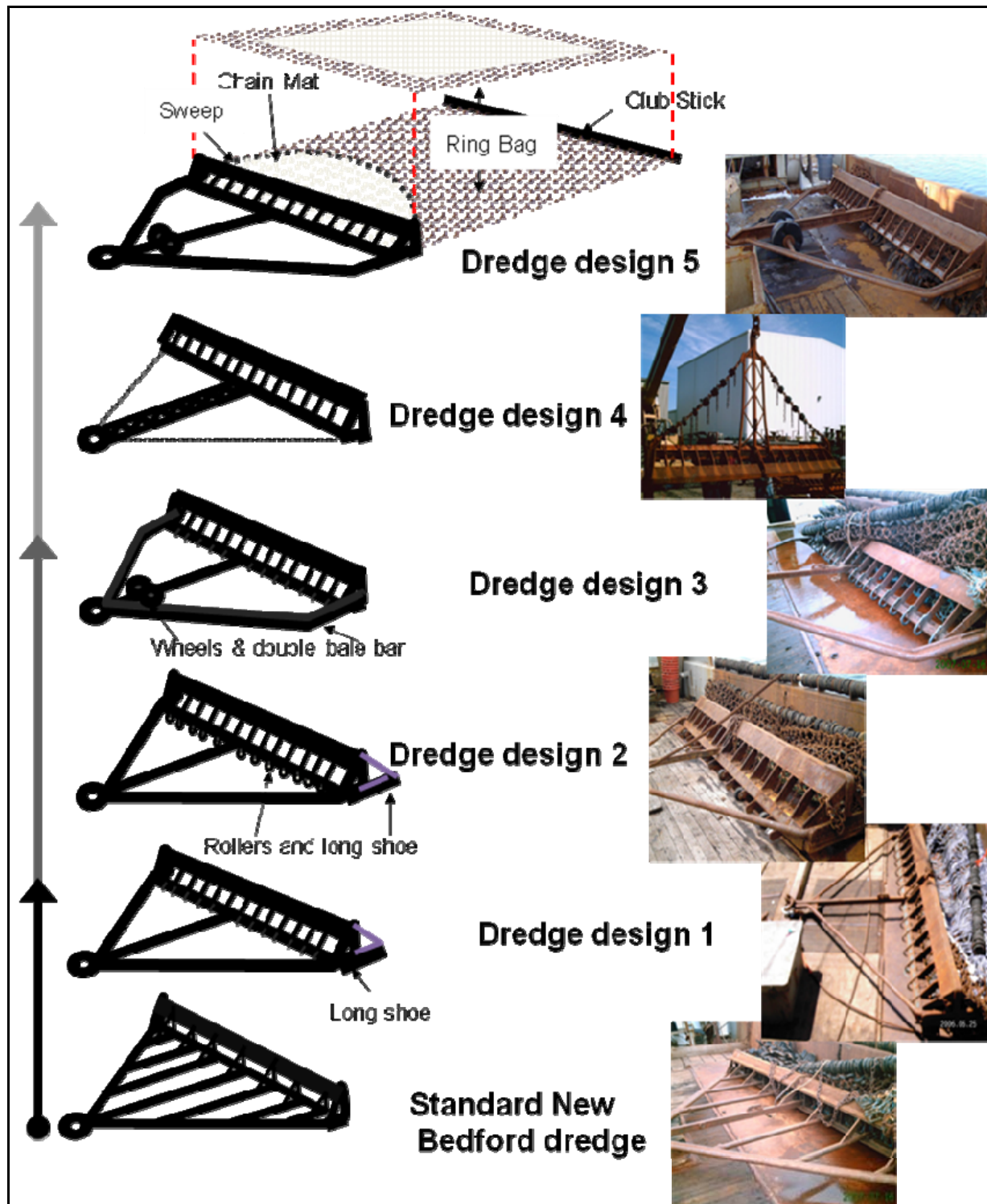
Figure 1 – Evolution of the standard New Bedford commercial scallop dredge to the turtle deflector dredge (Source: Smolowitz et al, 2010)
