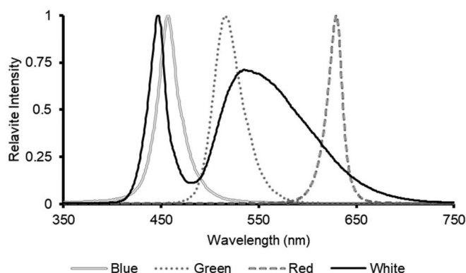
Fig. 2. Normalized spectral distribution of the LED outputs from the lights used in this study, indicating the wavelength of peak output ( \lambda_{\max} ) for the blue, green, and red LEDs was 460, 515, and 630 nm, respectively. The white LED was bimodal, with \lambda_{\max} at 445 nm and a secondary peak at 535 nm.
