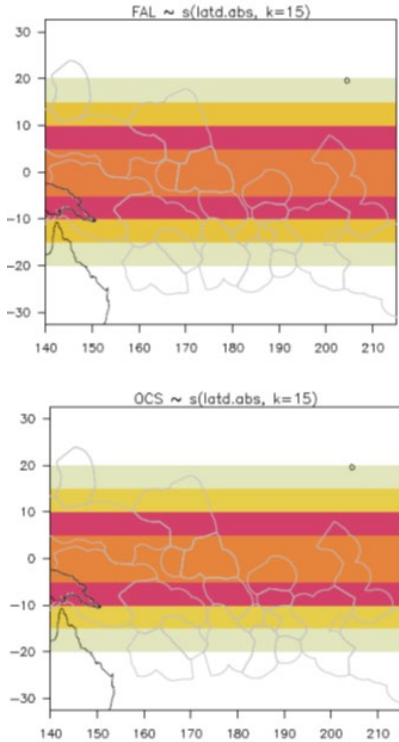
Figure 3. Predicted relative abundance surfaces for silky shark (FAL; top) and oceanic whitetip shark (OCS;bottom) for the absolute value of latitude model.
