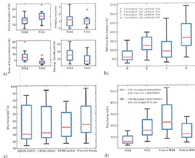
Figure 3. Results: a) Changes in the HEC-HMS parameters, b) Individual contribution of the increased precipitation and urbanization c) Comparison with other studies, and d) Sensitivity of future scenarios to the changes in precipitation and urbanization. Note: each box-and-whisker plot is based on all 12 watersheds in the study.
