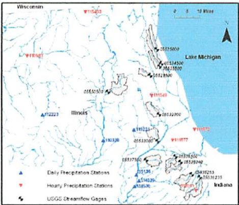
Figure 2. Streamgages, basins and precipitation stations used in rainfall-runoff modeling
