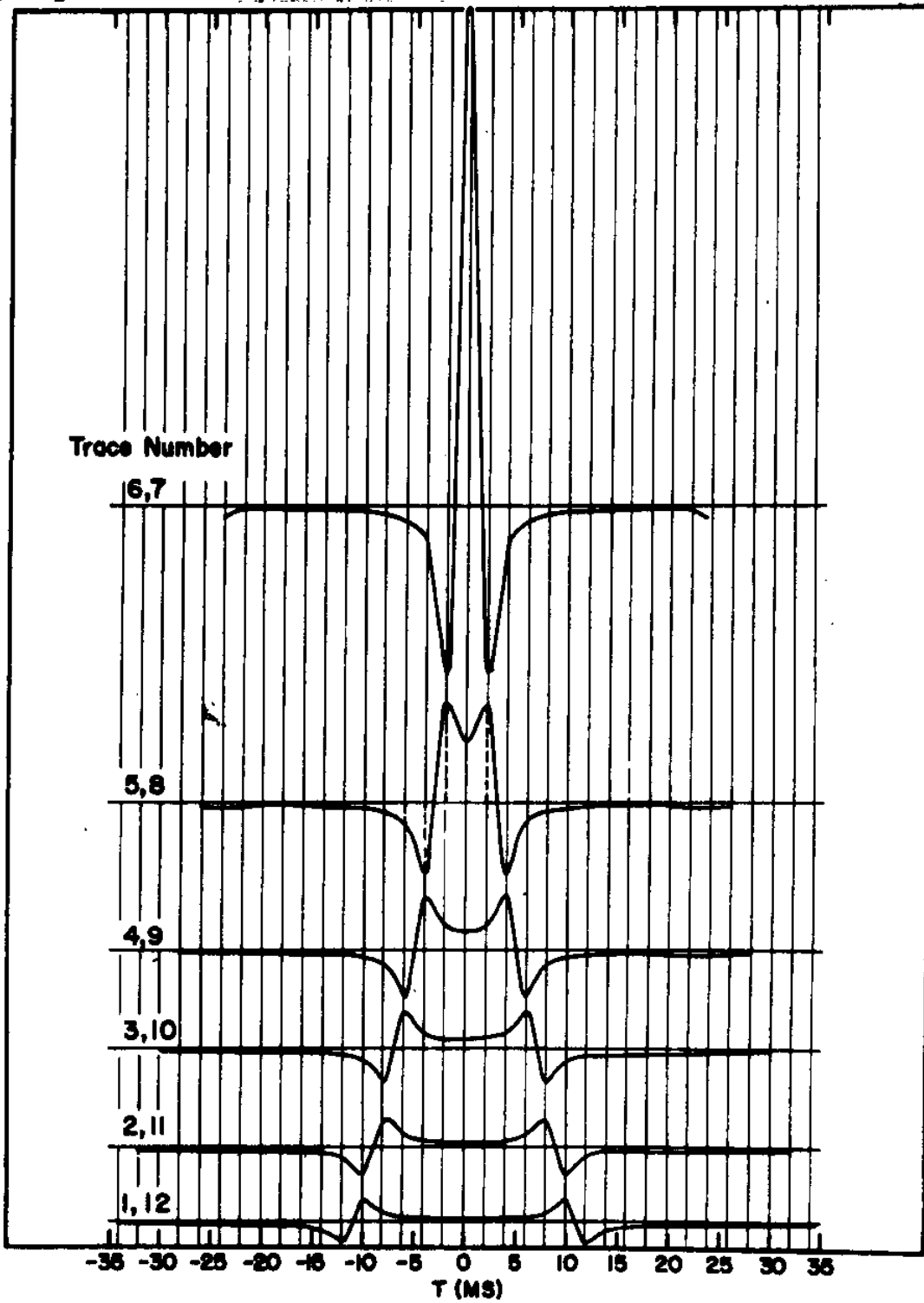
Figure 4. Impulse Response at y=0 for a 12 Trace, +0.5 Trace/ms Wideband Velocity Filter. (From Embree, et.al. 5 )
