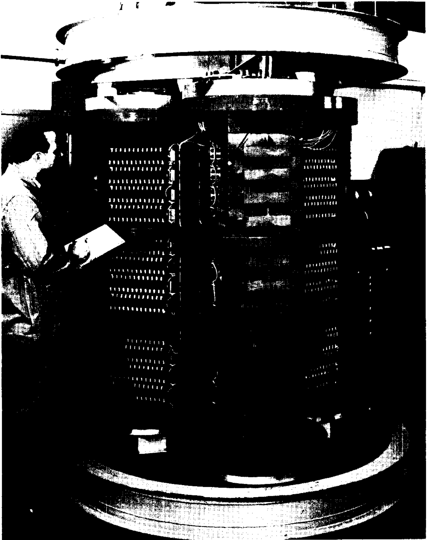
Figure 23. Bender Array (Honeywell)
