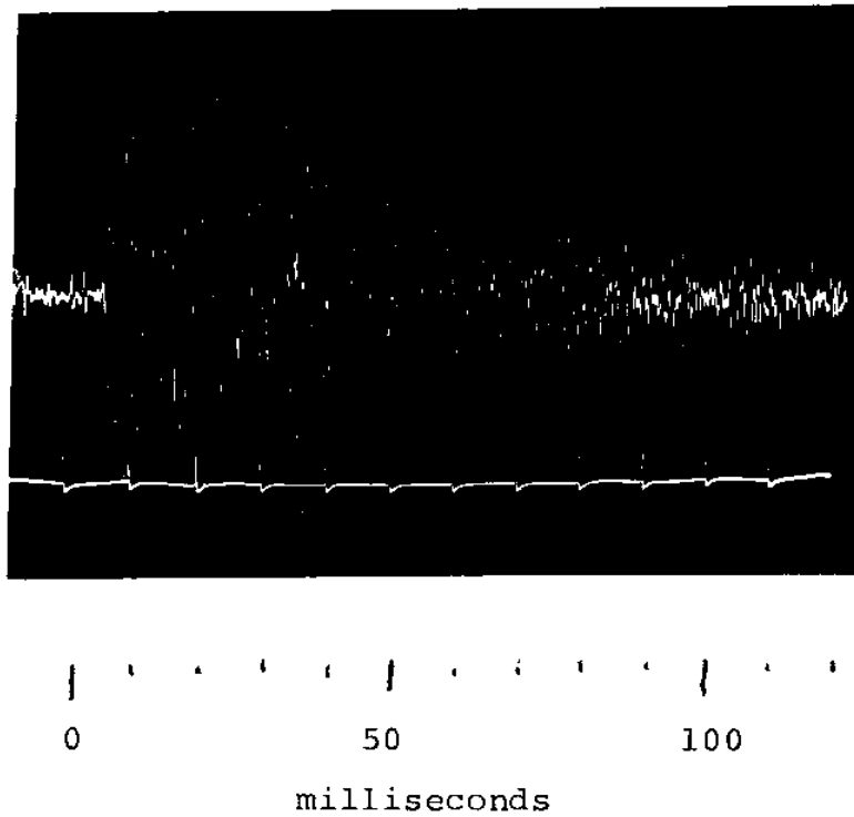
Submarine echo recorded 500-5000 Hz
