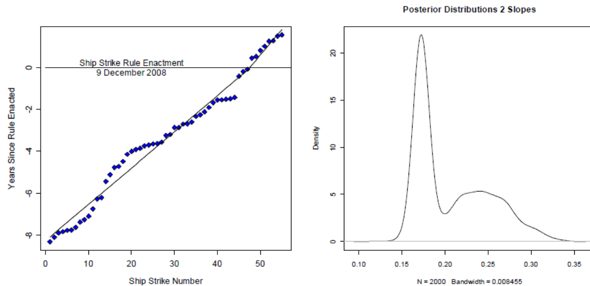
Figure 3. Whale and ship collisions resulting in serious injuries or mortalities detected along the US Eastern seaboard 2000-2010. Graphs depict Bayesian model fit of rate of events that included a change point fixed at Ship Strike Rule enactment date estimated for the timing of events in chronological order (A) and the posterior distributions of estimated of rates (1/years between events) for change point model (model 5 above).
