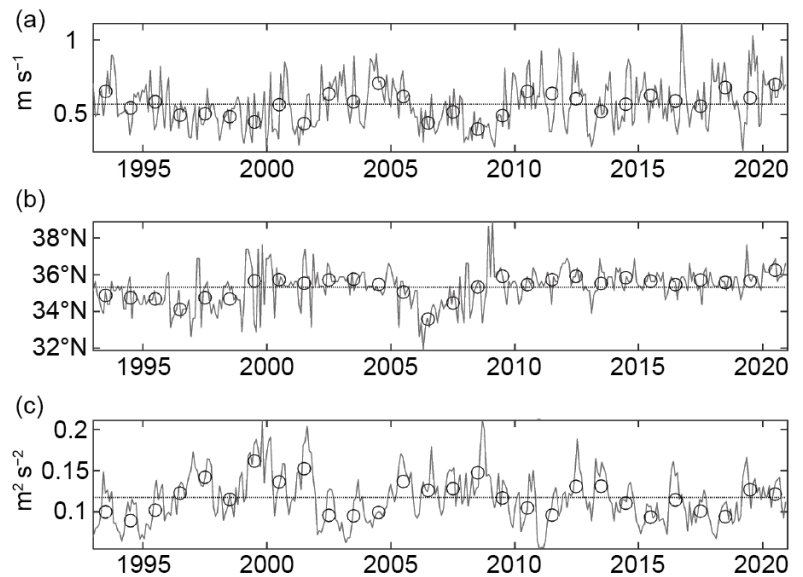
Fig. 3.20. (a) Maximum zonally averaged value of total geostrophic zonal velocity ( U ; \text{m s}^{-1} ) versus time in the Kuroshio Extension region ( 141^\circ – 153^\circ\text{E} , 32^\circ – 38^\circ\text{N} ; Qiu and Chen 2005). (b) Latitude ( ^\circ\text{N} ) of the maximum velocity shown in (a). (c) Eddy kinetic energy (EKE; \text{m}^2 \text{s}^{-2} ) averaged in the Kuroshio Extension region. In all plots, monthly values are shown in gray, annual averages as black circles, and the time-mean is shown as a horizontal gray line.
