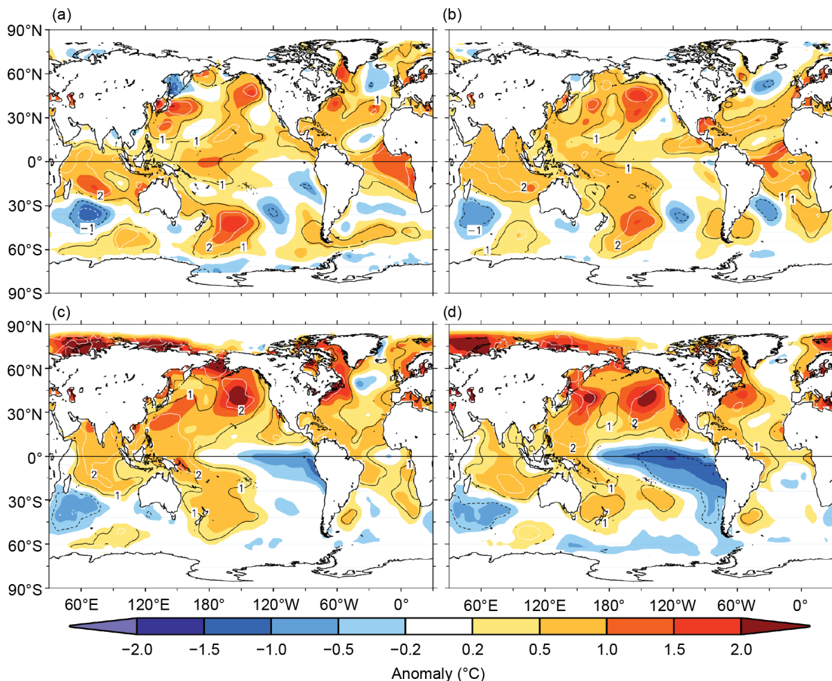
Fig. 3.2. Seasonally averaged SSTAs of ERSSTv5 ( ^{\circ}\text{C} ; shading) for (a) DJF 2019/20, (b) MAM 2020, (c) JJA 2020, and (d) SON 2020. Normalized seasonal mean SSTa based on seasonal mean std. dev. over 1981–2010 are contoured at values of -2 (dashed white), -1 (dashed black), 1 (solid black), and 2 (solid white).
