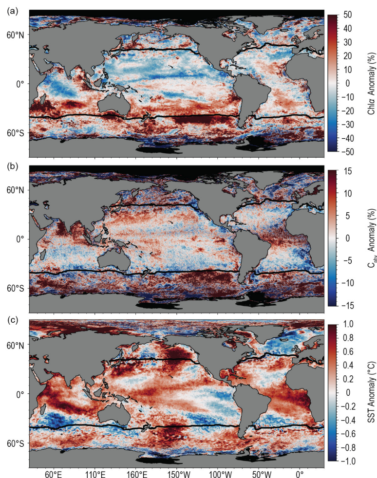
Fig. 3.24. Spatial distribution of average monthly (a) MODIS-A Chla anomalies, (b) MODIS-A C_{\text{phy}} anomalies, and (c) MODIS-A SST anomalies, where monthly differences were derived relative to a MODIS-A 17-year climatological record (Oct 2002–Sep 2019). Chla and C_{\text{phy}} are stated as % difference from climatology, while SST is shown as an absolute difference. Also shown in each panel is the location of the mean 15°C SST isotherm (black lines) delineating the permanently stratified ocean (PSO). Differences in the SST anomalies here versus in Fig. 3.1a are owing to differences in climatological periods, smoothing, and data sources.
