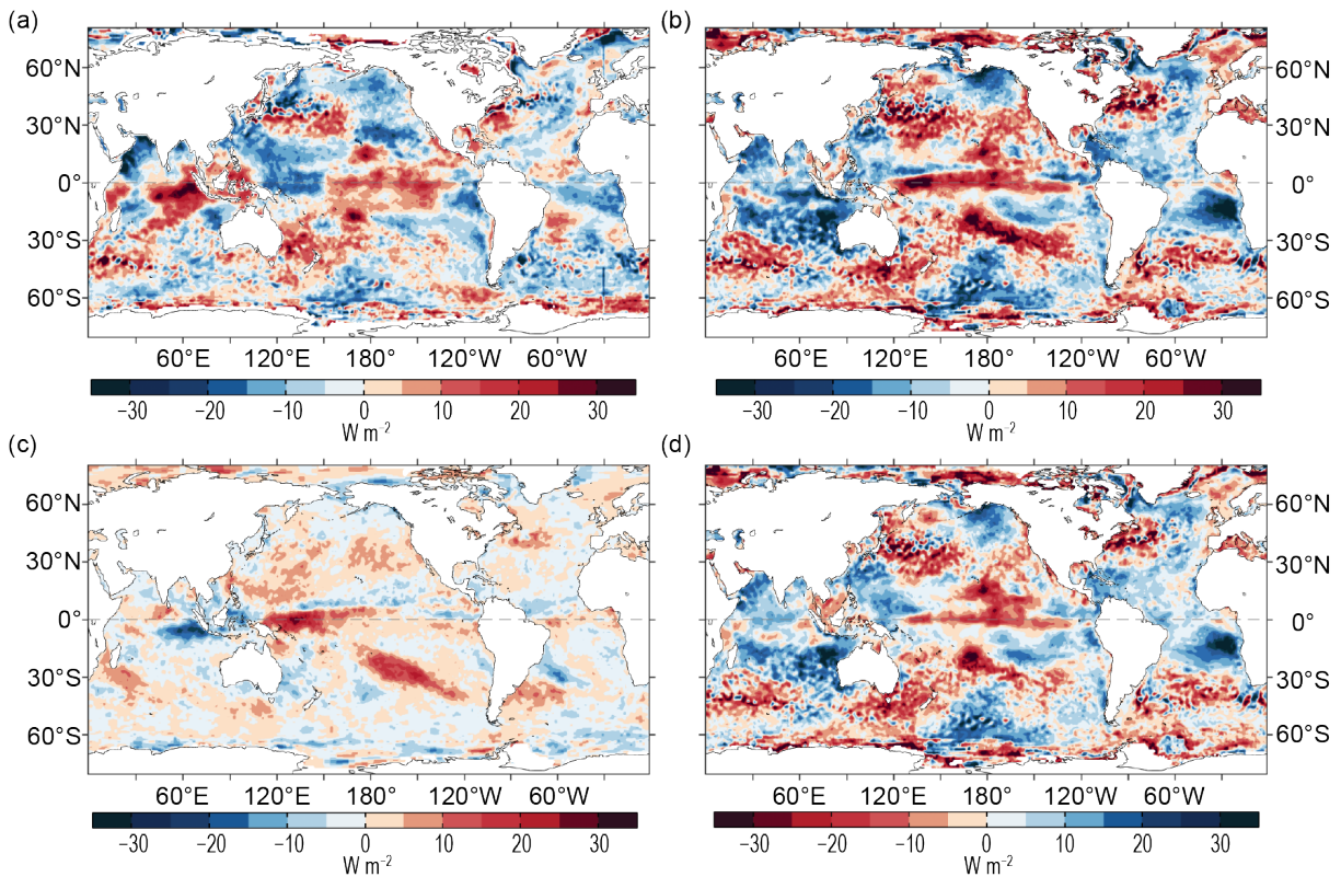
Fig. 3.11. (a) Surface heat flux ( Q_{\text{net}} ) anomalies for 2020 relative to the 2001–15 climatology. Positive values denote ocean heat gain. (b) 2020 minus 2019 difference for Q_{\text{net}} , (c) surface radiation (SW+LW), and (d) turbulent heat fluxes (LH+SH), respectively. Positive changes denote more ocean heat gain in 2020 than in 2019, consistent with the reversal of the color scheme in (d). All units are given in \text{W m}^{-2} . LH+SH are from OAFlux, and SW+LW is the NASA FLASHFlux version 4A.
