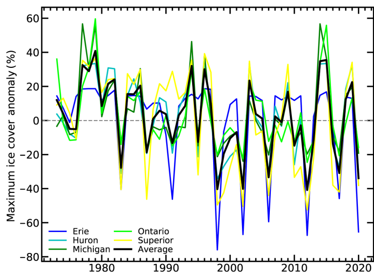
Fig. 2.18. Anomalies in Great Lakes maximum ice cover extent (%) for 1973–2020 (base period is 1981–2010). The black line shows the average anomaly for all of the Great Lakes, whereas the other lines show individual lakes (Erie, Michigan, Superior, Ontario, Huron).
