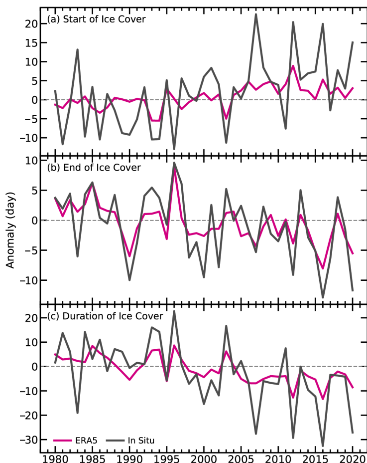
Fig. 2.17. (a) Lake ice on, (b) ice off, and (c) ice duration anomalies from 1980 to 2020 derived from in situ observations and ERA5. Base period is 1981–2010. In situ observations of ice on, ice off, and ice duration are derived from nine lakes monitored in Finland, one lake in Russia, nine lakes in the United States, and one lake in Canada.
