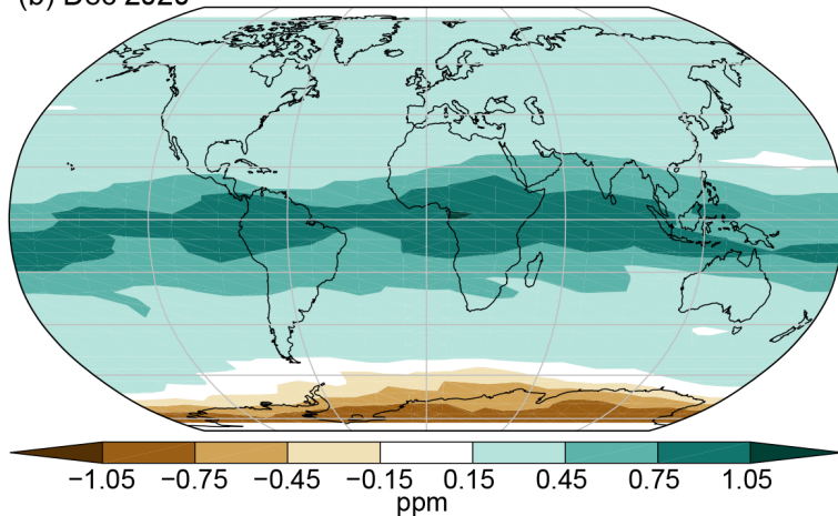
Fig. 2.62. Deseasonalized monthly lower stratospheric Microwave Limb Sounder (MLS) anomalies (ppm; 2004–20 base period) centered on 82 hPa in (a) Dec 2019 and (b) Dec 2020 from the Aura MLS.
