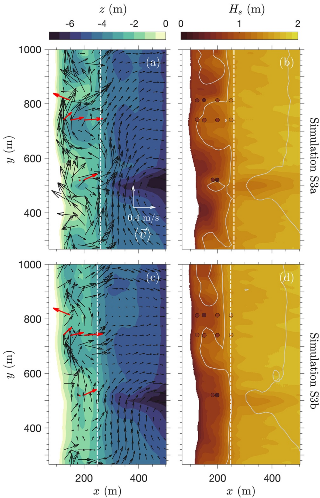
Figure 5. Observed (left: red arrows, right: filled circles) and modeled (left: black arrows, right: color contours) (a and c) hour-averaged depth-averaged velocity, \langle \vec{v} \rangle and (b and d) significant wave height, H_s for moderate-energy shore-normal wave conditions on October 28 with (a and b) October 14 (S3a) and (c and d) November 16 (S3b) bathymetry. Bathymetry (left: color contours, right: gray contour curves at 2.5 and 5.0 m depth) and the approximate outer edge of the surf zone ( x_{sz} , all panels: dashed-white lines) are shown. The \langle \vec{v} \rangle scale (left) and H_s colorbar (right) span approximately twice the range of those in Figure 4.
