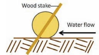
Figure 23: Proper staking of bioroll
