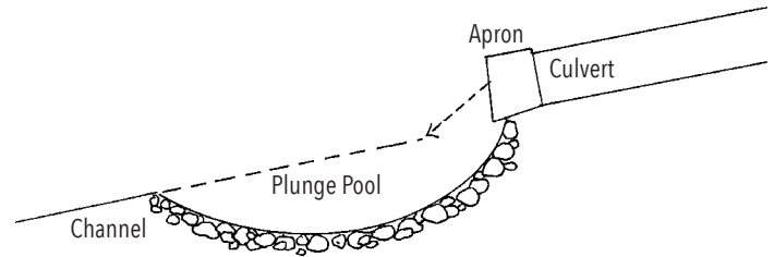
Figure 29: Side view of plunge pool riprap installation
