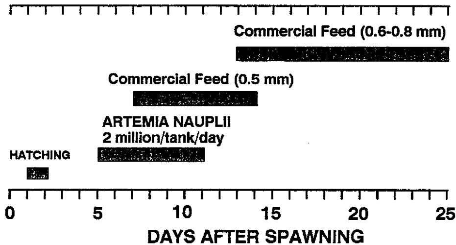
Figure 13. Schematic diagram of the feeding regimen used for the larval culture of tiger barbs.
