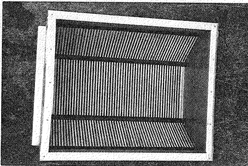
Figure 15. Photograph of bar grader used to sort tiger barbs by size.
