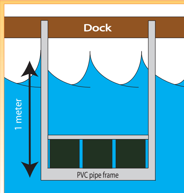
FIGURE 4. Experimental frame design
