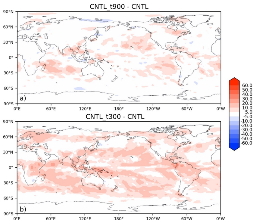
Figure 13. Differences of shortwave cloud radiative effect (SWCRE), relative to CNTL, for sensitivity experiments where the time step E3SM time step is adjusted to (a) 900 s and (b) 300 s. See Table 2 for simulation details.
