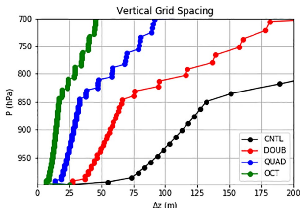
Figure 1. Estimated vertical grid spacing for the control (CNTL) simulation the various principle experiments described in Table 1 in the lower troposphere.
