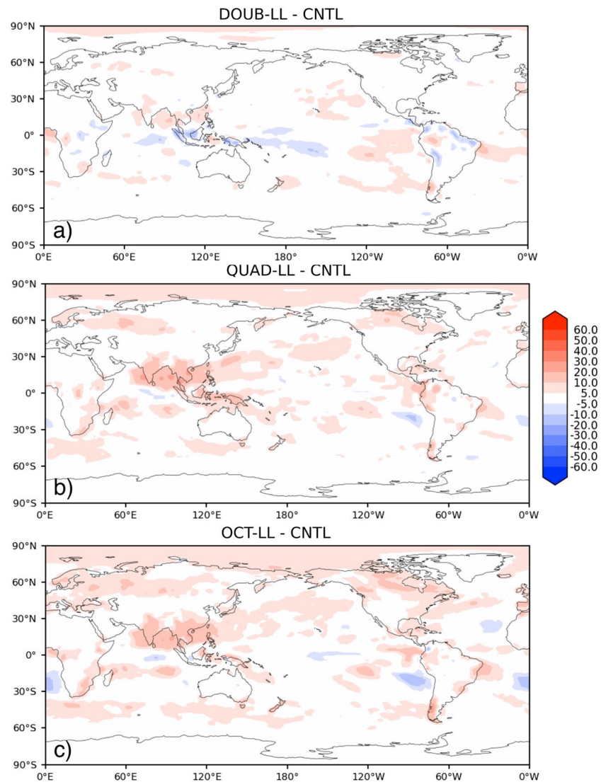
Figure 15. Evolution of the SWCRE biases relative to CNTL for vertical grid experiments where the lowest model level is refined for the (a) DOUB, (b) QUAD, and (c) OCT experiments. Results can be compared against those in Figure 6.
