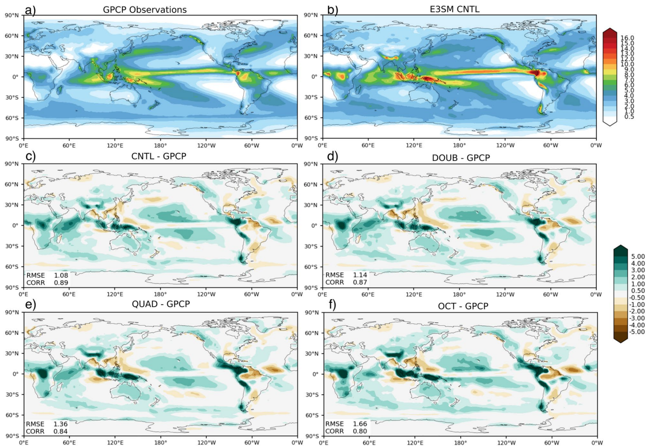
Figure 10. Same as Figure 2 but for surface precipitation rate. The Global Precipitation Climatology Project (GPCP) serves as the observational reference.
