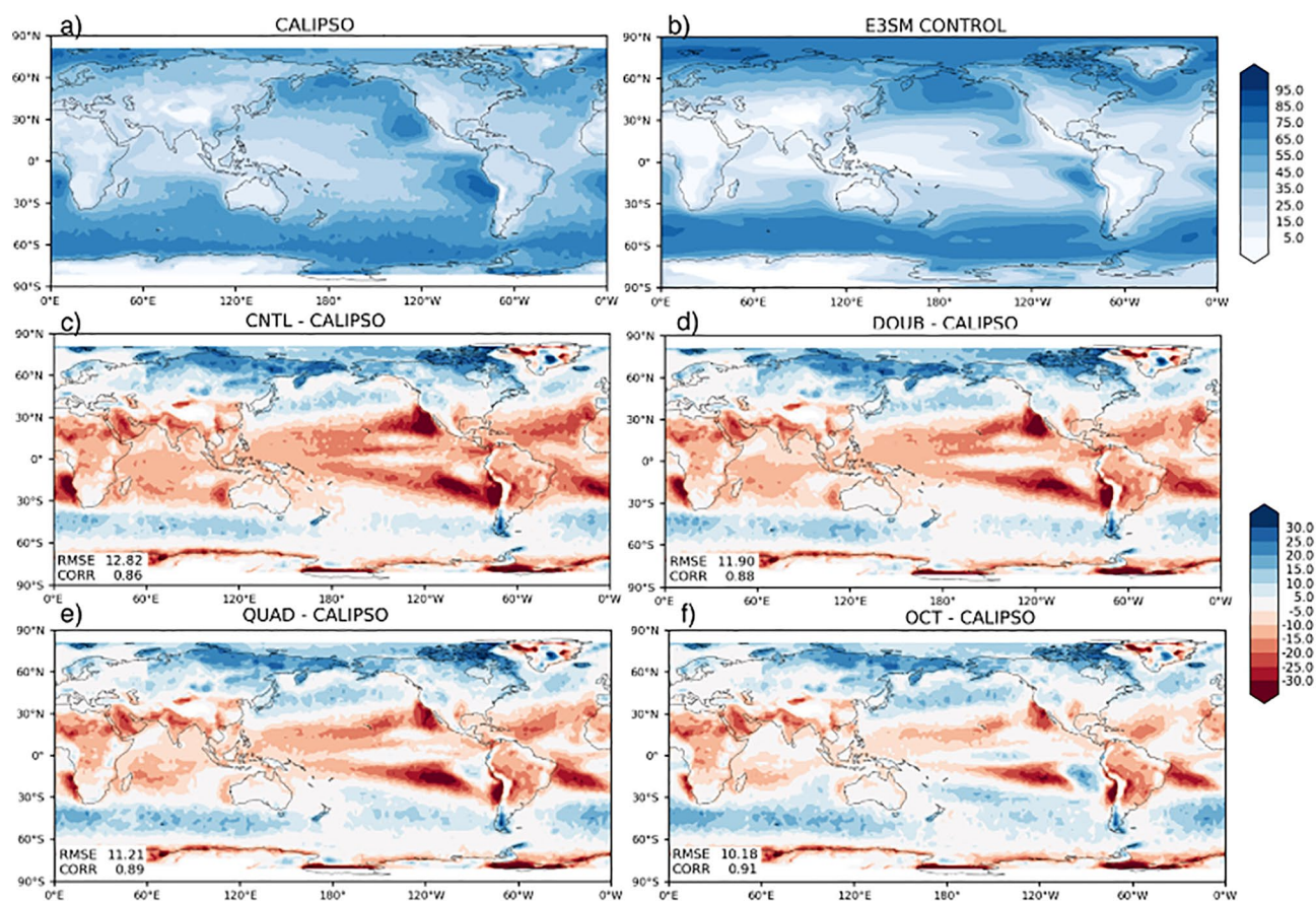
Figure 2. (a) Low cloud amounts from Cloud-Aerosol Lidar and Infrared Pathfinder Satellite Observation (CALIPSO) from January 2007 to January 2010 and (b) E3SM control simulation. (c)–(f) The biases for CNTL and the principle experiments, with the correlation coefficient and root mean squared error (RMSE) denoted for each simulation.
