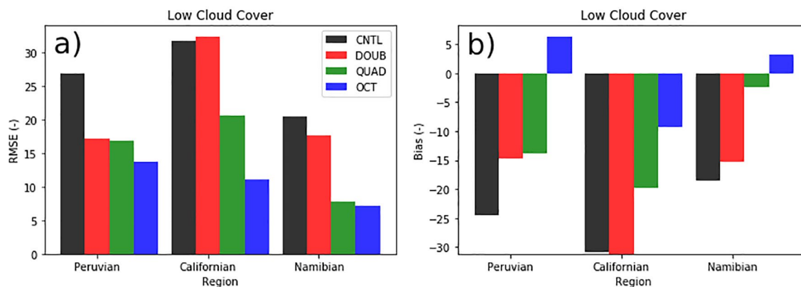
Figure 4. (a) Root mean squared error (RMSE) and (b) bias computed relative to CALIPSO observations for the low cloud amounts for three stratocumulus regions for each principle experiment. The California region is defined as the area bounded by 20°N to 30°N and 230°E to 240°E, the Peruvian region is defined as the area bounded by 20°S to 10°S and 260°E to 270°E, and the Namibian region is defined as the area bounded by 20°S to 10°S and 0°E to 10°E.
