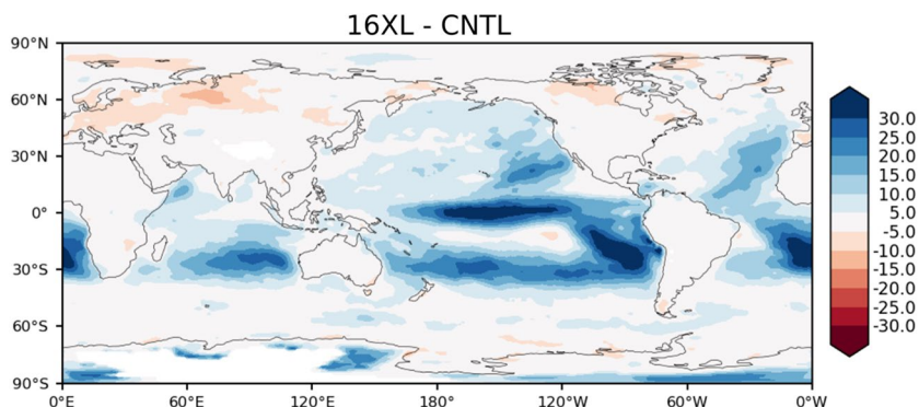
Figure 14. Low cloud amount difference relative to CNTL for the 16XL experiment simulation. See Table 3 for simulation details. Results can be compared against those in Figure 3.
