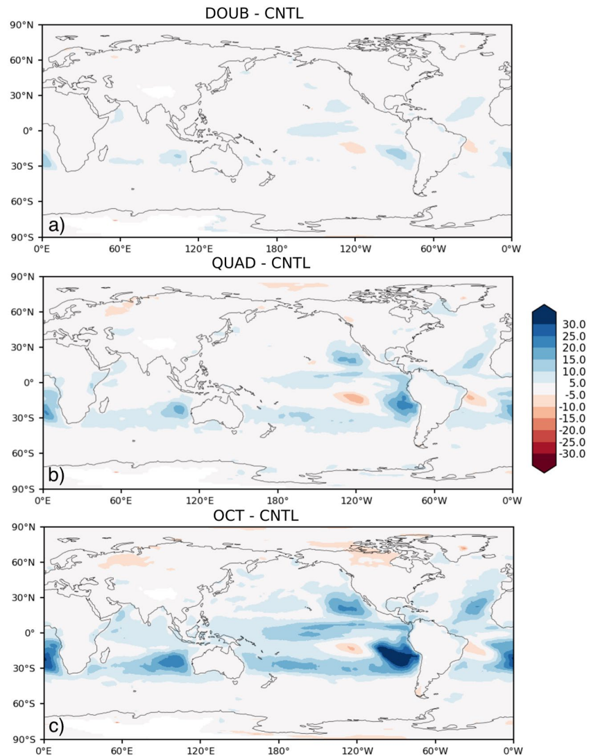
Figure 3. Low cloud amount differences computed relative to CNTL for (a) DOUB, (b) QUAD, and (c) OCT principle experiments.
