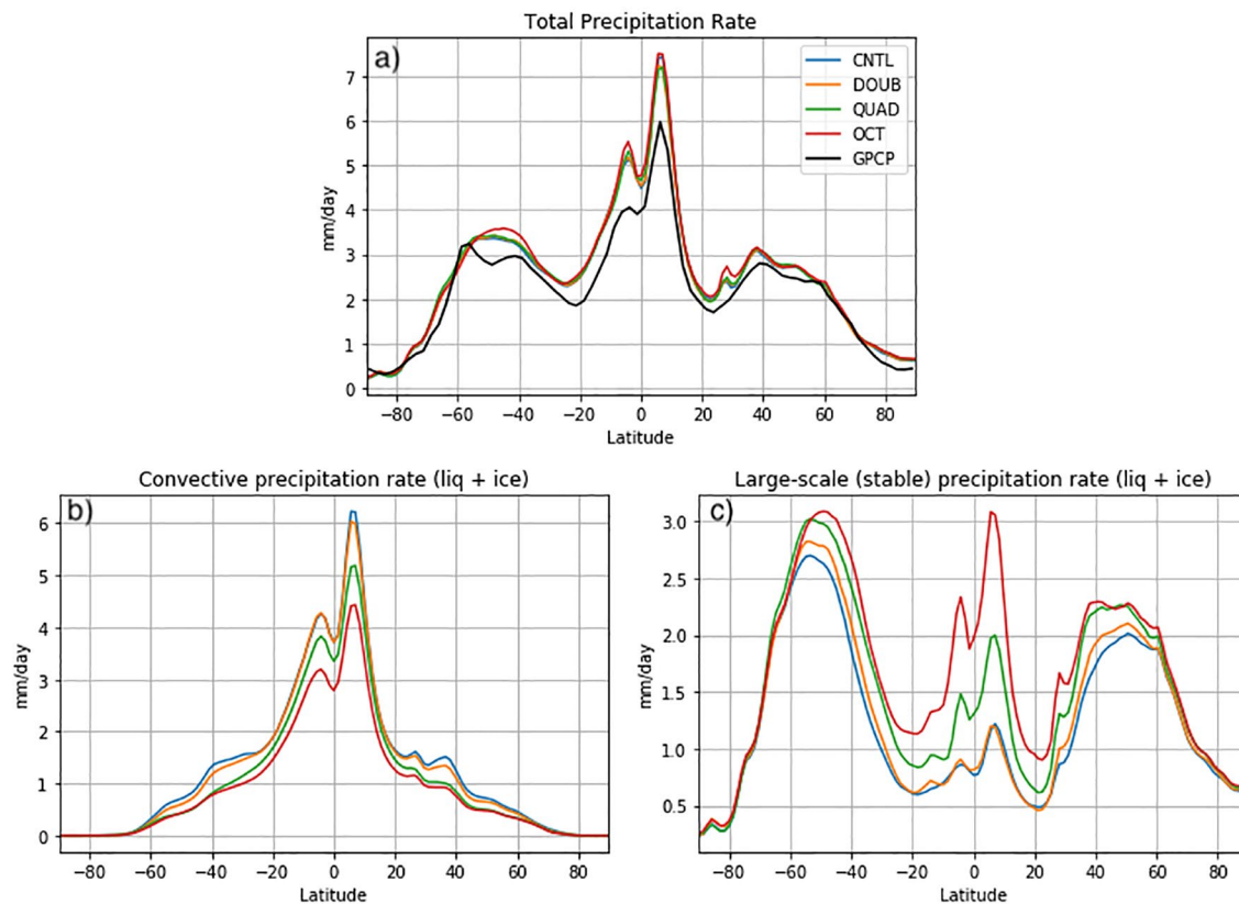
Figure 11. Zonally averaged (a) total surface precipitation rate, (b) contribution from convective precipitation, and (c) contribution from large-scale precipitation for CNTL and the principle vertical resolution experiments.
