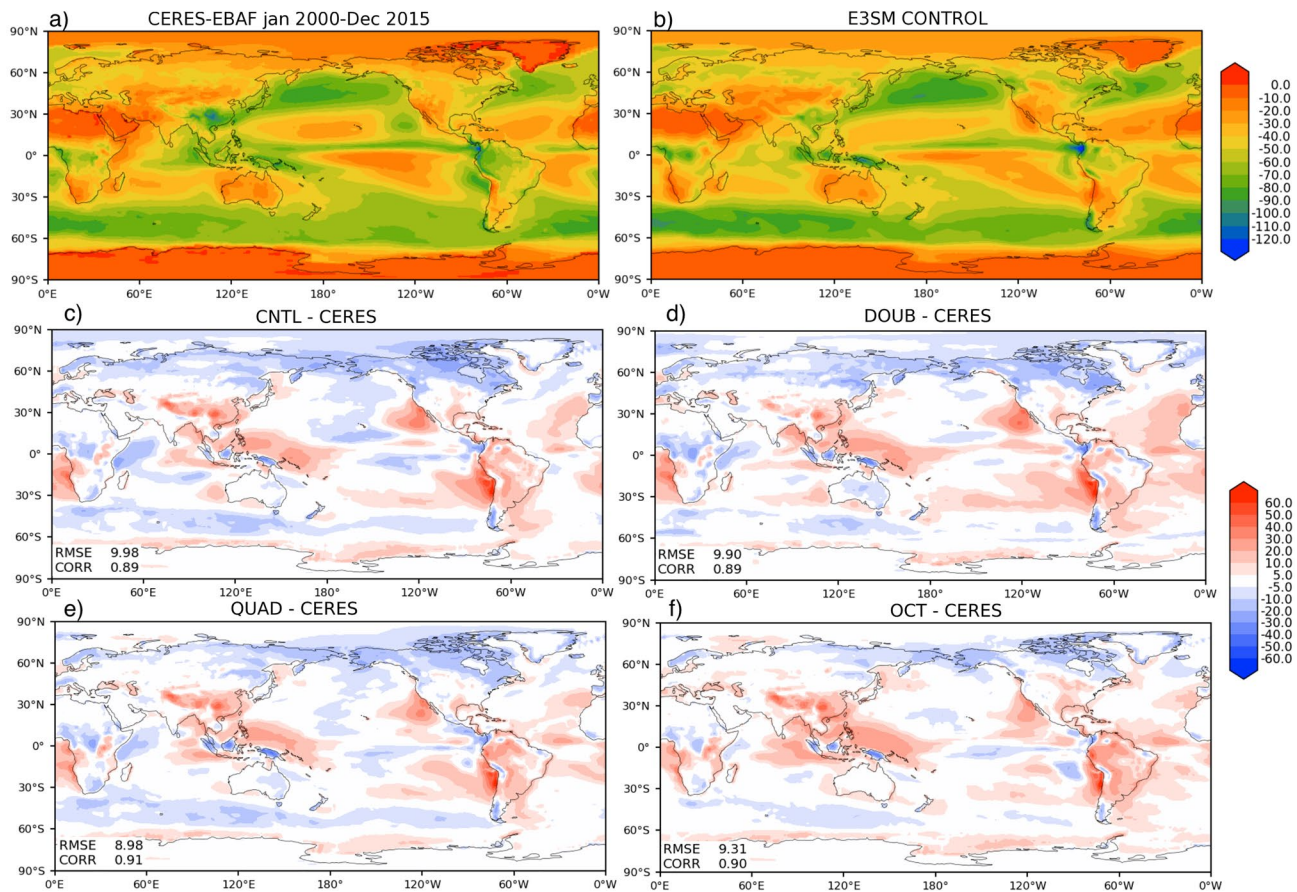
Figure 5. Same as Figure 2 but for shortwave cloud radiative effect (SWCRE). CERES-EBAF serves as the observational reference.
