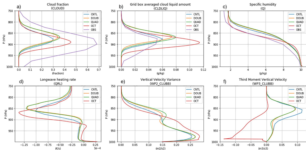
Figure 8. Temporally averaged profiles from September, October, and November for (a) cloud fraction, (b) cloud mixing ratio, (c) specific humidity, (d) longwave heating rate, (e) second moment of vertical velocity, and (f) third moment of vertical velocity for CNTL and the principle vertical resolution experiments. CALIPSO, CloudSat, and Moderate Resolution Imaging Spectroradiometer (MODIS) (C3M Kato et al. (2010)) observations are used for cloud fraction and cloud liquid water, while Era-Interim is used as the observational guidance for specific humidity. Profiles displayed are from the Peruvian stratocumulus area bounded by 20°S to 10°S and 260°E to 270°E.
