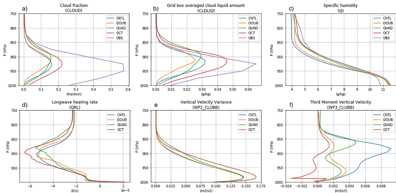
Figure 9. Same as Figure 8 but for June, July, and August and for the Californian stratocumulus area bounded by 20°N to 30°N and 230°E to 240°E.
