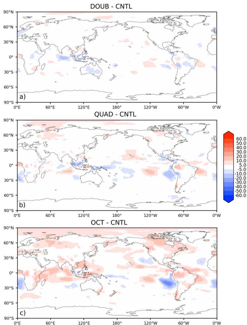
Figure 6. Same as Figure 3 but for SWCRE.
