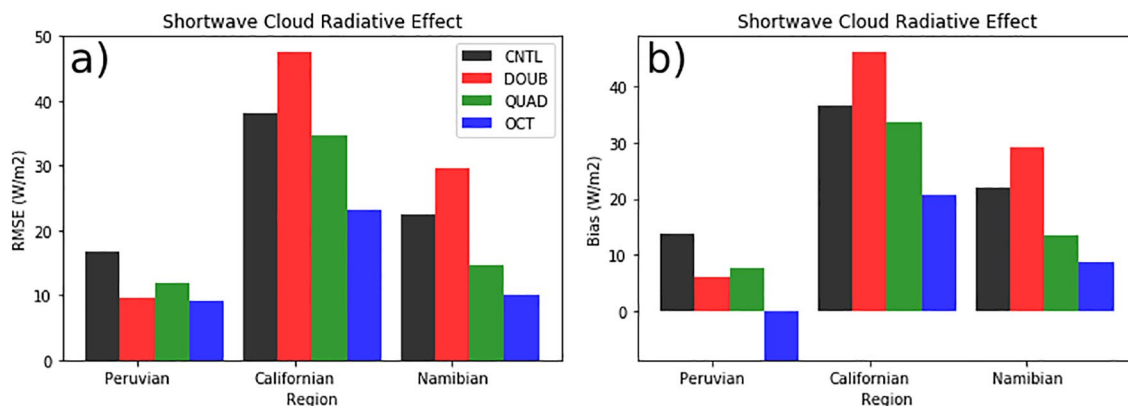
Figure 7. Same as Figure 4, but for SWCRE.
